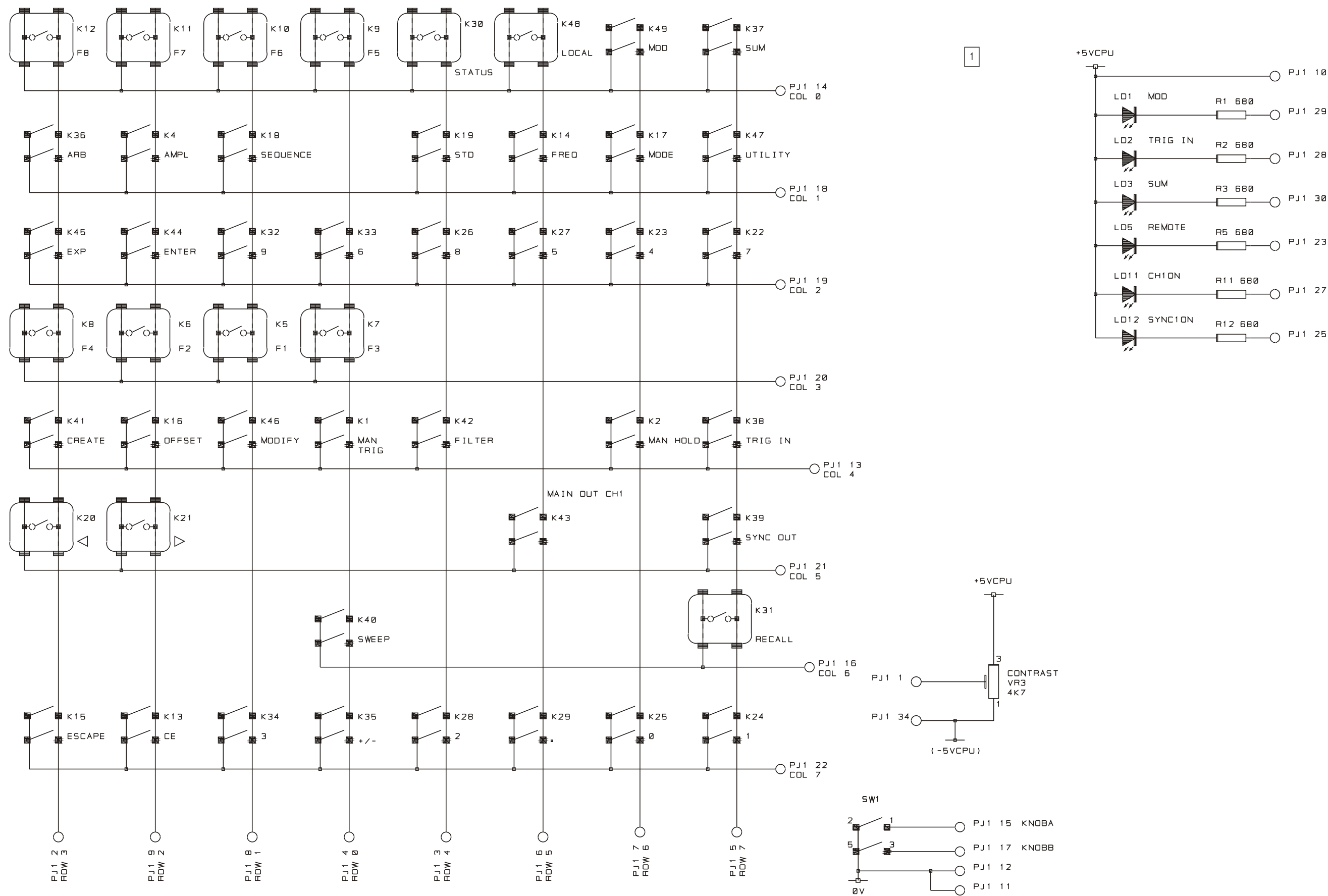
Keyboard Pcb
