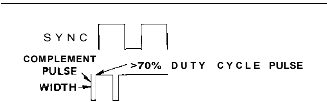
Figure 3-4. Greater Than 70% Duty Cycle Pulse
