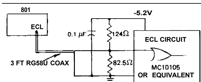
Figure 3-3. ECL Termination
