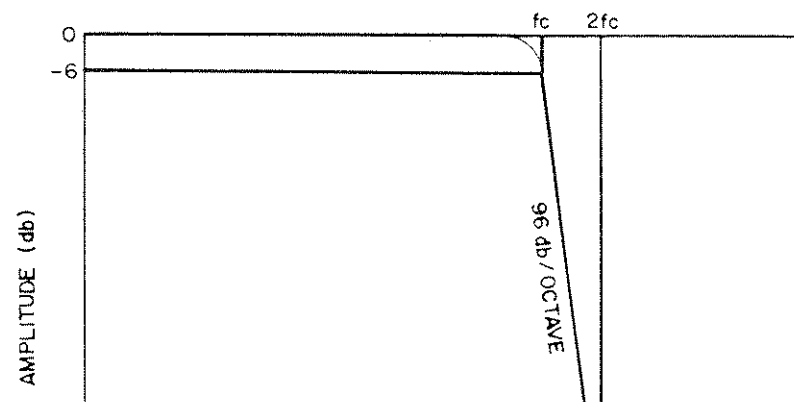
Fig. 2-11 Interconnection of Filter Channels (Model 852 Rolloff shown)
