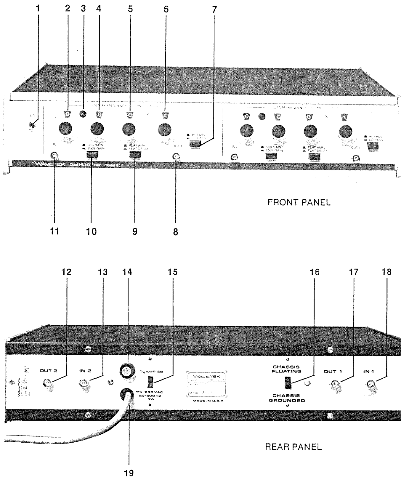
Figure 2-1. Controls and Indicators
