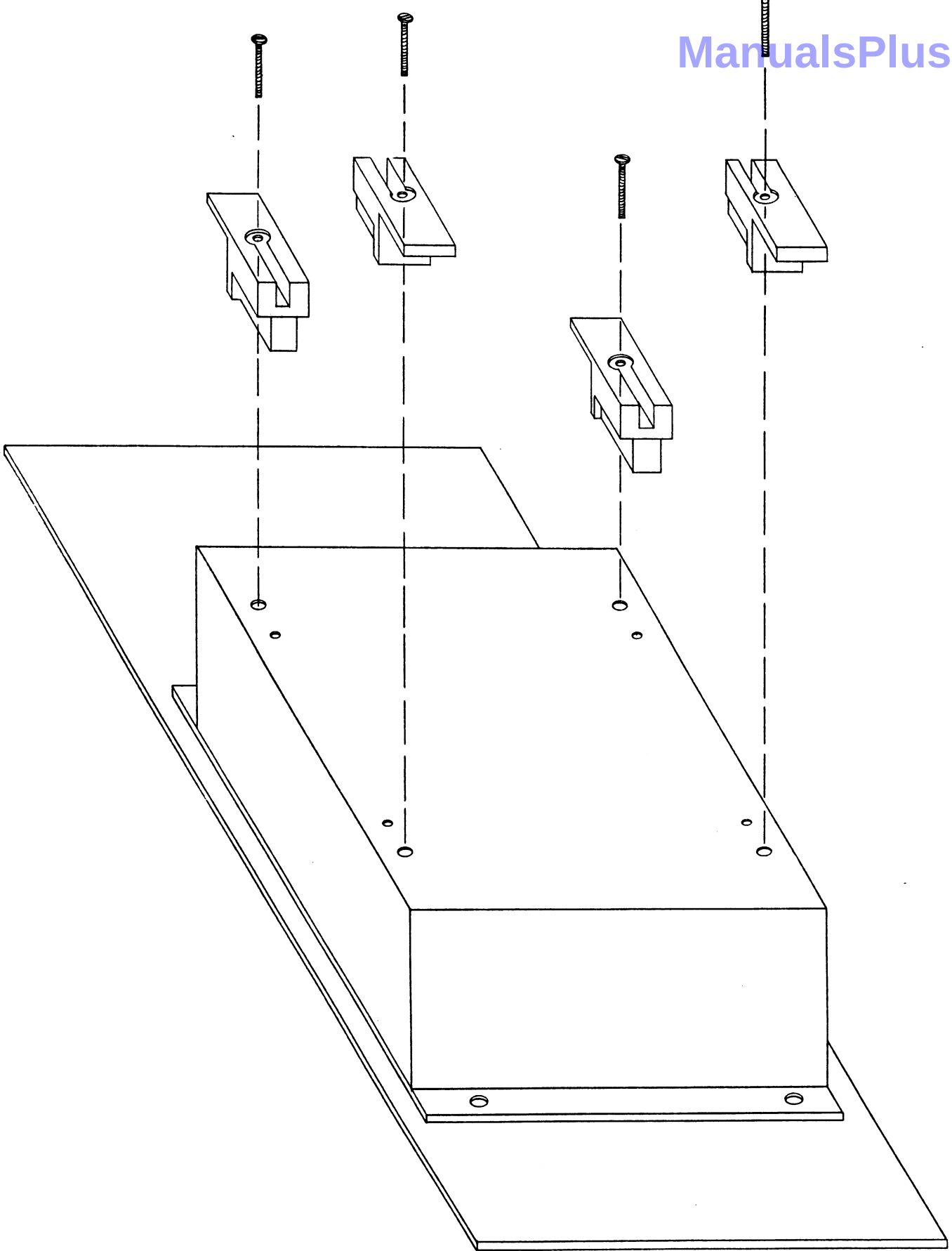
Figure 2-1. Inverter Installation
