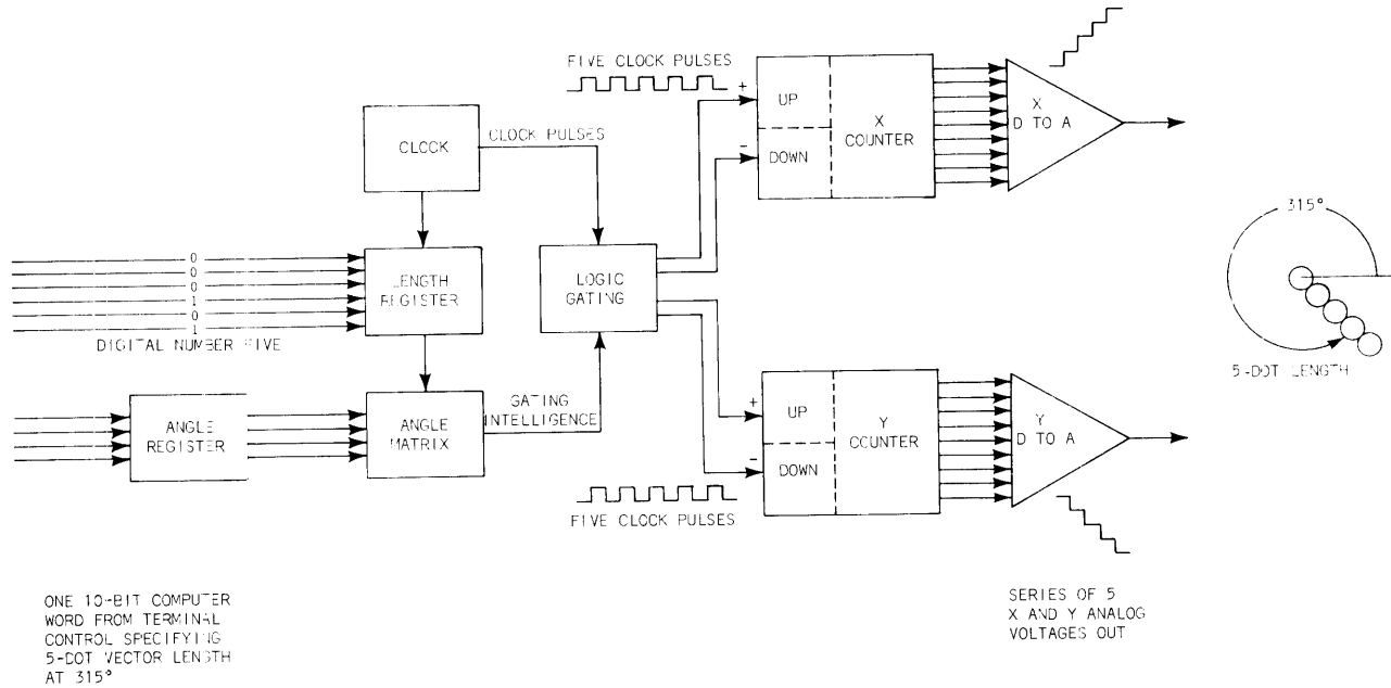
Fig. 8-5. Vector generator.
