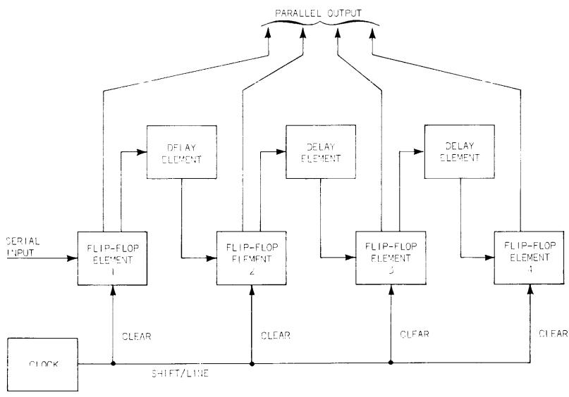
Fig. 5 6. Shift register -- serial to parallel.
