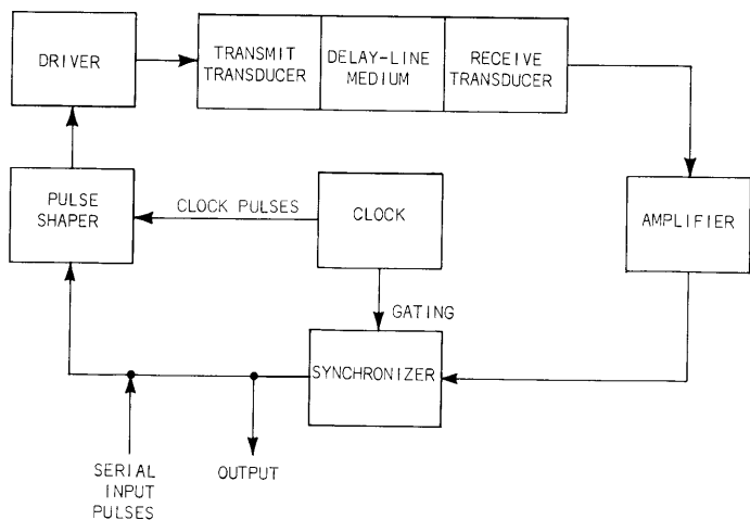
Fig. 6-5. Delay-line memory.
