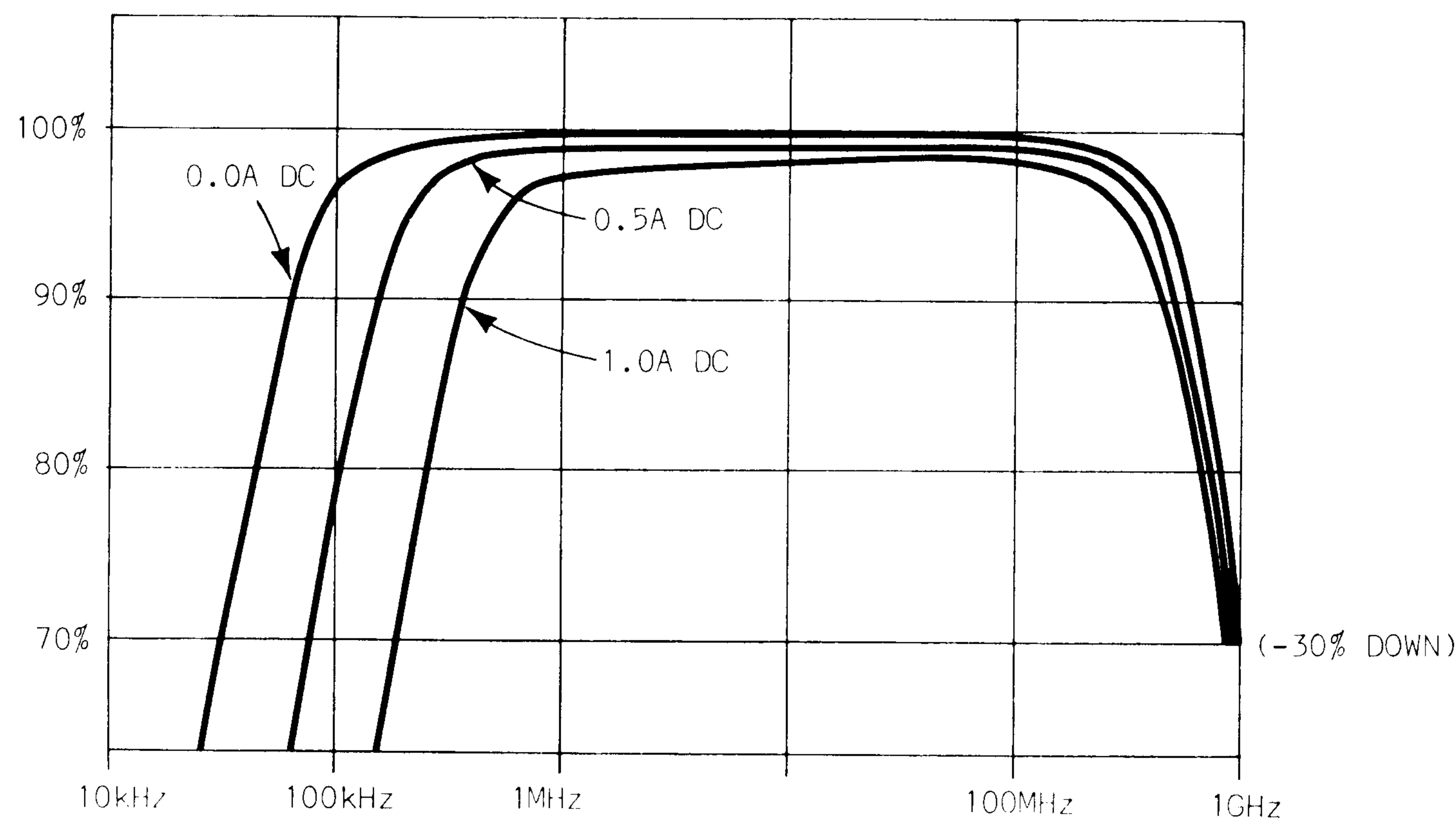
Fig. 7-8A. CT-1 bandwidth change with a DC bias current.
