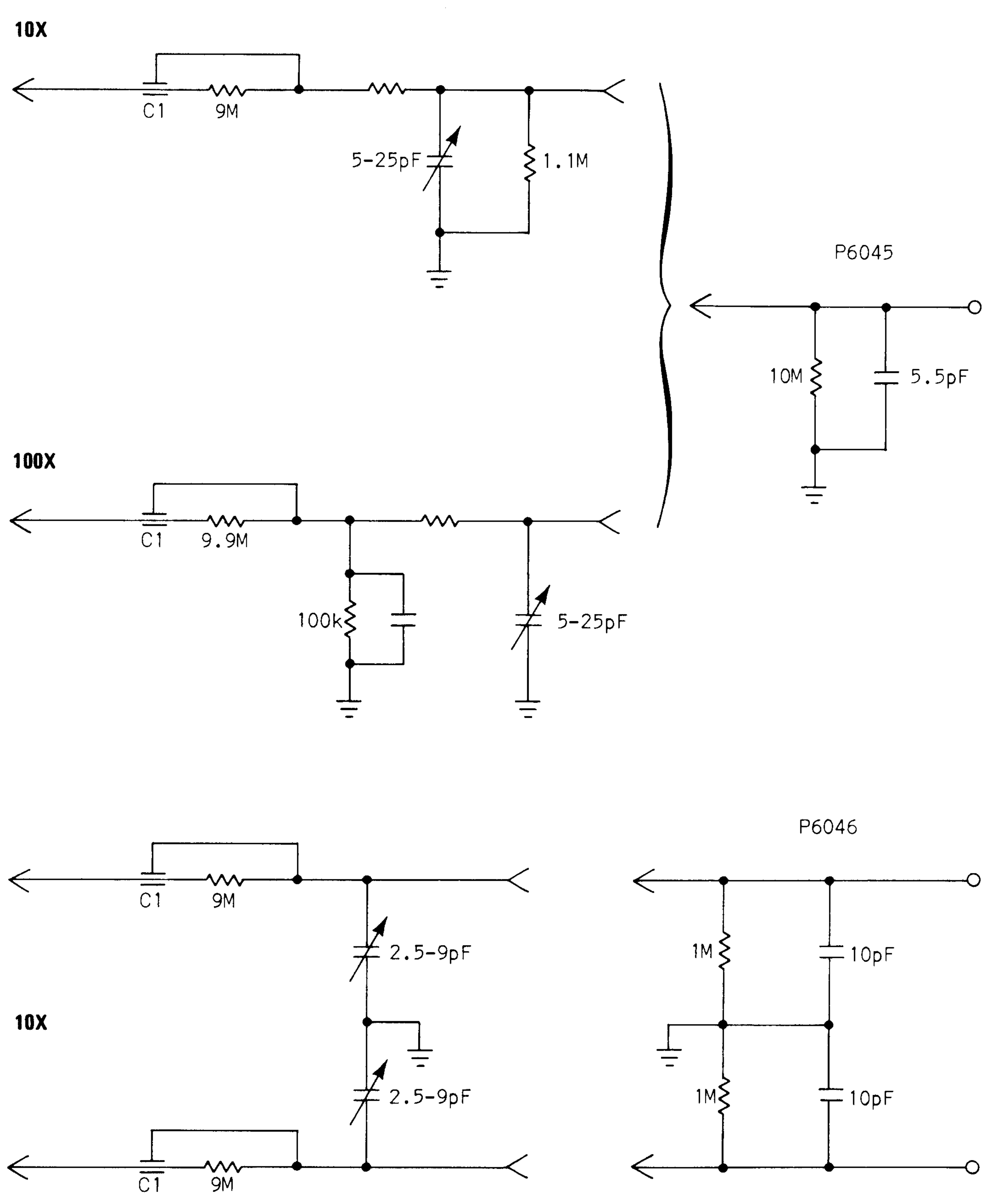
Fig. 5-2. Plug-on attenuator heads for active probes.
