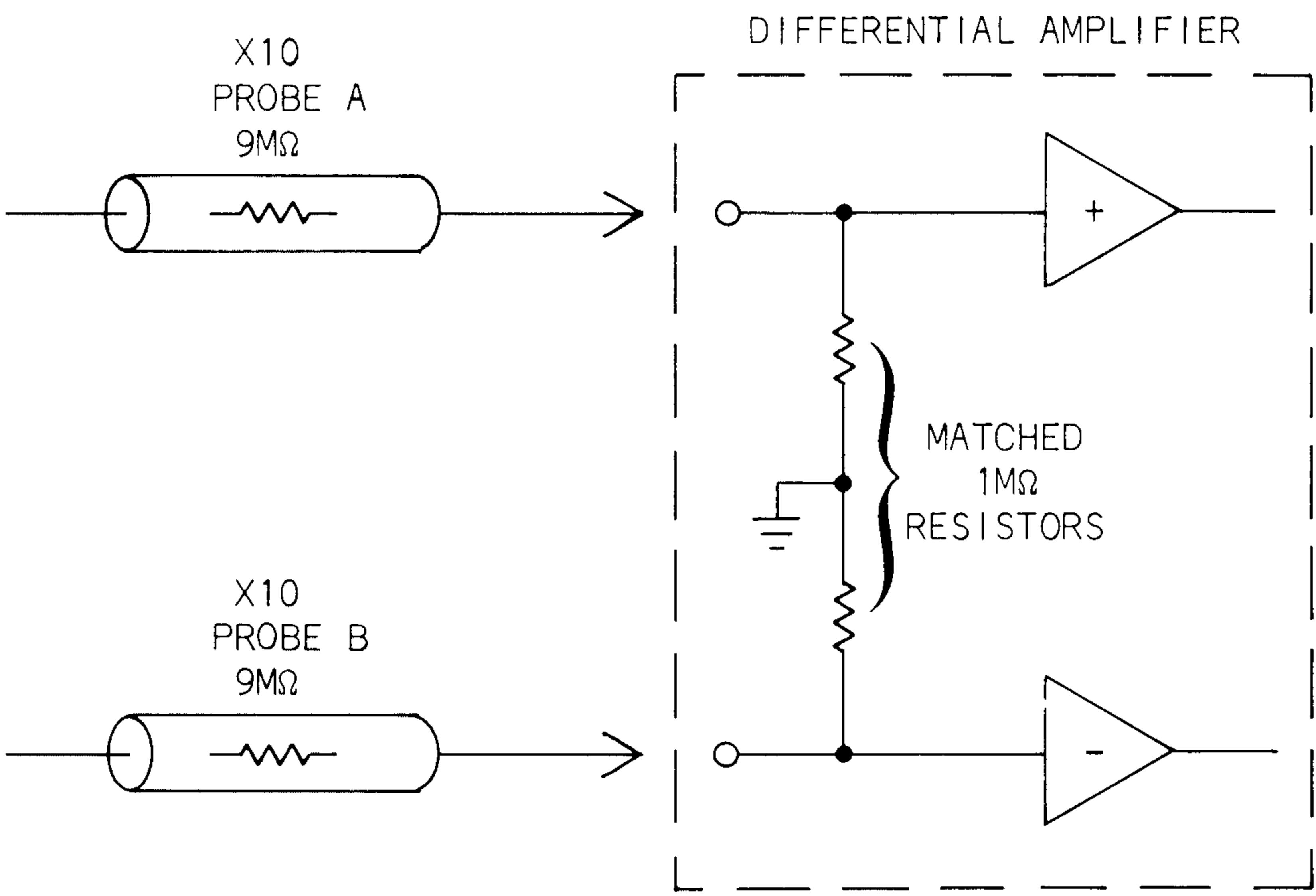
DIFFERENCES BETWEEN PROBE CAPACITANCES ADD TO THE EFFECT ON AC SIGNALS.
