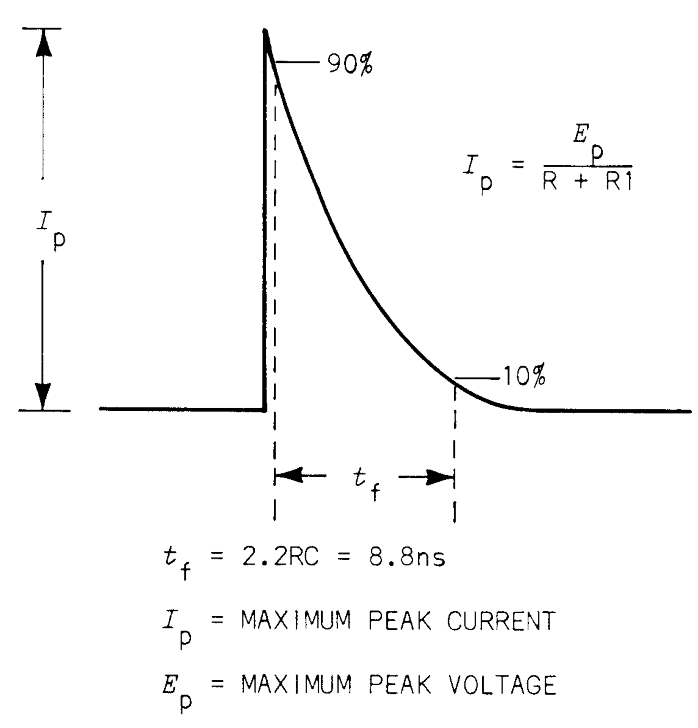
Fig. 6-2A. Ideal current waveform.
