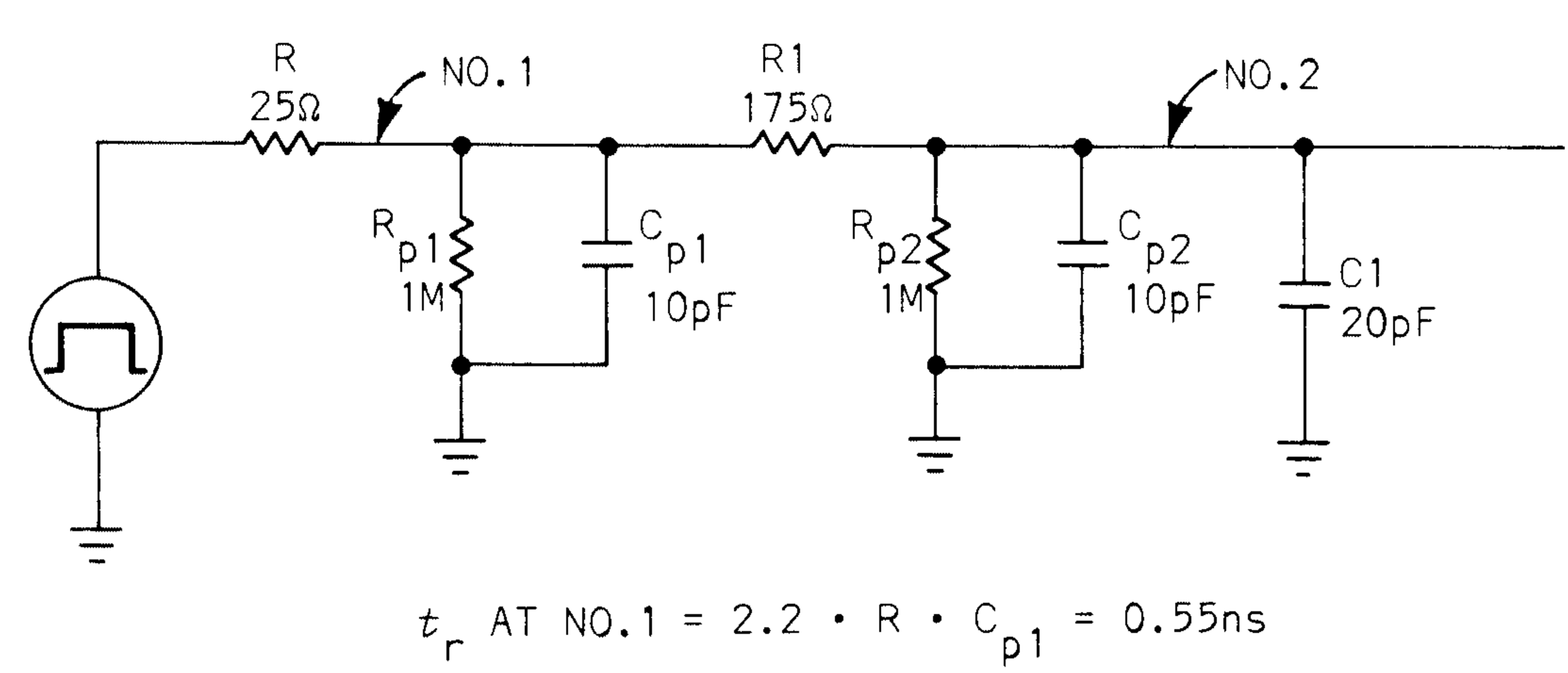
Fig. 6-2B. Typical signal source with P6046 added.
