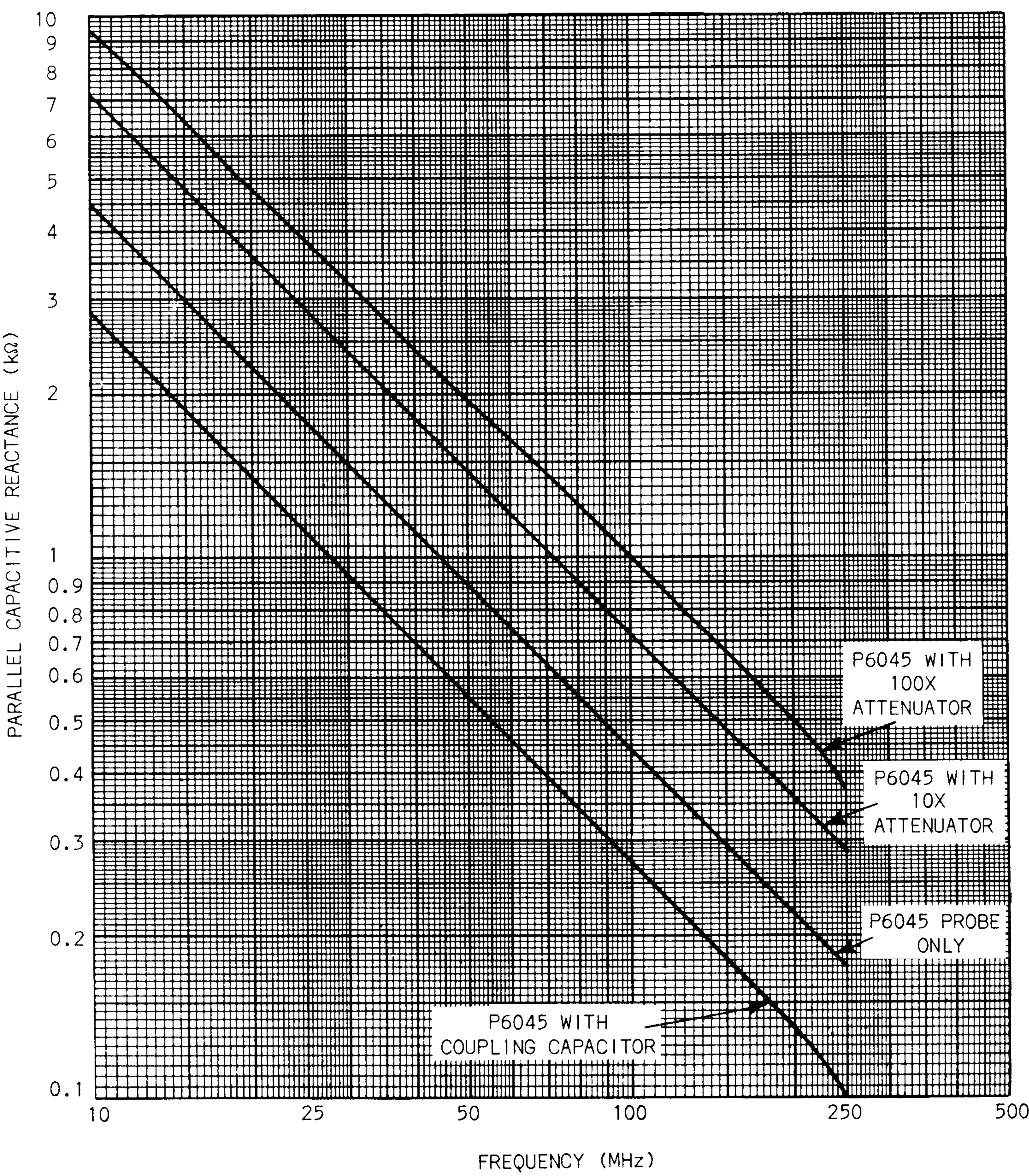
Fig. 5-6B. Typical input capacitive reactance vs frequency curves of the P6045 probe.
