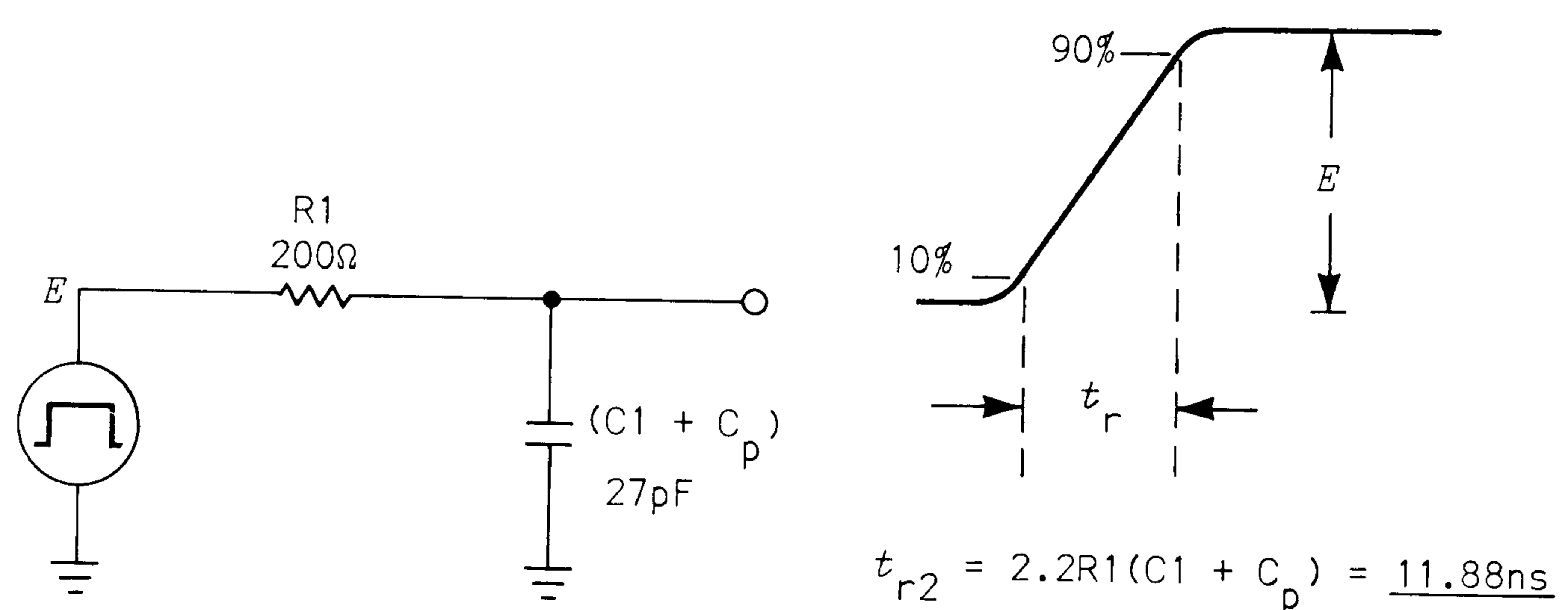
Fig. 3-3. P6006 probe added to signal source.
