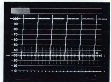
Staircase signal with variable average picture level (shown at 100). Every fourth line in successive frames carries the stairstep signal. APL variable in 11 equal steps from black to white.
