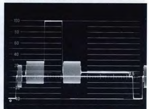
Fig 18: Display of -I, W, Q and B.
