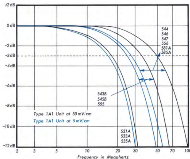
TYPICAL BANDWIDTH
