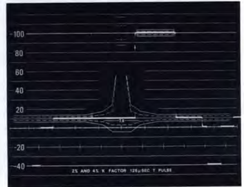
Sine 2 Pulse and Bar Signal. 0.125 \mu s HAD T-Pulse and Bar.
