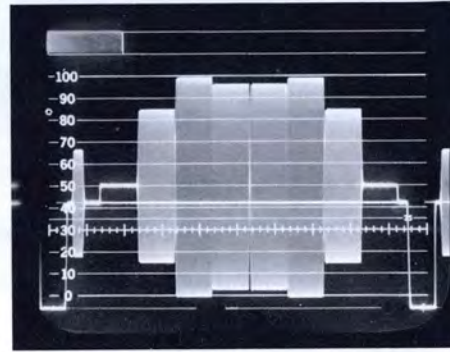
PAL colour bars, luminance component switched off.
