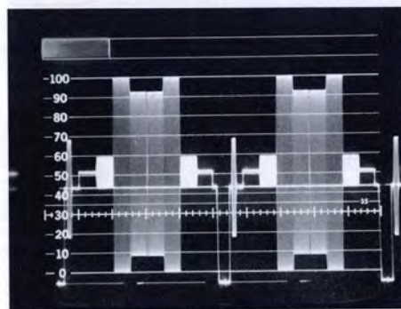
PAL colour bars, V component only; U, Y switched off.
