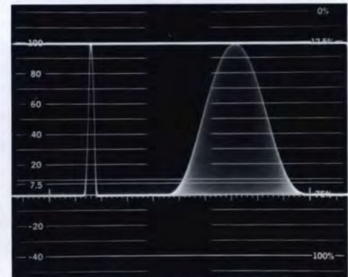
Fig 9. .250 \mu s HAD Sin 2 Pulse (left) and Modulated 20 T Sin 2 Pulse (right) with superimposed Bar Signal (top).
