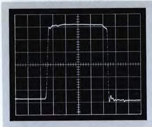
+12-volt pulse, 5 ns/cm.
