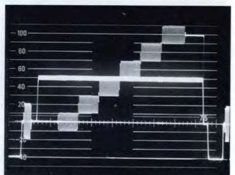
Fig 6: Modulated staircase signal with variable APL, 30 mV of subcarrier phased 90° to burst inserted on the 4 out of 5 variable lines which are at 50 IRE.
