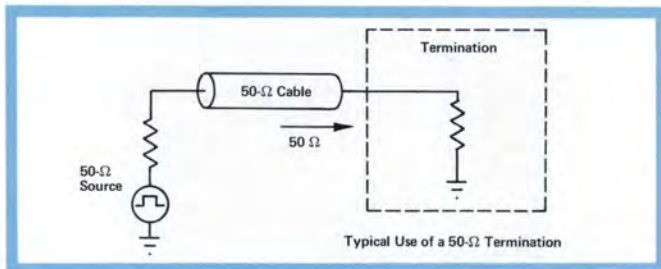
END LINE TERMINATION
