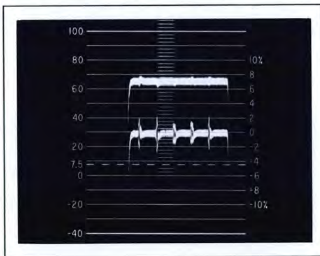
Fig 2—Differential Gain display from the Type 520 using the Type 140 NTSC Test Signal Generator. Lower trace, luminance is on. Upper trace, luminance is off. Minor divisions of graticule indicate .5% Differential Gain. Double exposure.
