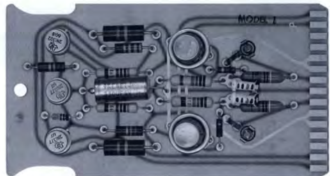
CATHODE-FOLLOWER CIRCUIT CARD ..... $32.50 Order 018-0001-00
