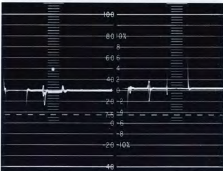
Fig 16: Double exposure (left and right) of the -I, W, Q and B bars with the I and Q depressed.
