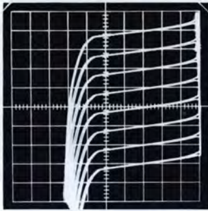
PNP TRANSISTOR
