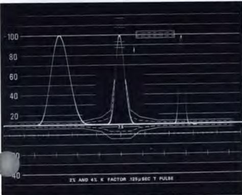
Multiple exposure. Left: 2T. Center: T. Right: 1/2 T Sine 2 , 0.25, 0.125, 0.0625 \mu s HAD.
