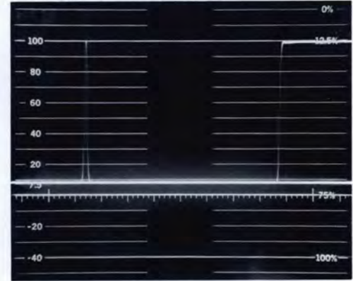
Fig 6. .125 \mu s HAD Sin 2 Pulse and Bar. 1- \mu s/div calibrated sweep, FLAT response.
