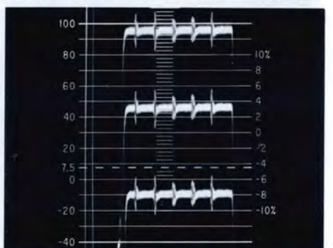
Fig 9: Triple exposure of modulated staircase viewed on a Type 520 Vectorscope in the differential gain mode. Top, 90% APL; middle, 50% APL; bottom, 10% APL.
