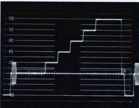
Fig 4: Modulated staircase signal, subcarrier off.
