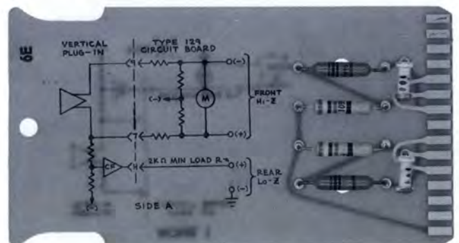
PASSIVE DIVIDER CIRCUIT CARD ..... $12 Order 018-0002-00
