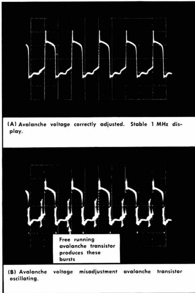
Fig. 5-17. Adjusting avalanche voltage.
