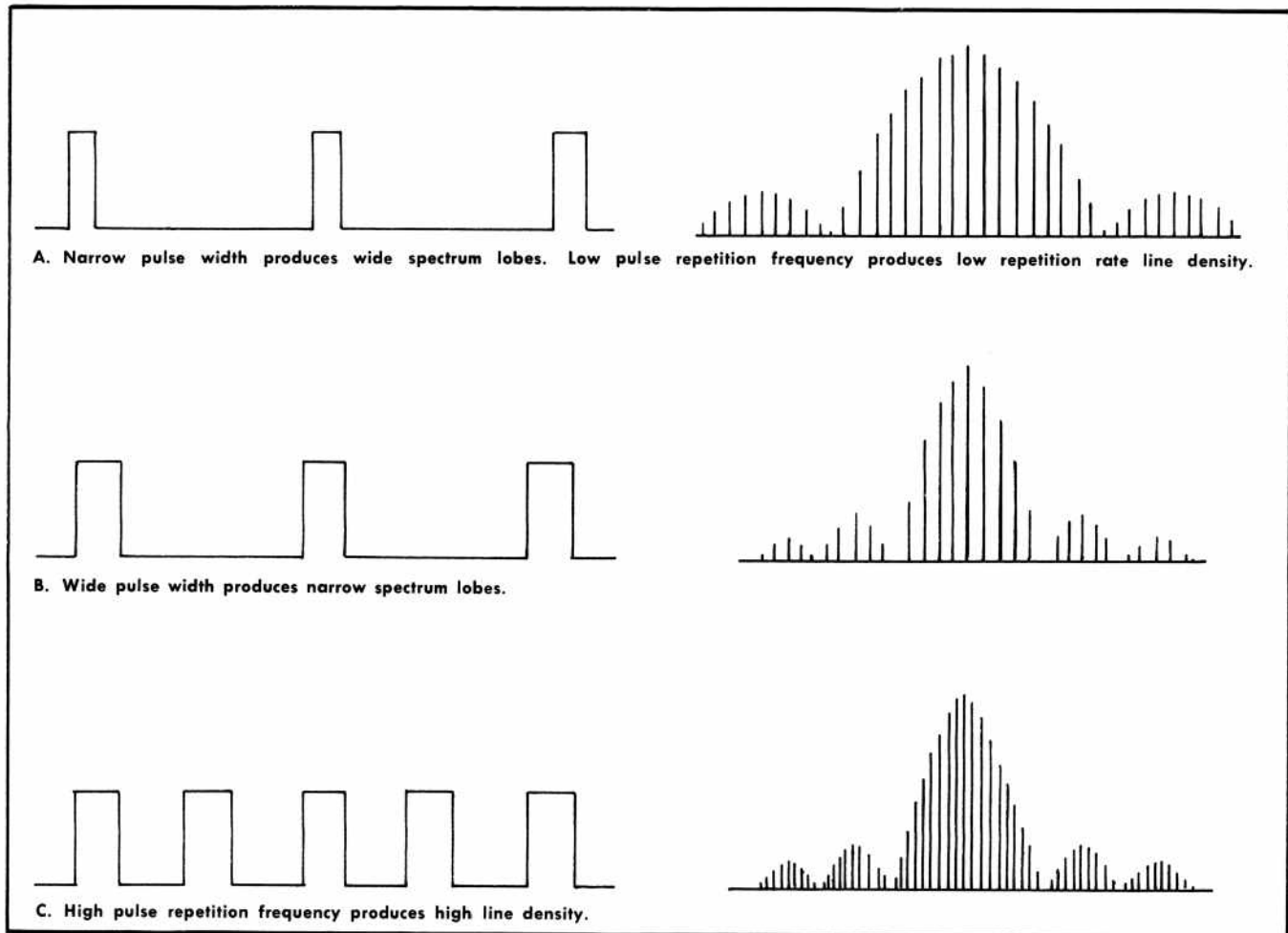
Fig. 2-17. Pulse width and PRF effects on pulse modulated spectrum.
