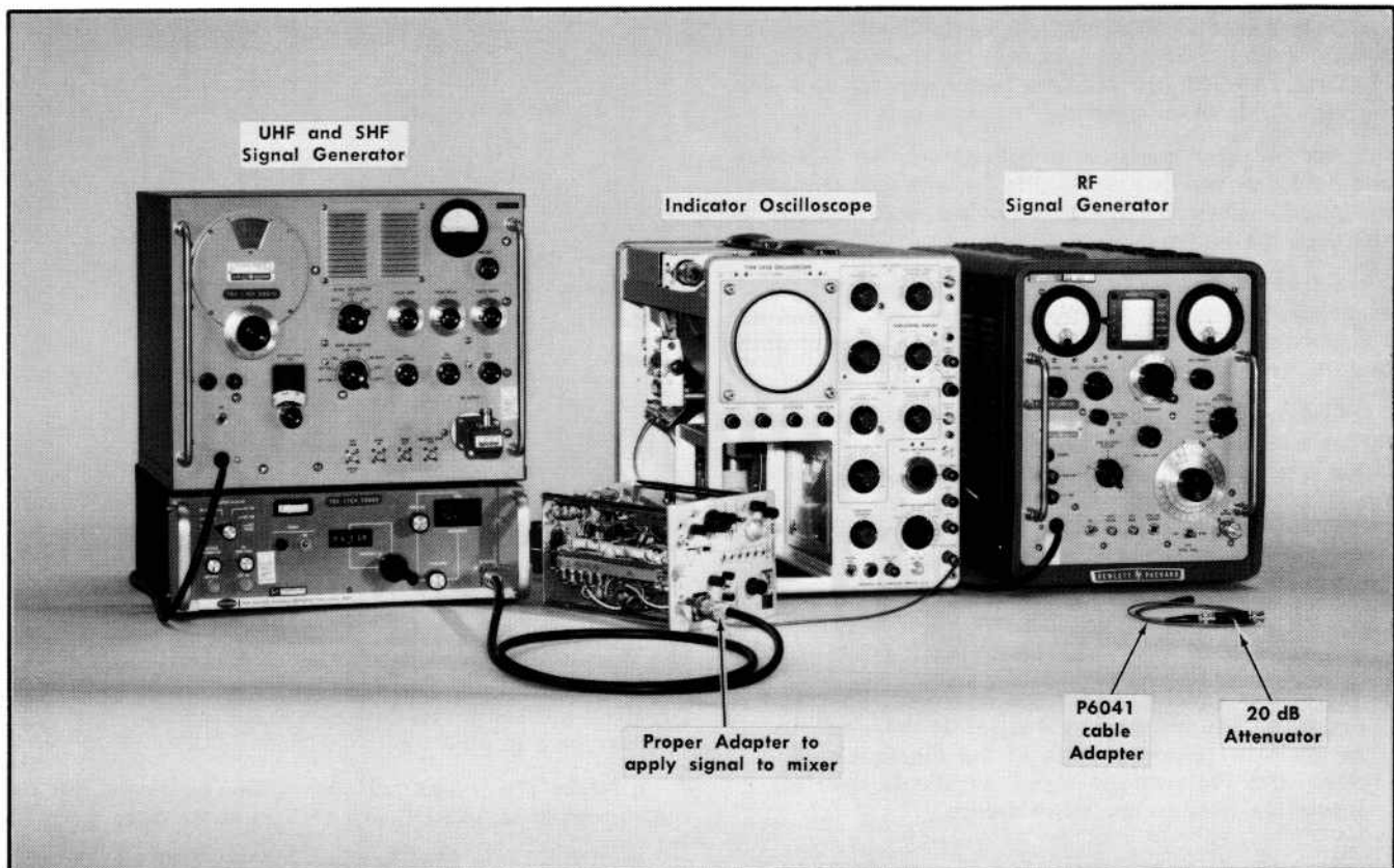
Fig. 5-22. Equipment setup to adjust the wide band IF amplifier and check RF Mixer and wide band IF amplifier response flatness (step 13).
