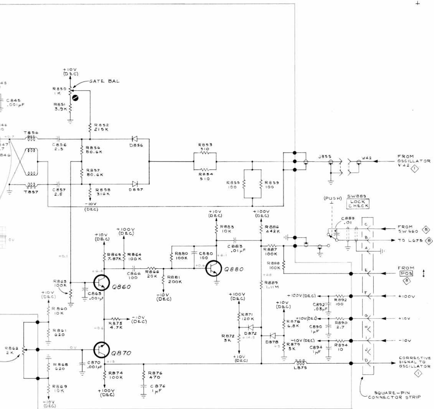
PHASE LOCK CIRCUIT 2
