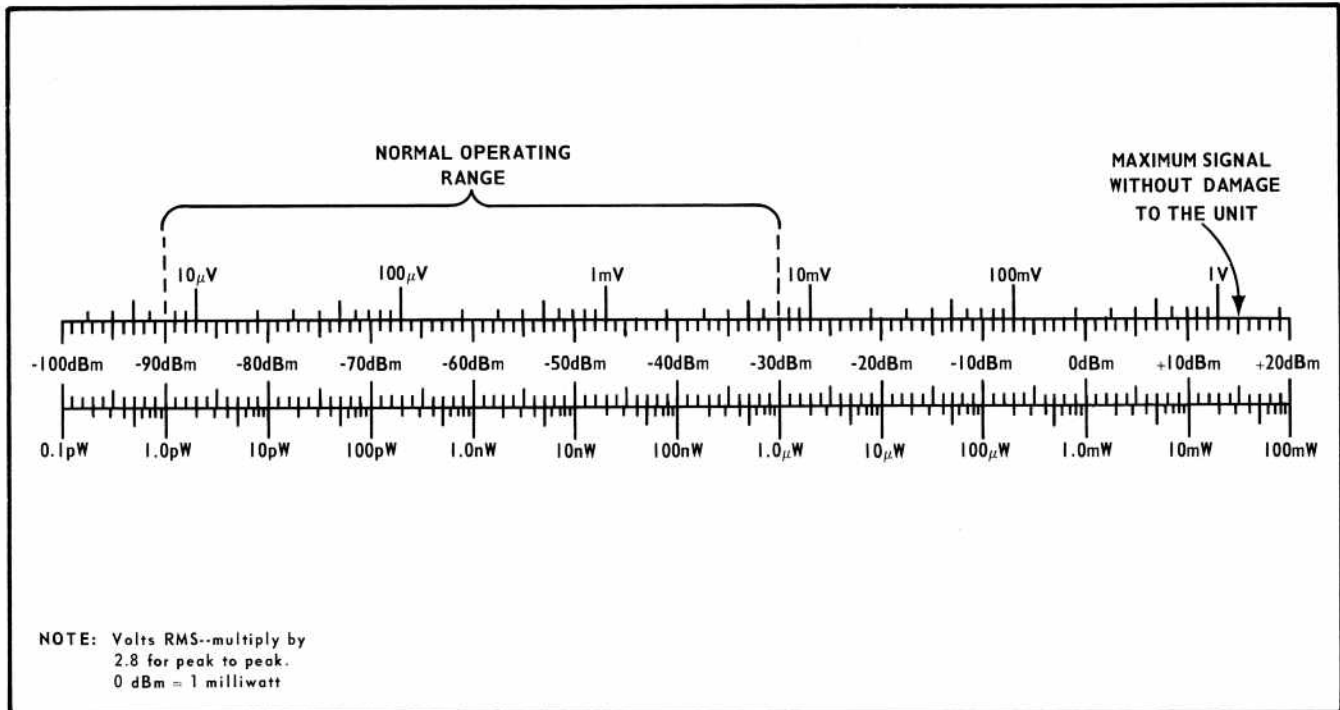
Fig. 2-5. Volts-dBm-Watts conversion chart for 50 \Omega impedance.
