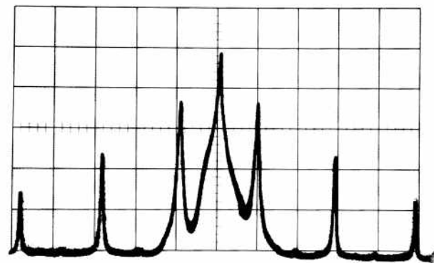
(C) Over modulated signal produces extra sidebands. LOG mode.
