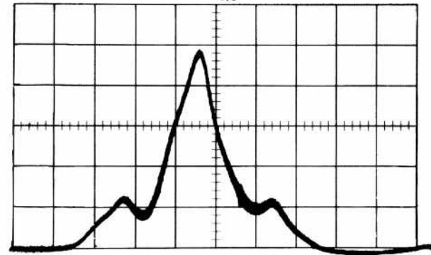
(B) Same as A but resolution bandwidth increased so that modulation is barely discernible.
