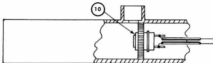
Fig. 4-4A. Tube subassembly removal procedure.
