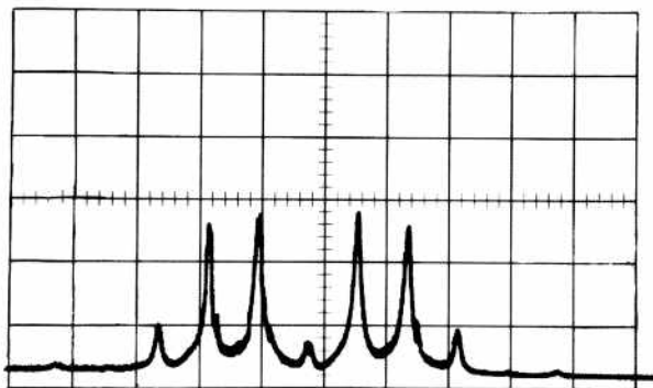
(C) Carrier almost at a null.
