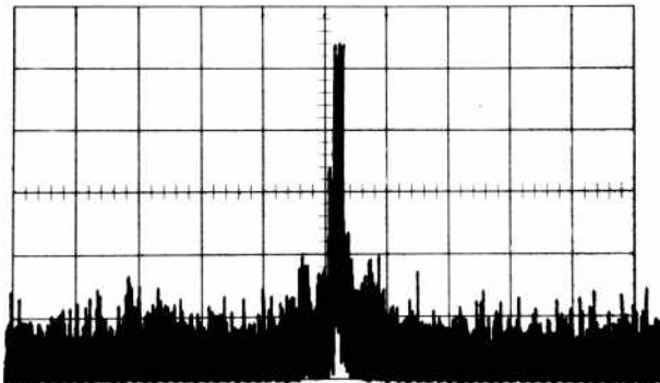
(C) Amplitude modulated signal. 2 kHz sidebands.
