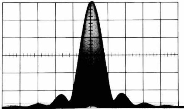
(A) \frac{\sin X}{X} spectrum of a rectangular RF pulse.
