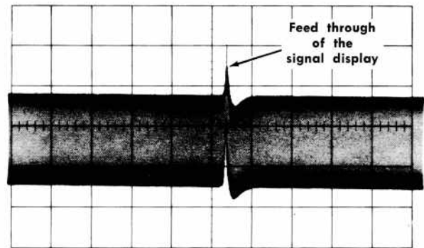
(B) LOCK CHECK button depressed while RF FINE FREQ control is adjusted. Display DC level will shift as control is adjusted. Select a beat mode near the screen center for best operation.
