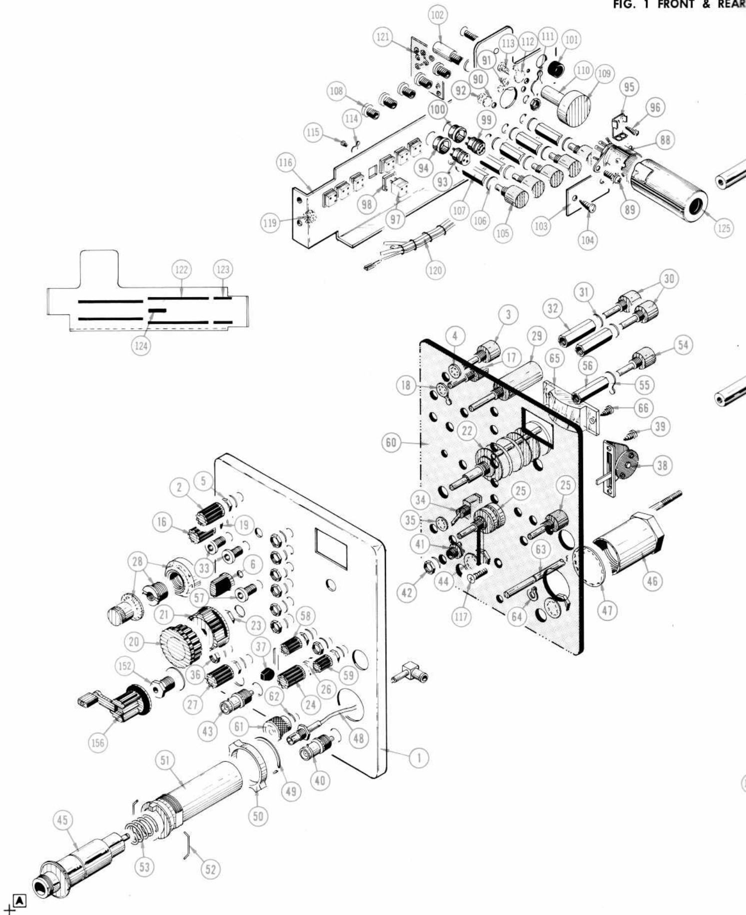
FIG. 1 FRONT & REAR
