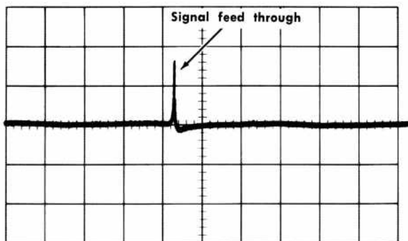
(C) Null point. Oscillator will now lock in phase with the reference frequency. Release LOCK CHECK button.
