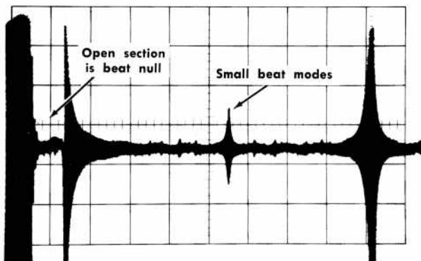
(A) Large and small beat signal displays. LOCK CHECK button is depressed while the RF CENTER FREQUENCY control is slowly tuned.
