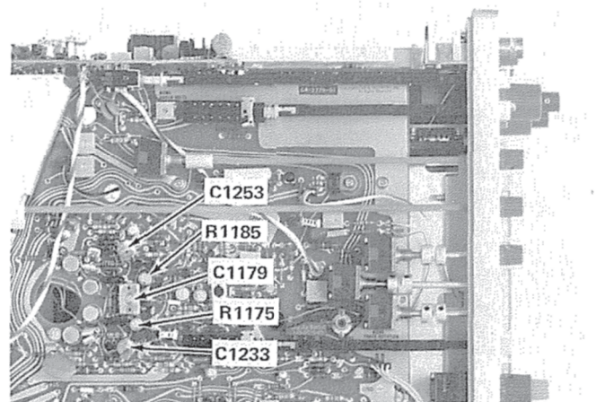
Fig. 5-27. Location of high-speed timing adjustments (except R1075).
