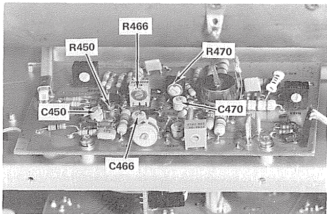
Fig. 5-16. Location of vertical output high-frequency adjustments.
