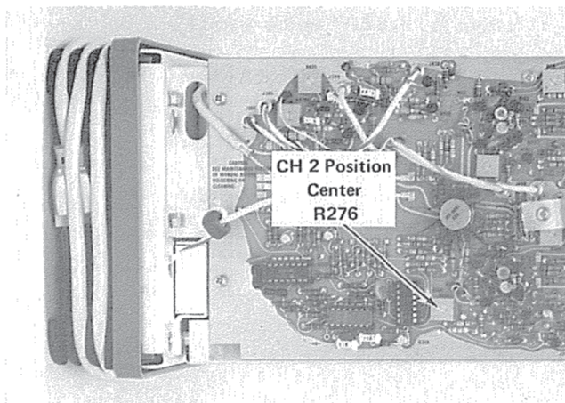
Fig. 5-11. Location of CH 2 Position Centering adjustment.
