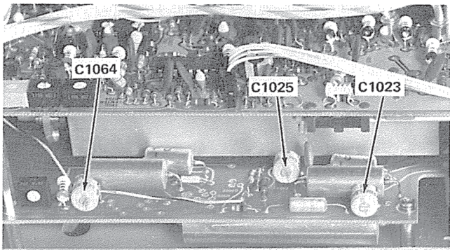
http://www.ccskill.com Fig. 5-25. Location of A and B Sweep timing adjustments.
