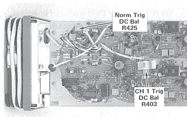
Fig. 5-21. Location of Normal Trigger DC Balance and CH 1 Trigger DC Balance adjustments.
