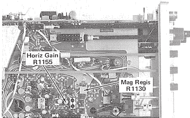
Fig. 5-24. Location of Horizontal Gain and Magnifier Registration adjustments.
