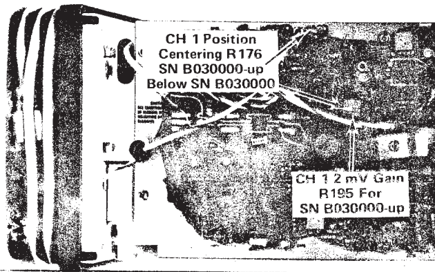
Fig. 5-9. Locations of CH 1 position centering adjustment R176 and CH 1 2 mV Gain R195 (SN B030000-up).
