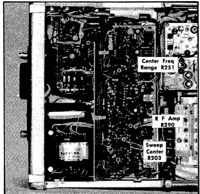
Fig. 6-18. Sweeper circuit adjustments.
