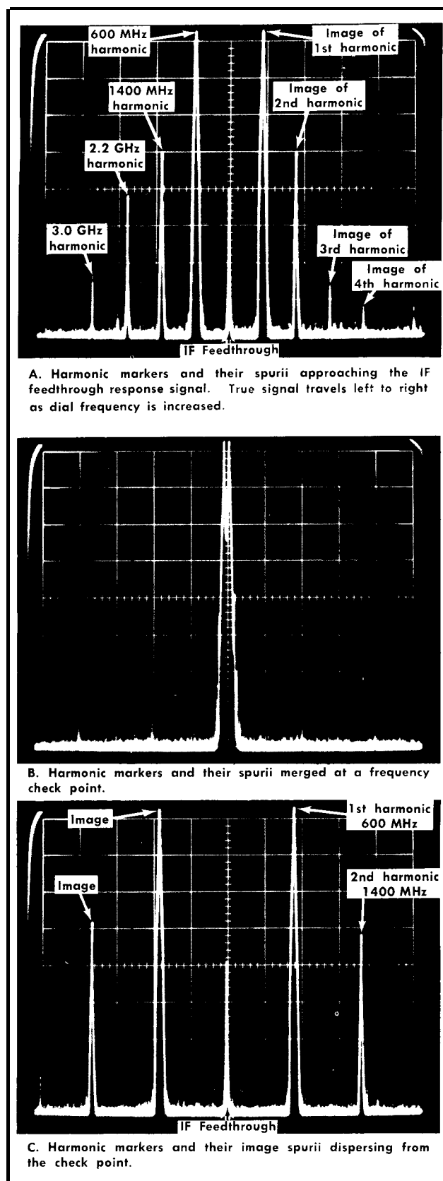
Fig. 5-8. Harmonic frequency markers used to check dial accuracy.
