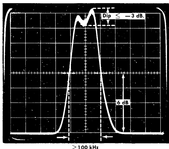
A. Resolution at -6 dB point \geq 100 kHz. Dispersion 50 kHz/div.
