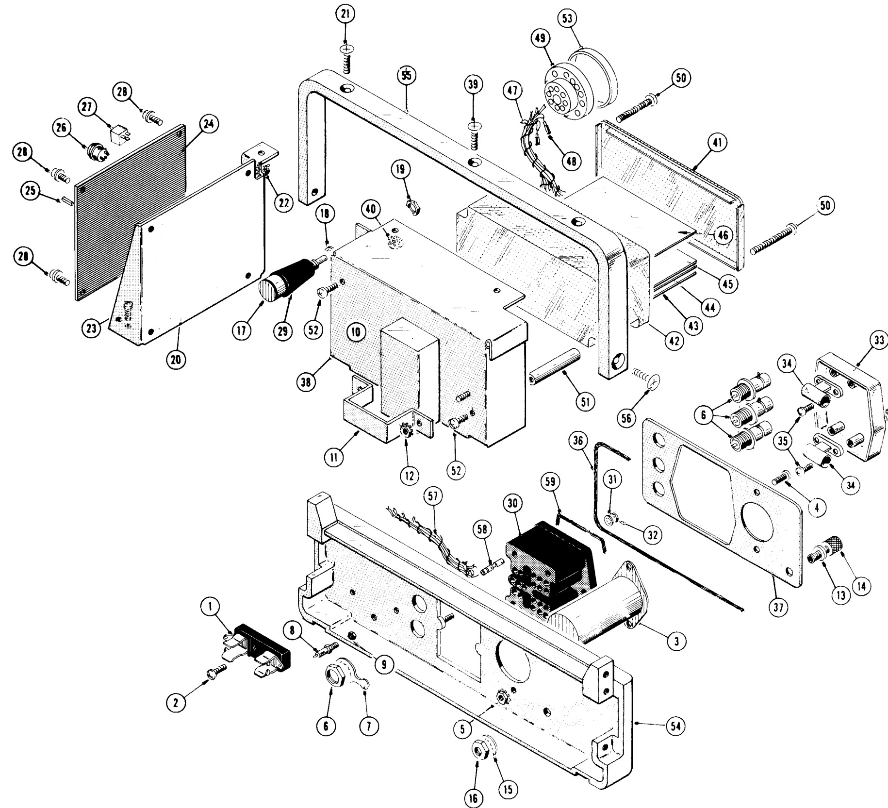
FIG. 2 REAR
