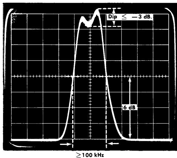
A. Resolution at -6 dB point \geq 100 kHz. Dispersion 50 kHz/div.
