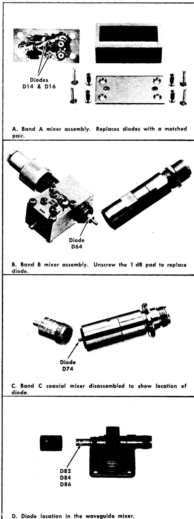
Fig. 4-18. Replacing the mixer diodes.
