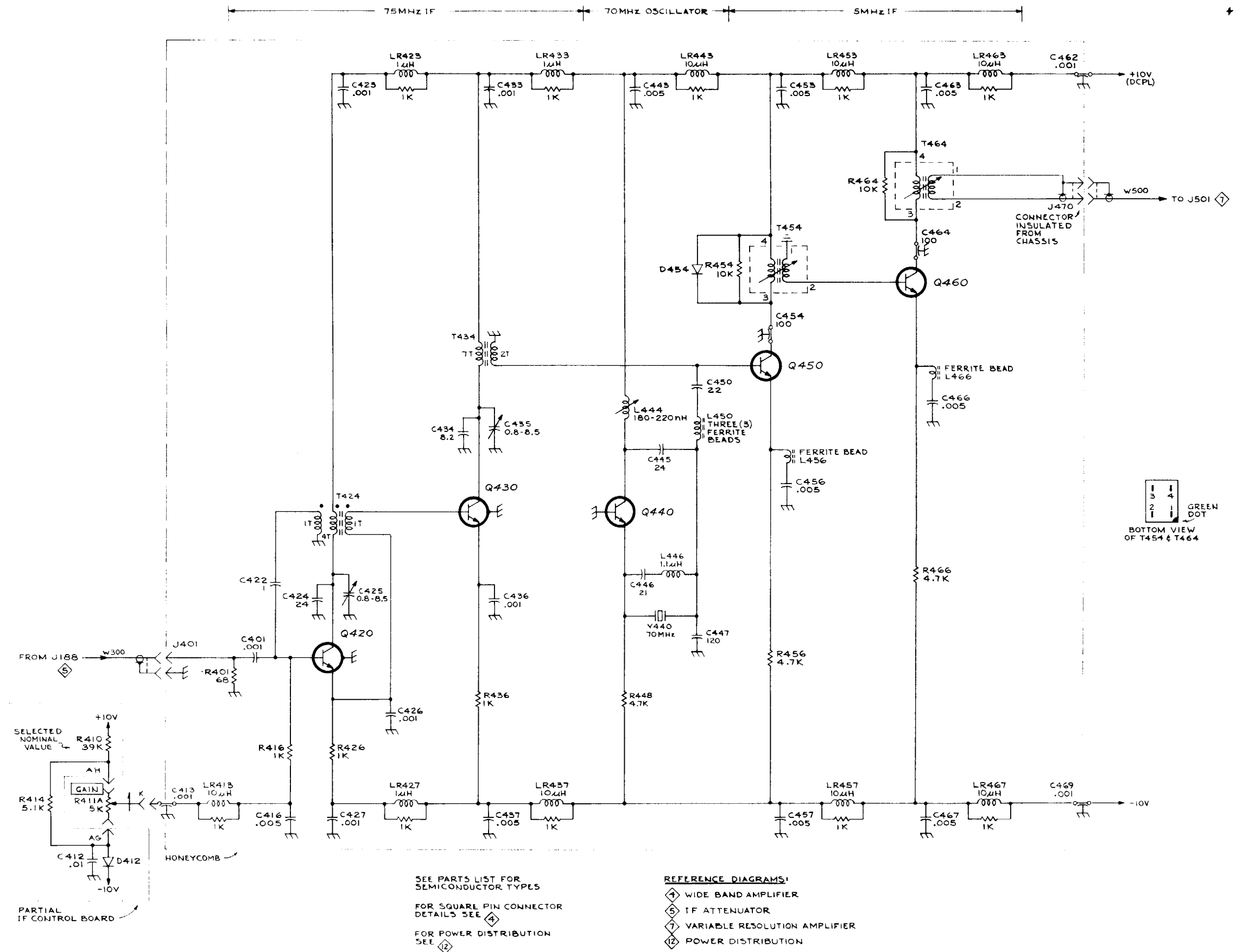
NARROW BAND AMPLIFIER (6) 1166
