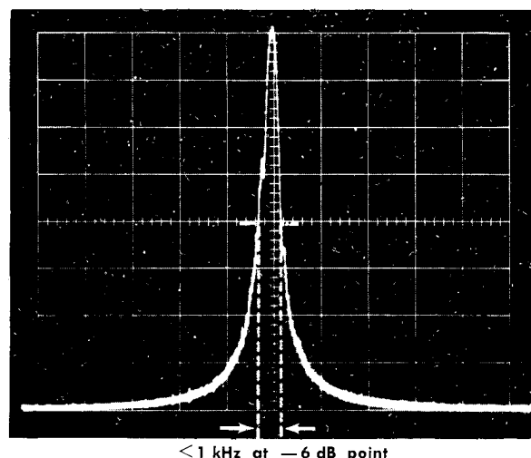
B. 1 kHz/div resolution.
