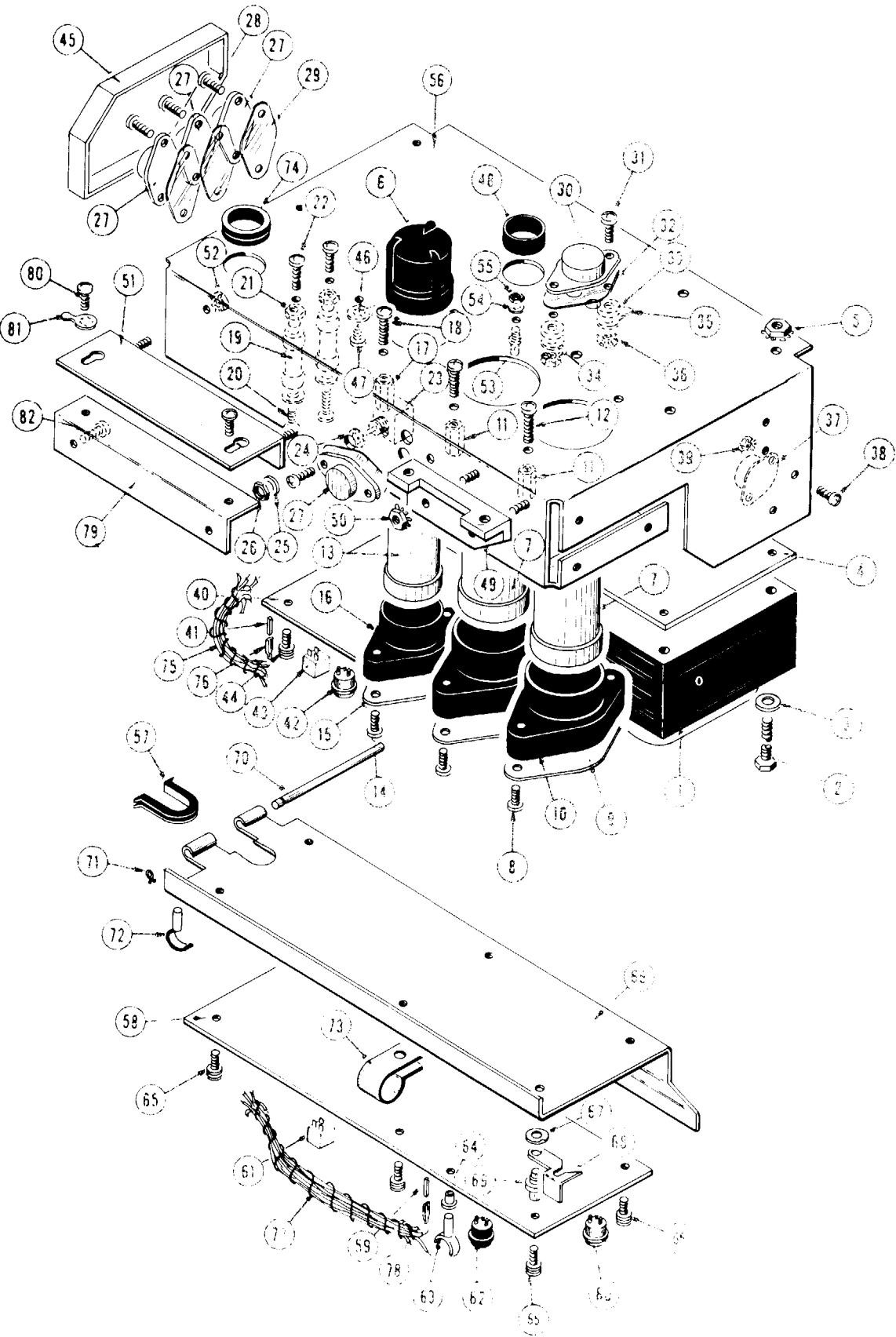
FIG. 4 POWER CHASSIS
