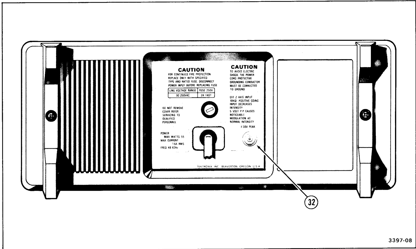
Figure 2-7. Rear-panel connector.
