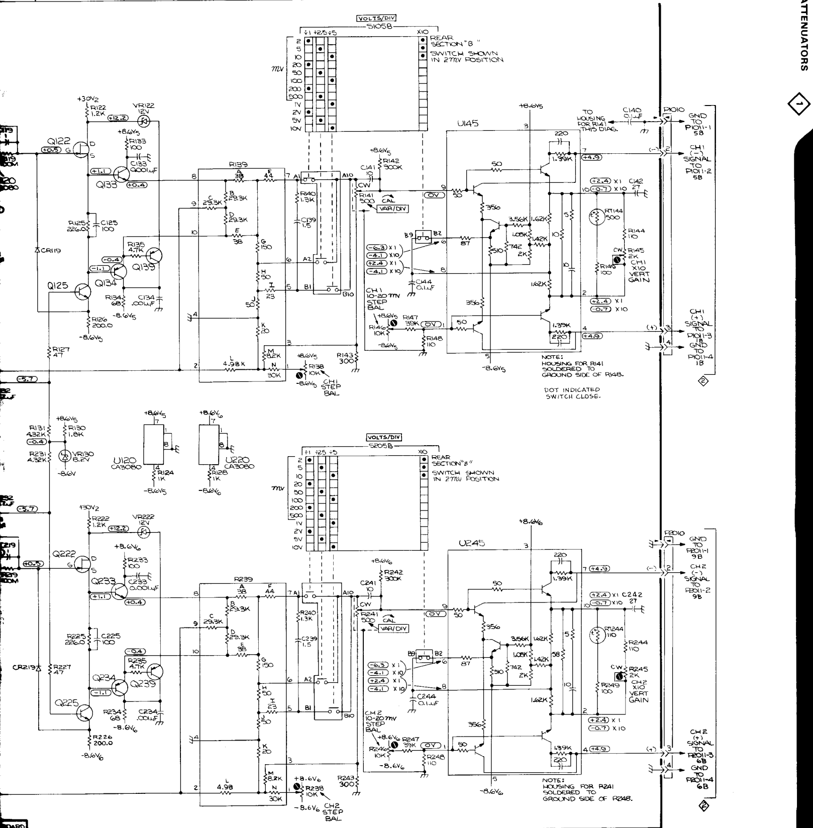
CH1 & CH2 ATTENUATORS
