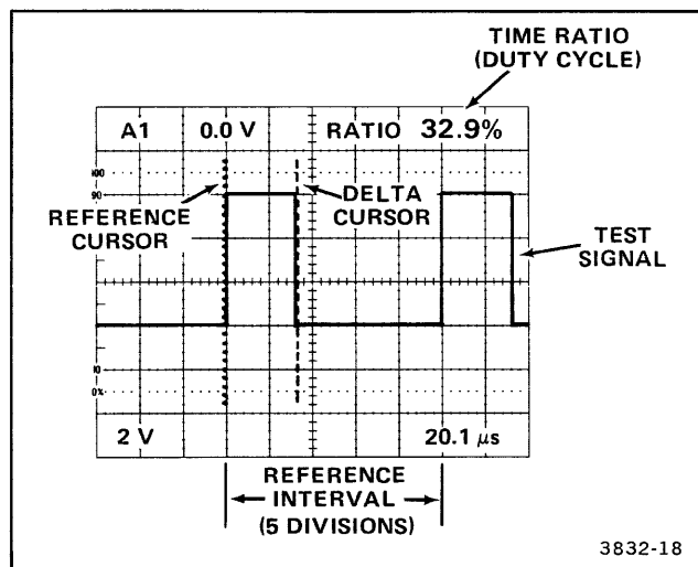
Figure 6-6. Time ratios (duty cycles).
