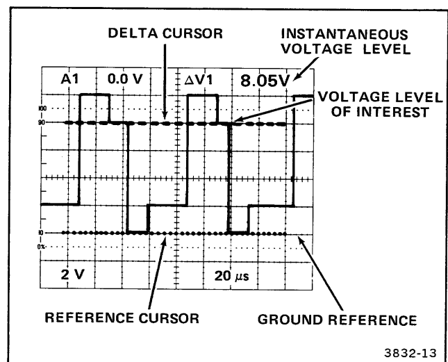
Figure 6-1. Instantaneous dc levels.
