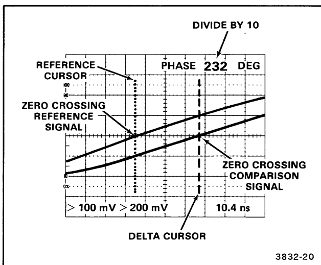
Figure 6-8. Small-angle phase difference.
