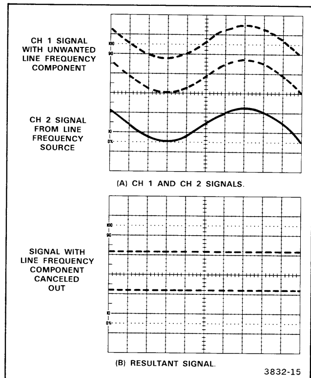
Figure 6-3. Eliminating common-mode signals.
