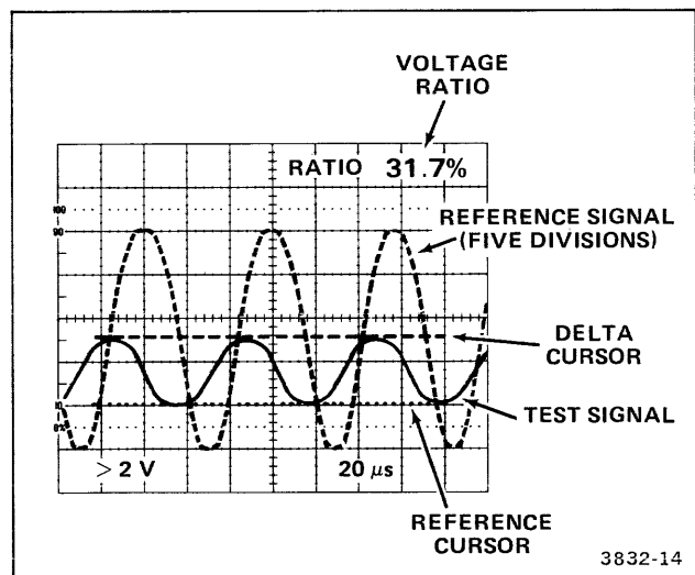
Figure 6-2. Voltage ratios.
