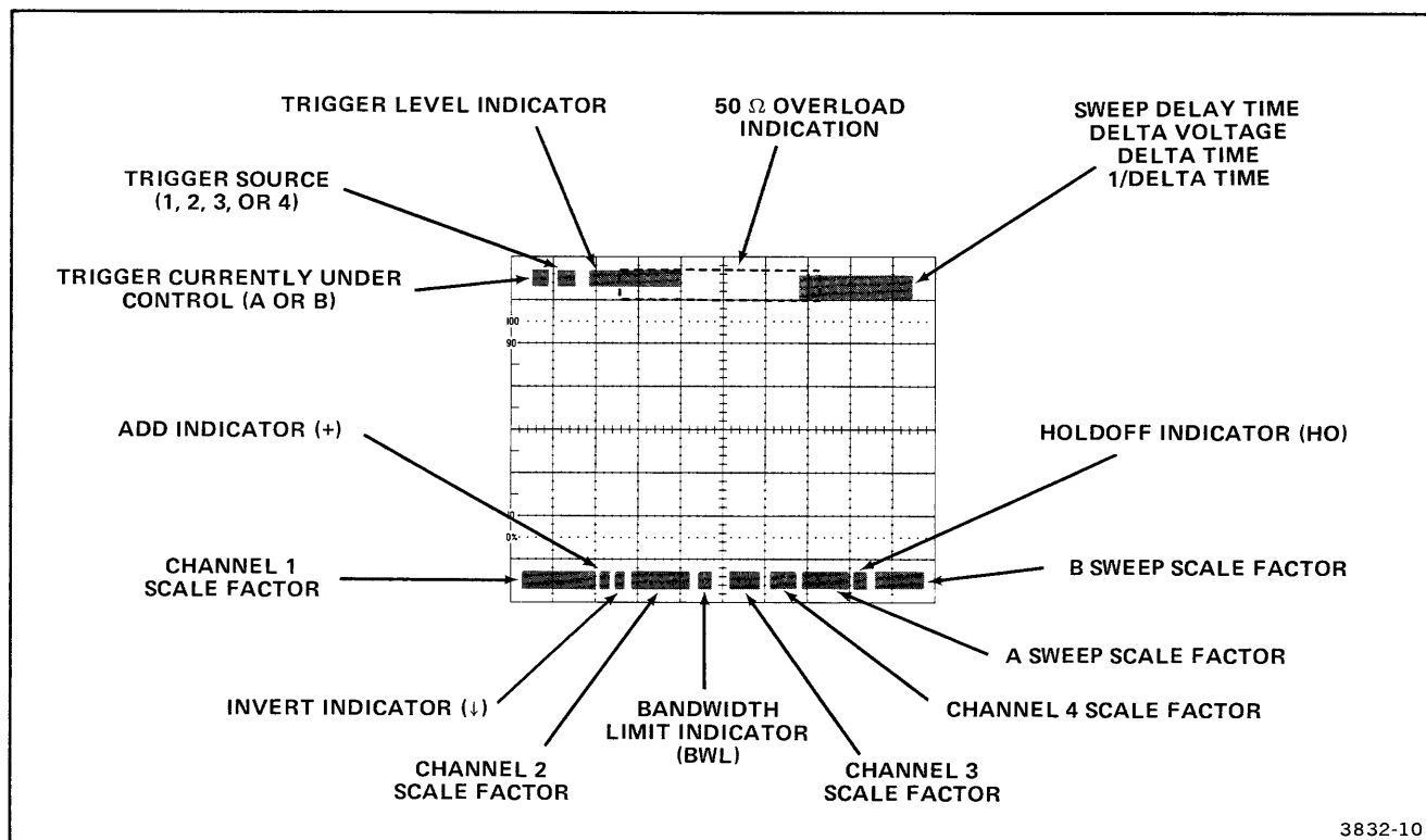
Figure 3-7. Readout display locations.
