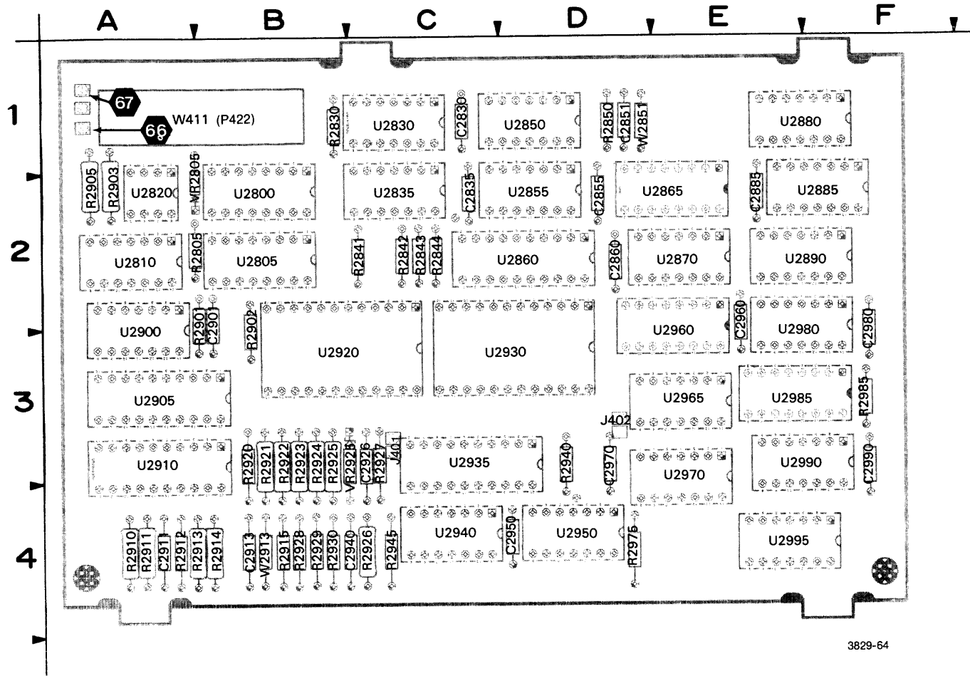
Figure 9-10. A4—Readout board.
