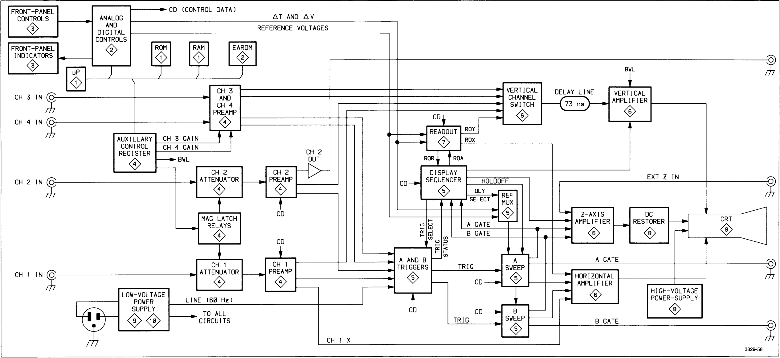
Figure 9-4. 2445 block diagram.
