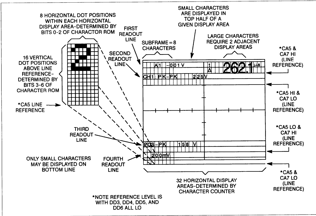
Figure 3-5. Developing the readout display.
