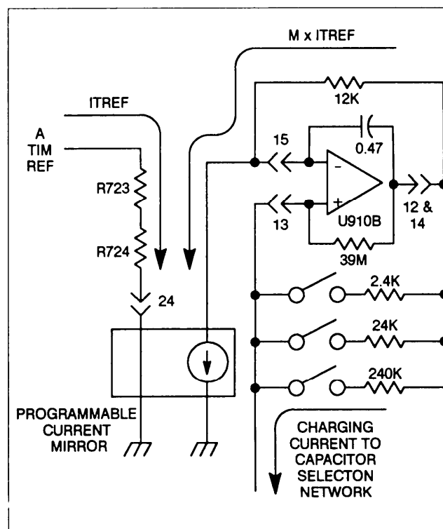
Figure 3-4. Sweep generator.
