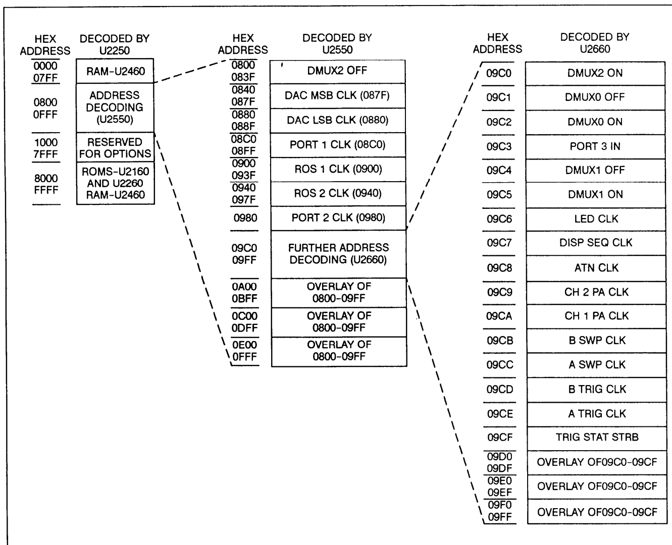
Figure 3-1. Address decoding.
