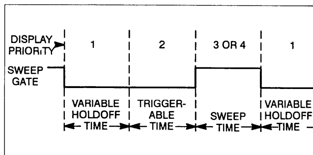
Figure 3-6. Readout display priorities.
