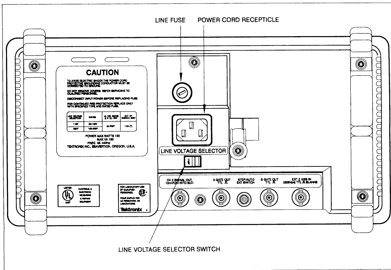
Figure 2-1. Line voltage selector switch, line fuse, and power cord receptacle.
