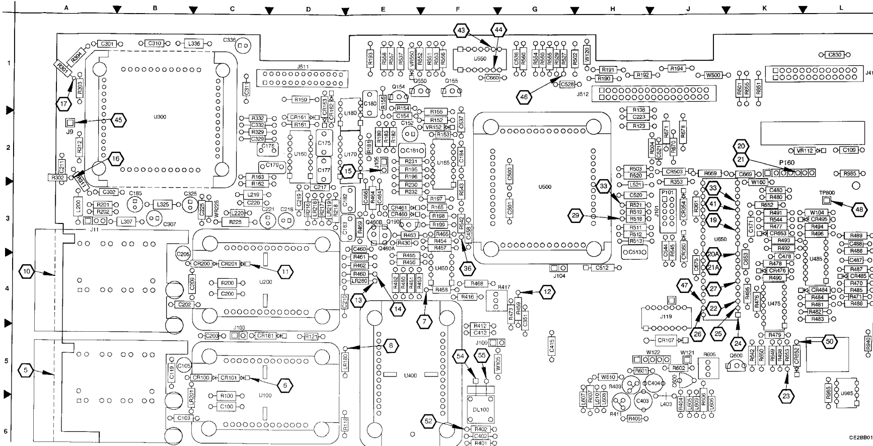
Figure FO-7. A1 Main Board Component Locator (Sheet 1 of 2) FP-19/(FP-20 blank)
