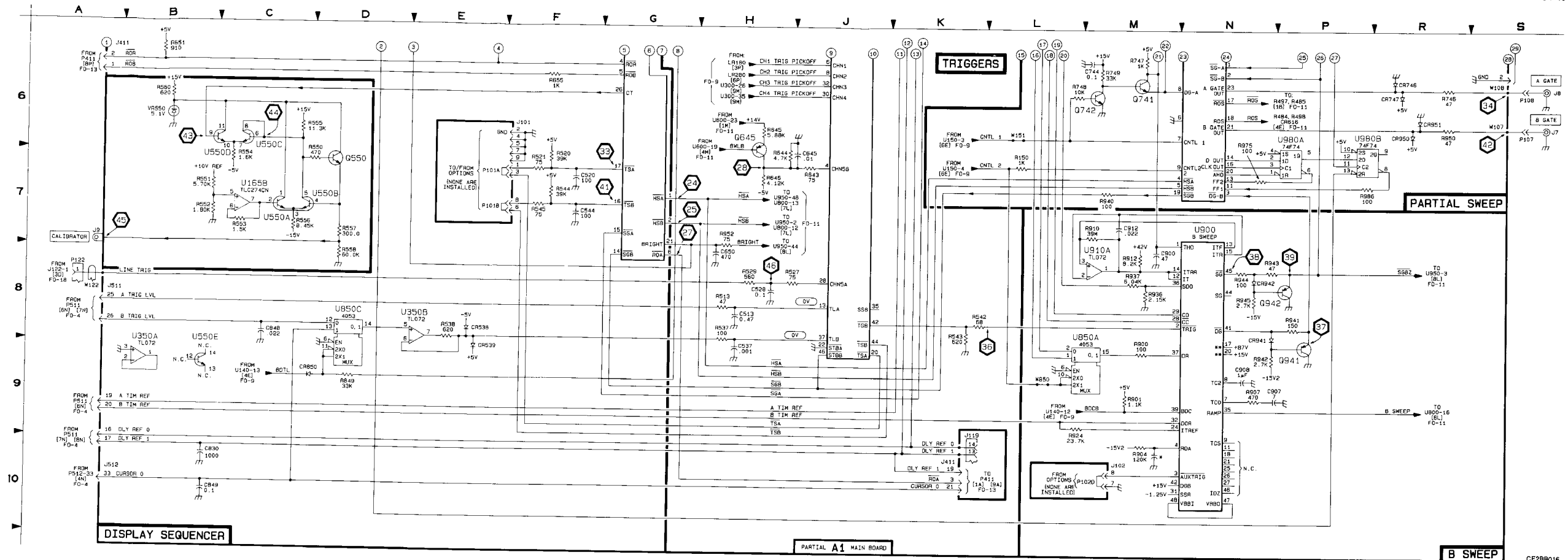
Figure FO-10. Holdoff, Display Sequencer, Triggering and Sweeps Schematic (Sheet 2 of 3). FP-31/(FP-32 blank)
