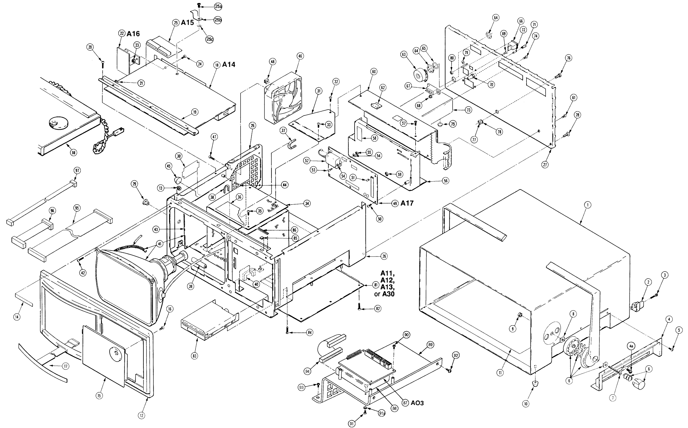
Figure 2. Exploded View
