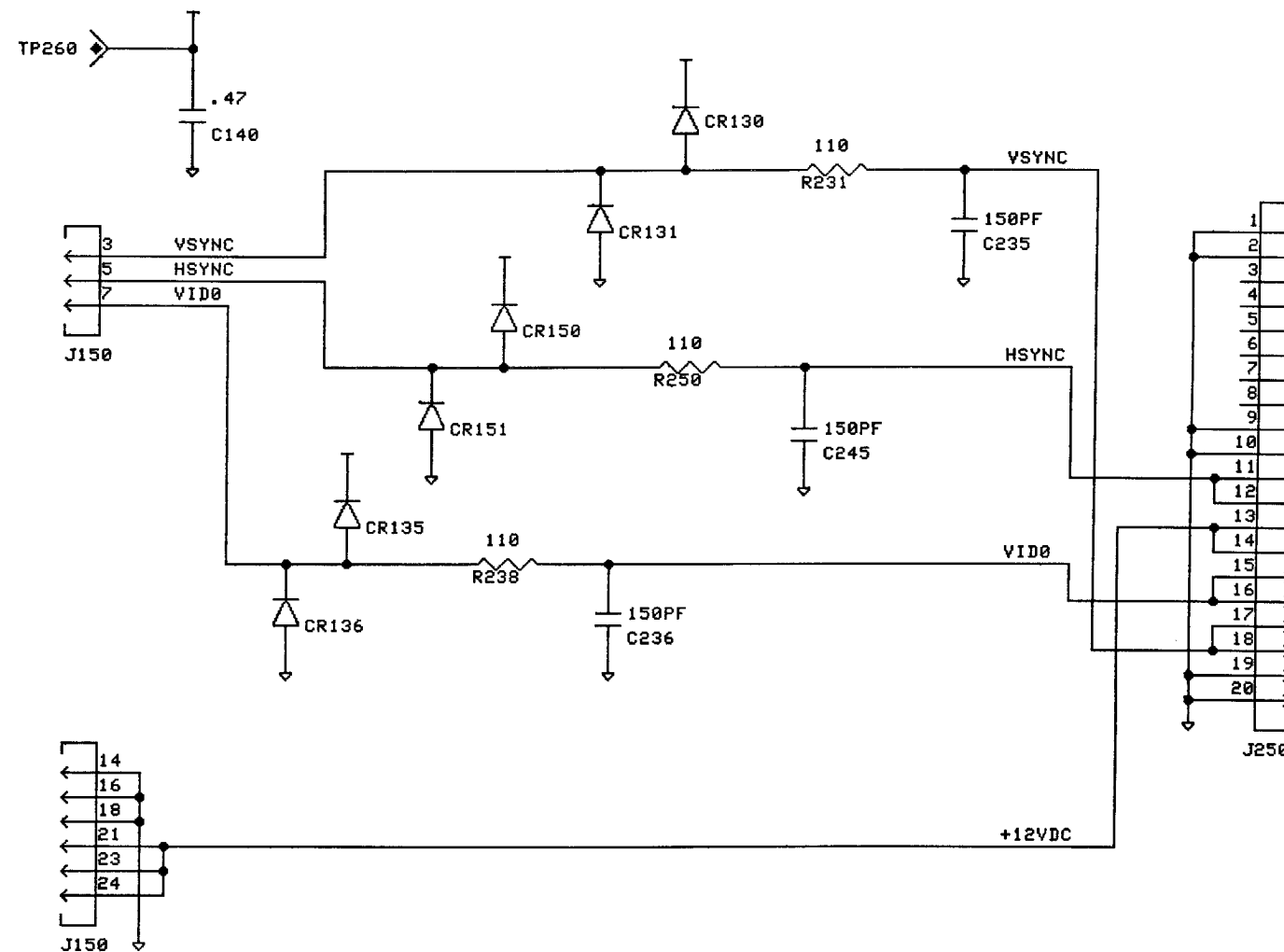
VIDEO INTERCONNECT
