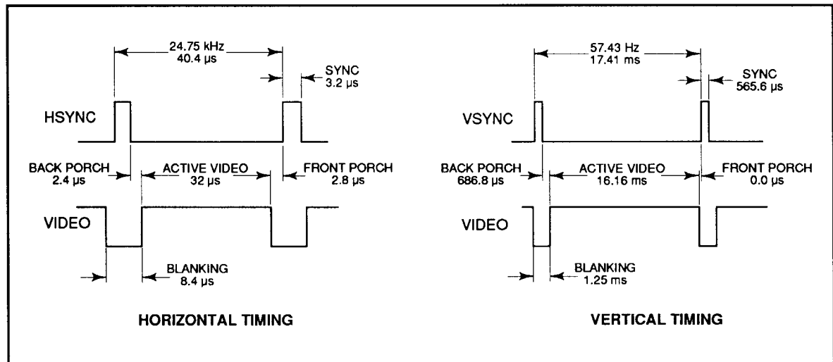
Figure 2-3. Video timing.
