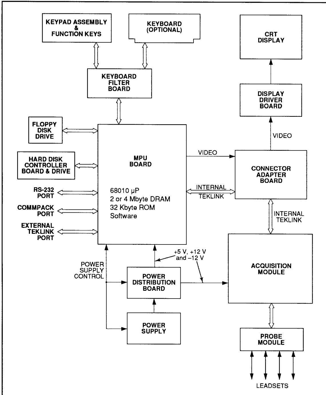
Figure 1-1. Configuration diagram.
