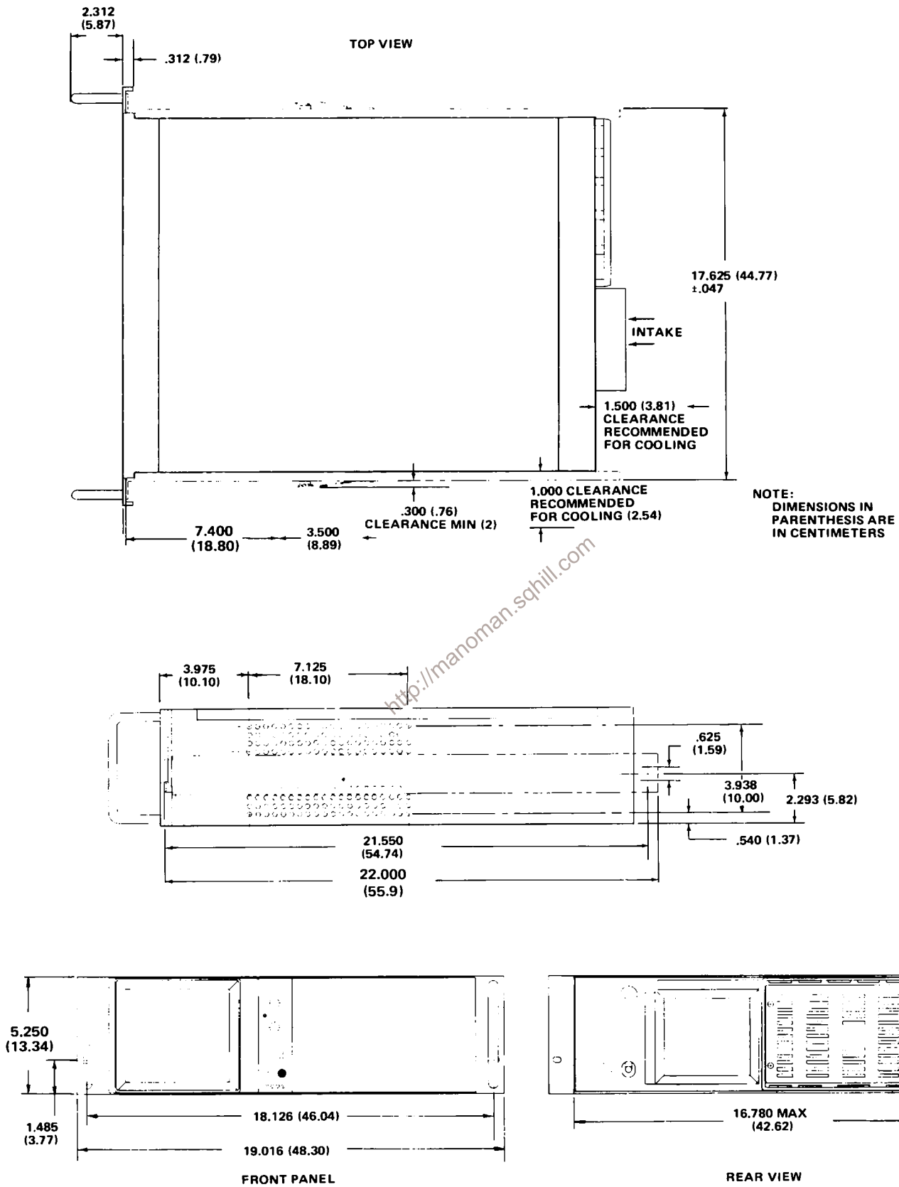
Fig. 6-6. Dimensional drawing.
