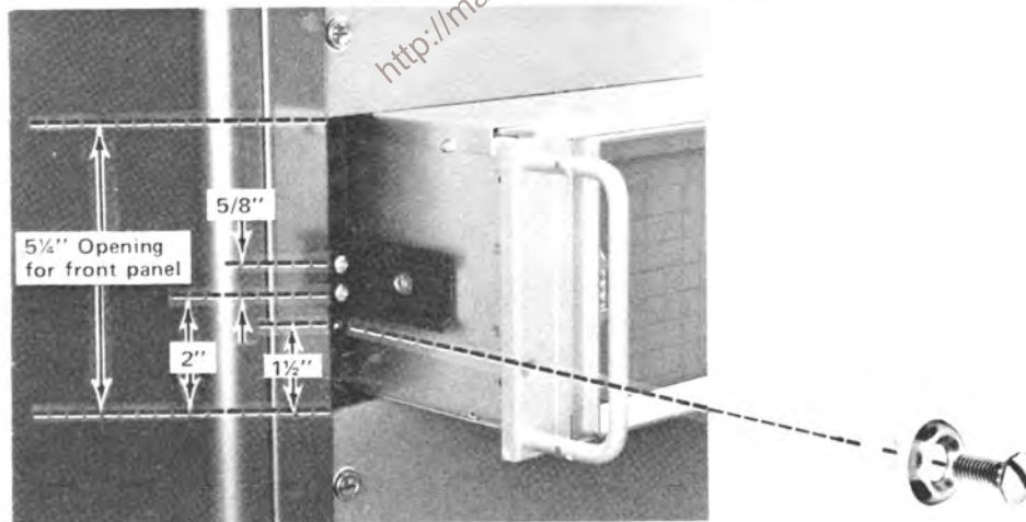
Fig. 6-2. Locating the mounting holes for the left stationary section. Same dimensions apply to right stationary section.
