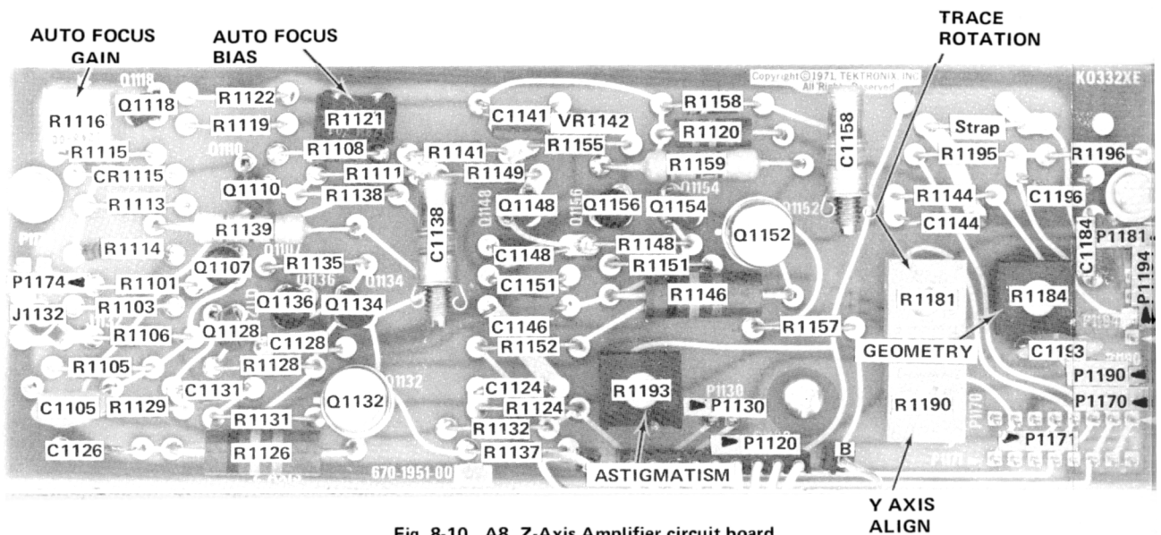
Fig. 8-10. A8. Z-Axis Amplifier circuit board.
