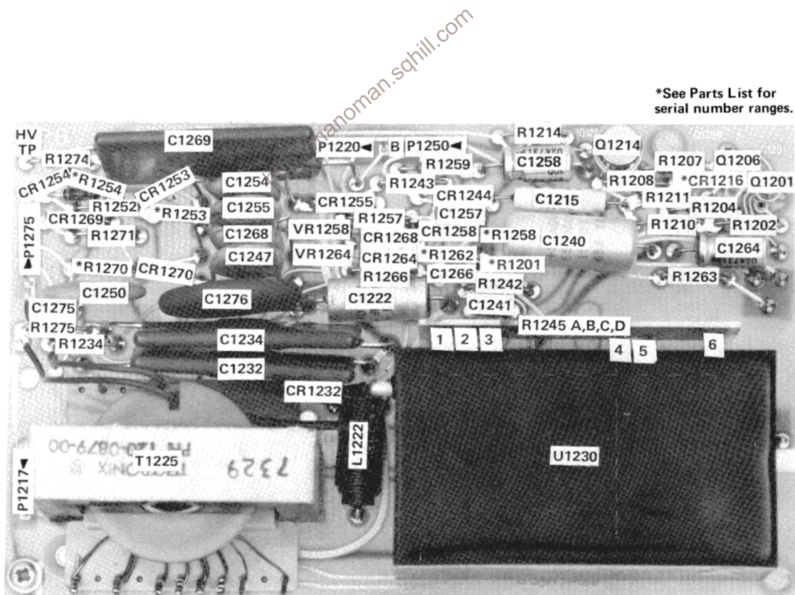
Fig. 8-11A. A9. High Voltage circuit board SN B100000-up.
