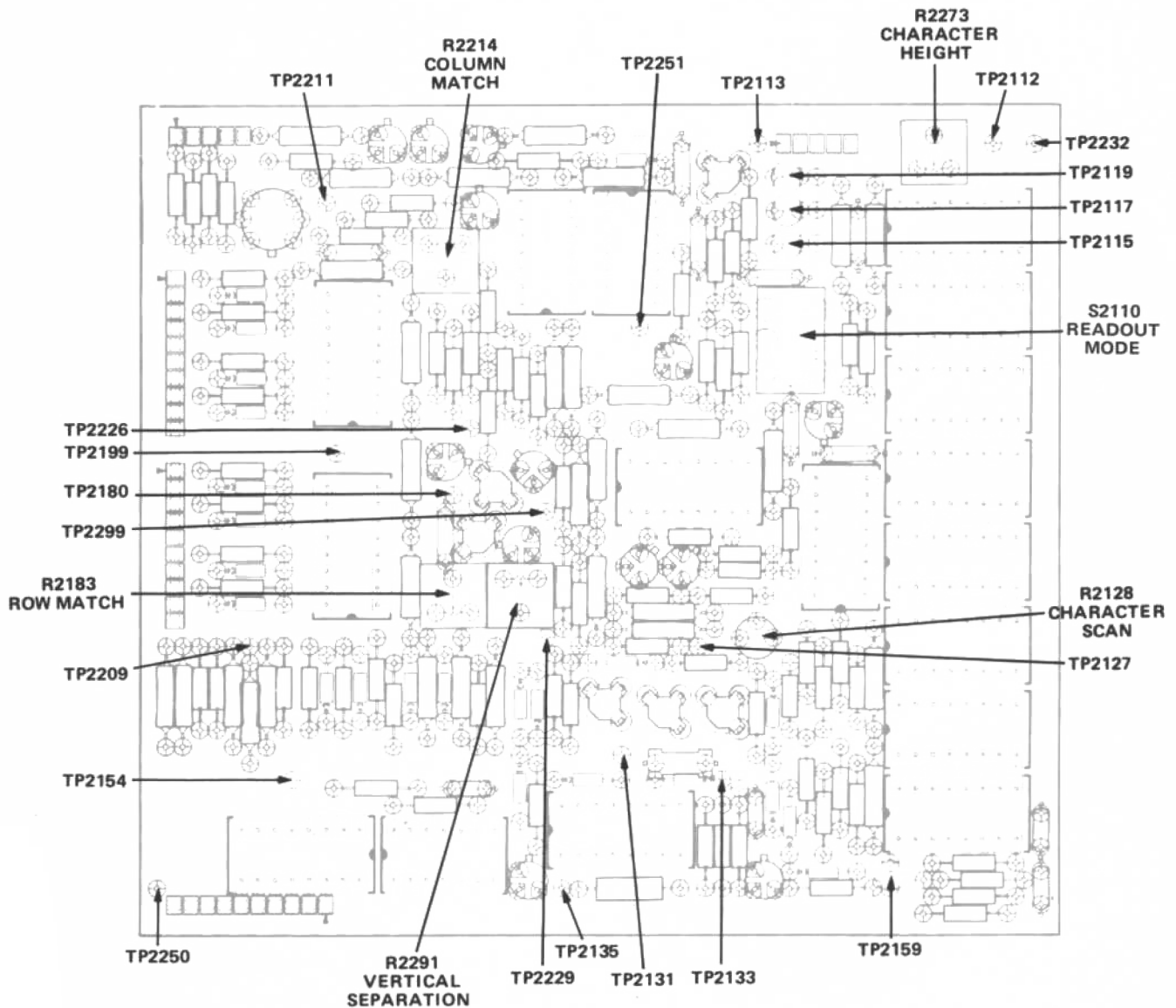
Figure 8-23. Readout board.
