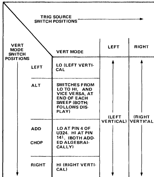
Figure 3-14. Input levels at pin 4 of U324.
