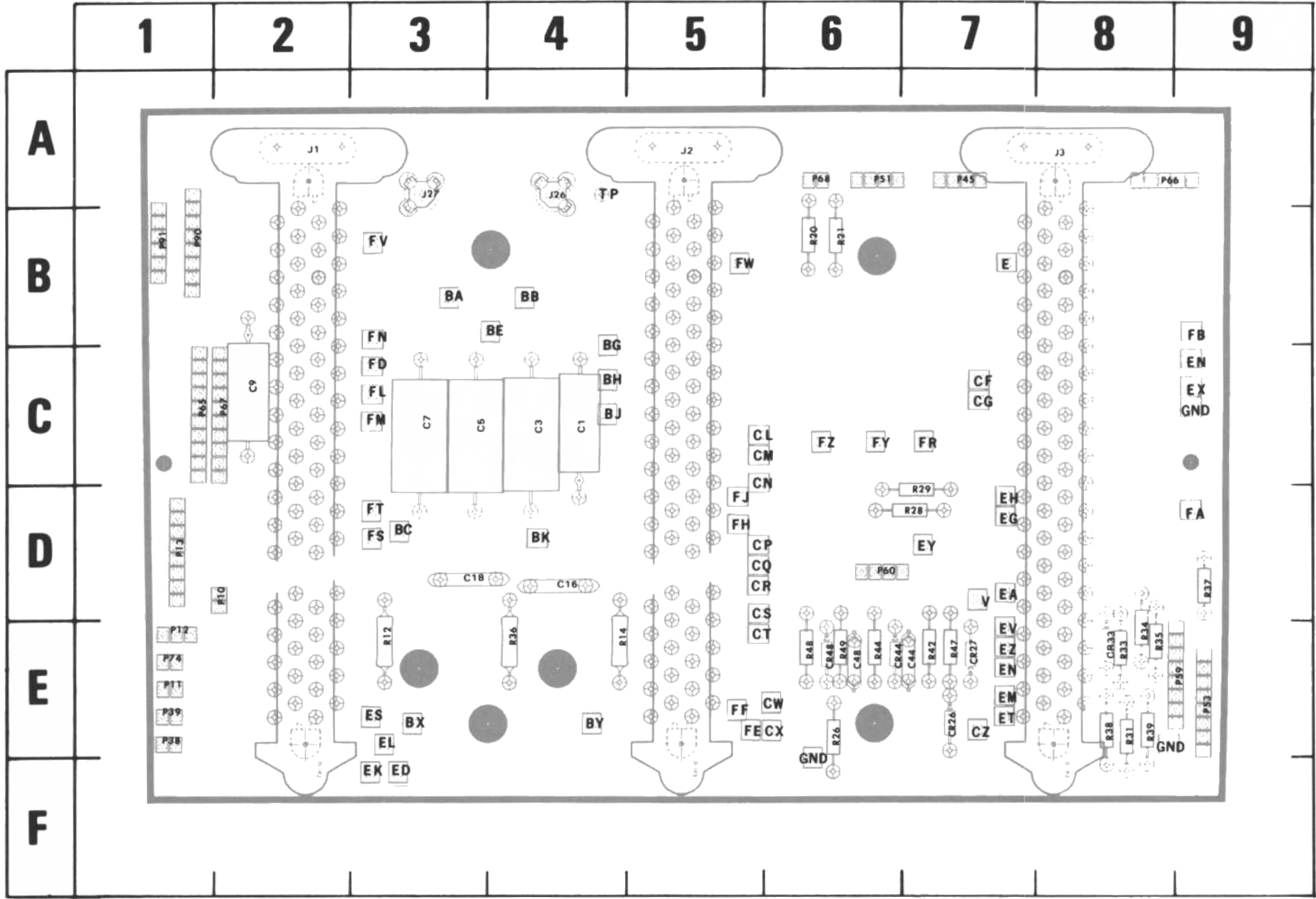
Figure 8-2. A1-Main Interface board.
