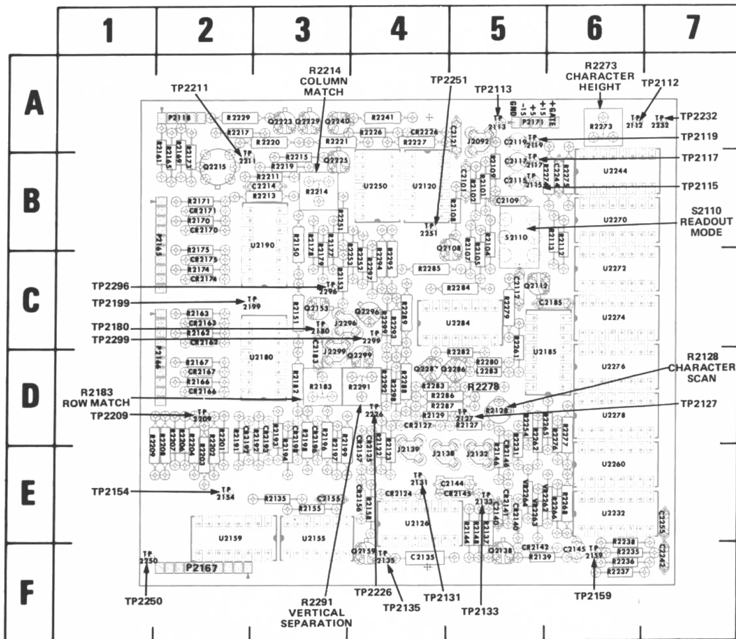
Figure 8-15. A13-Readout board.
