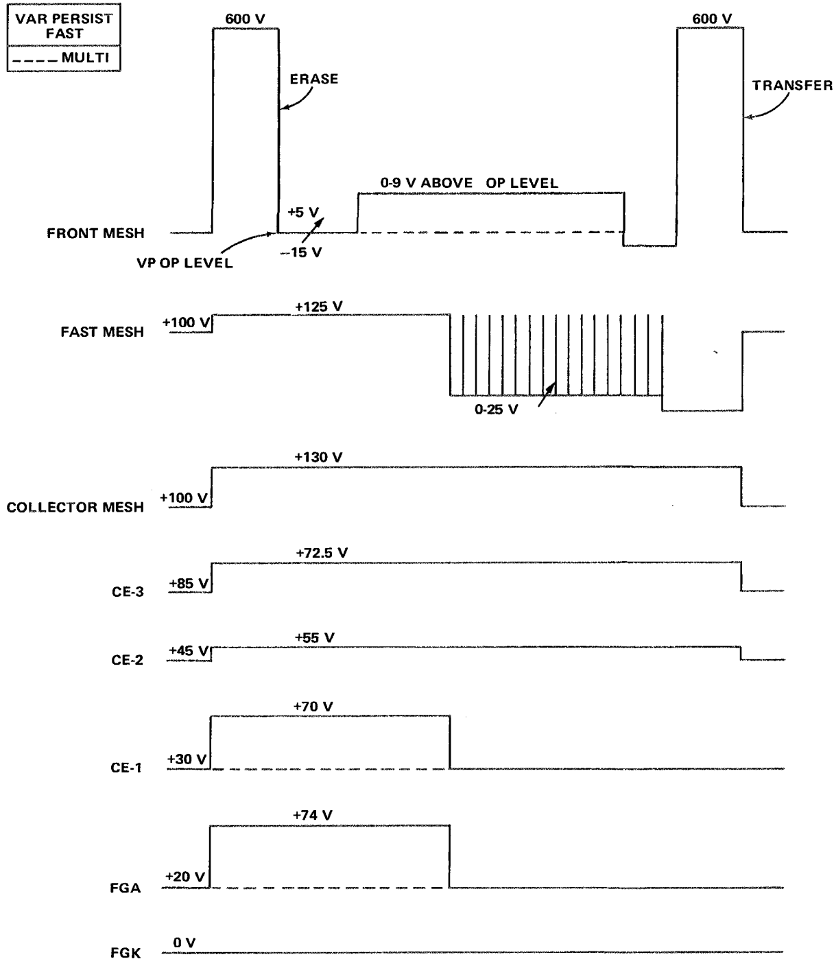
Figure 3-43. FAST VAR PERSIST mode Storage waveforms.
