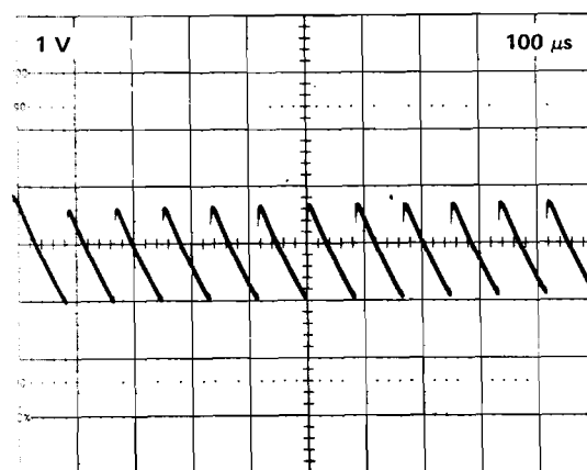
Figure 5-10. VAR PERSIST Front Mesh ramp.
