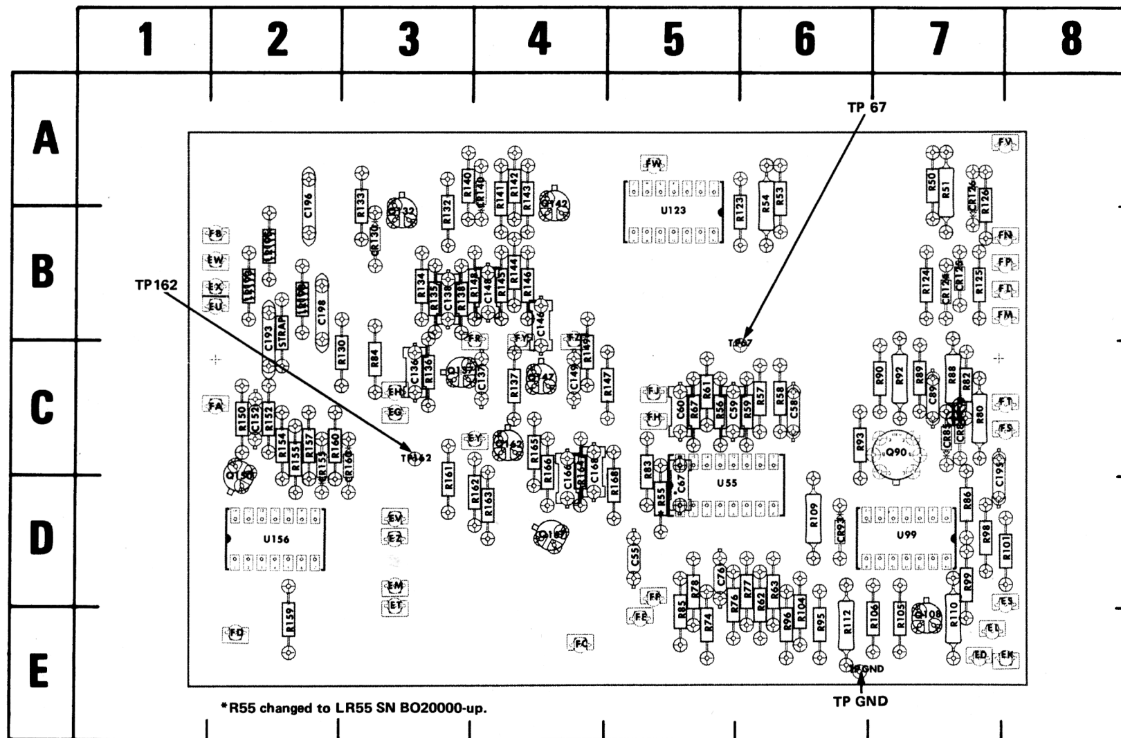
Figure 8-3. A2-Logic board.
