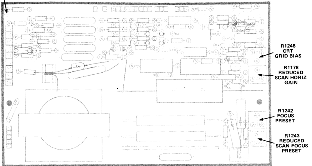
Figure 8-18. High-Voltage board.
