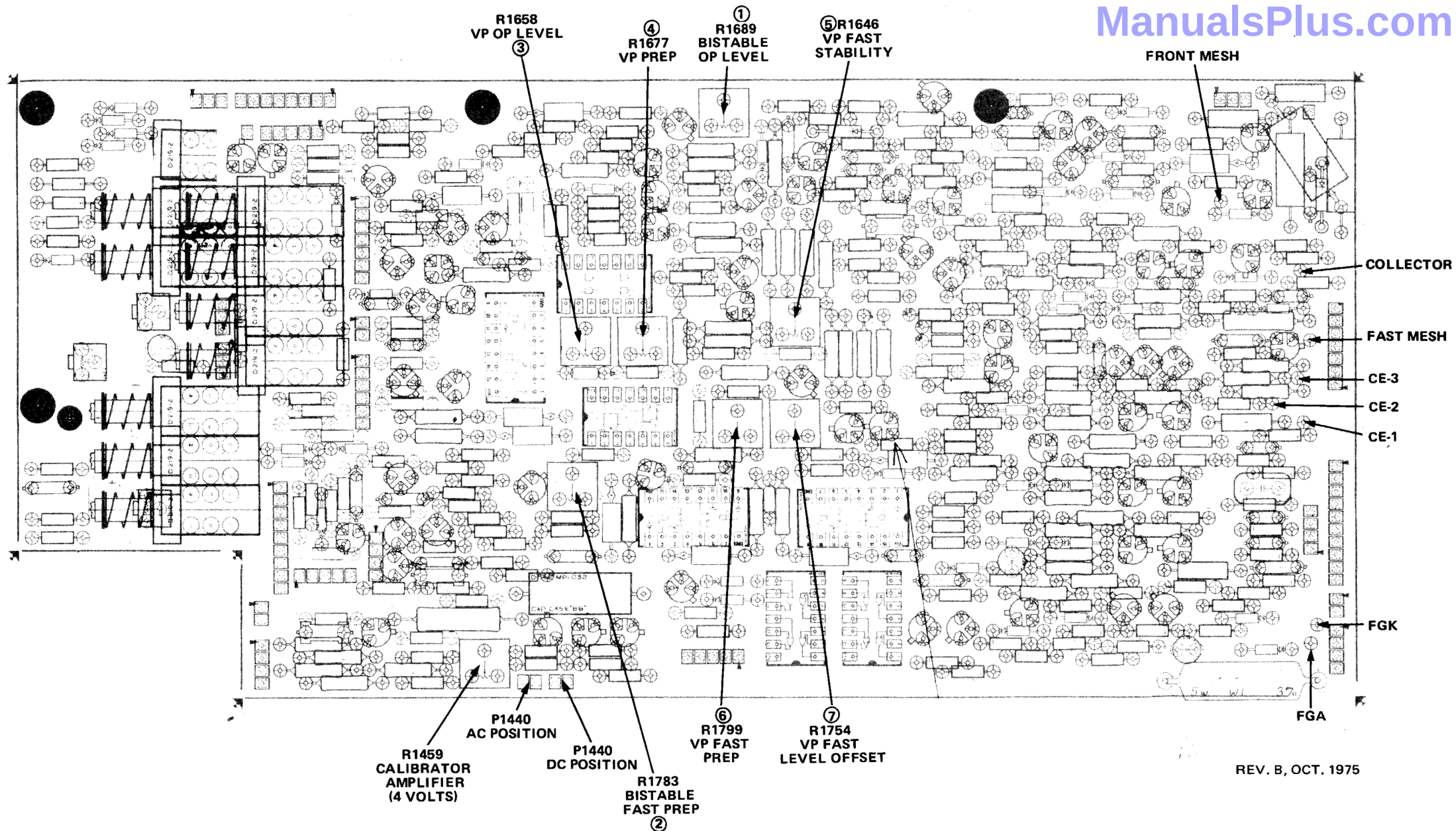
Figure 8-24. Storage board.
