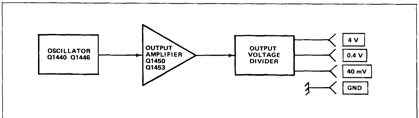
Figure 3-23. Calibrator detailed block diagram.
