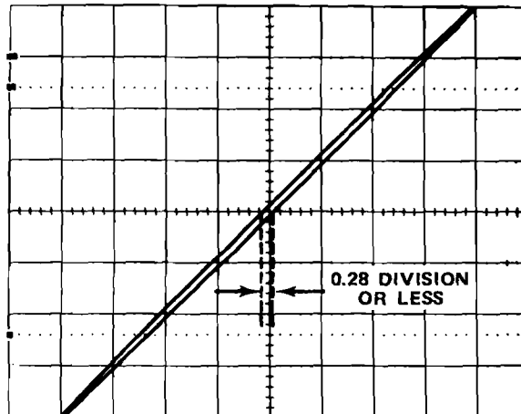
Figure 5-6. Typical crt display when checking X-Y phase shift.
