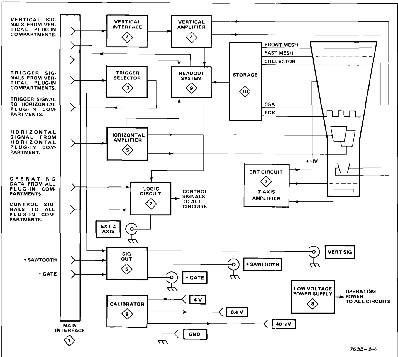
Figure 3-1. Block diagram 7633.
