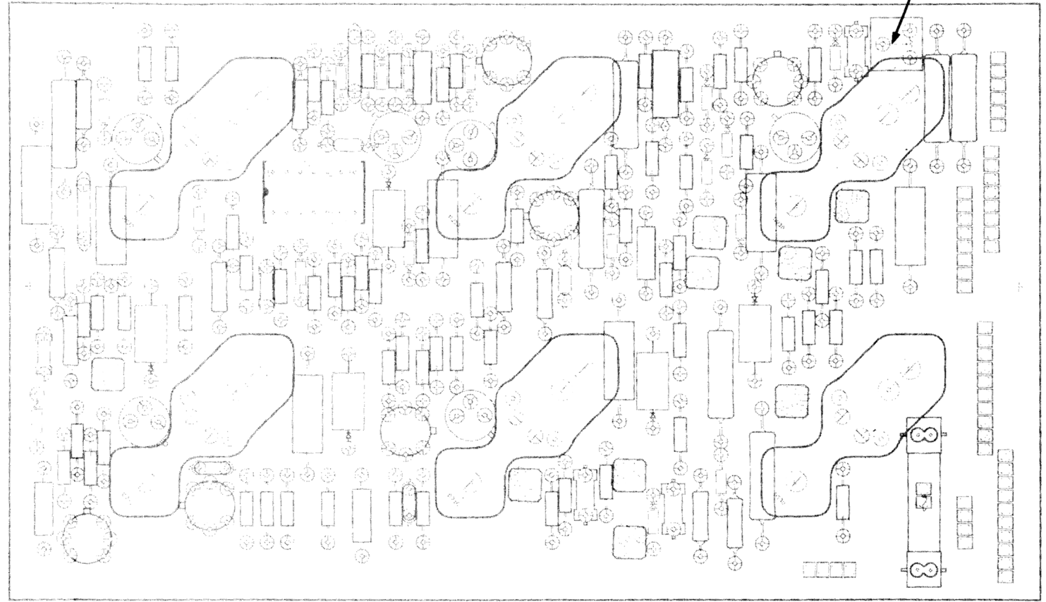
Figure 8-23. Low-Voltage Regulator board.
