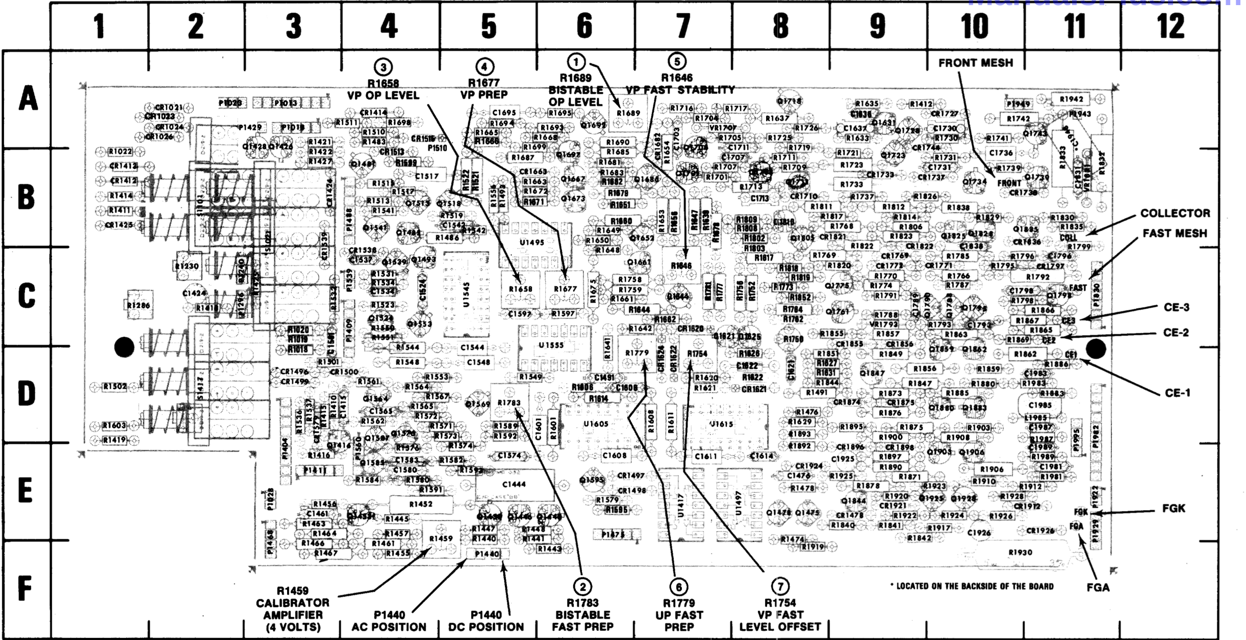
Figure 8-16A. A14-Storage board, SN B150000 — UP.
