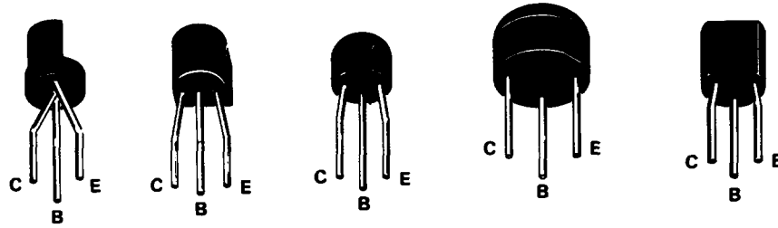
Plastic-Cased Transistors
