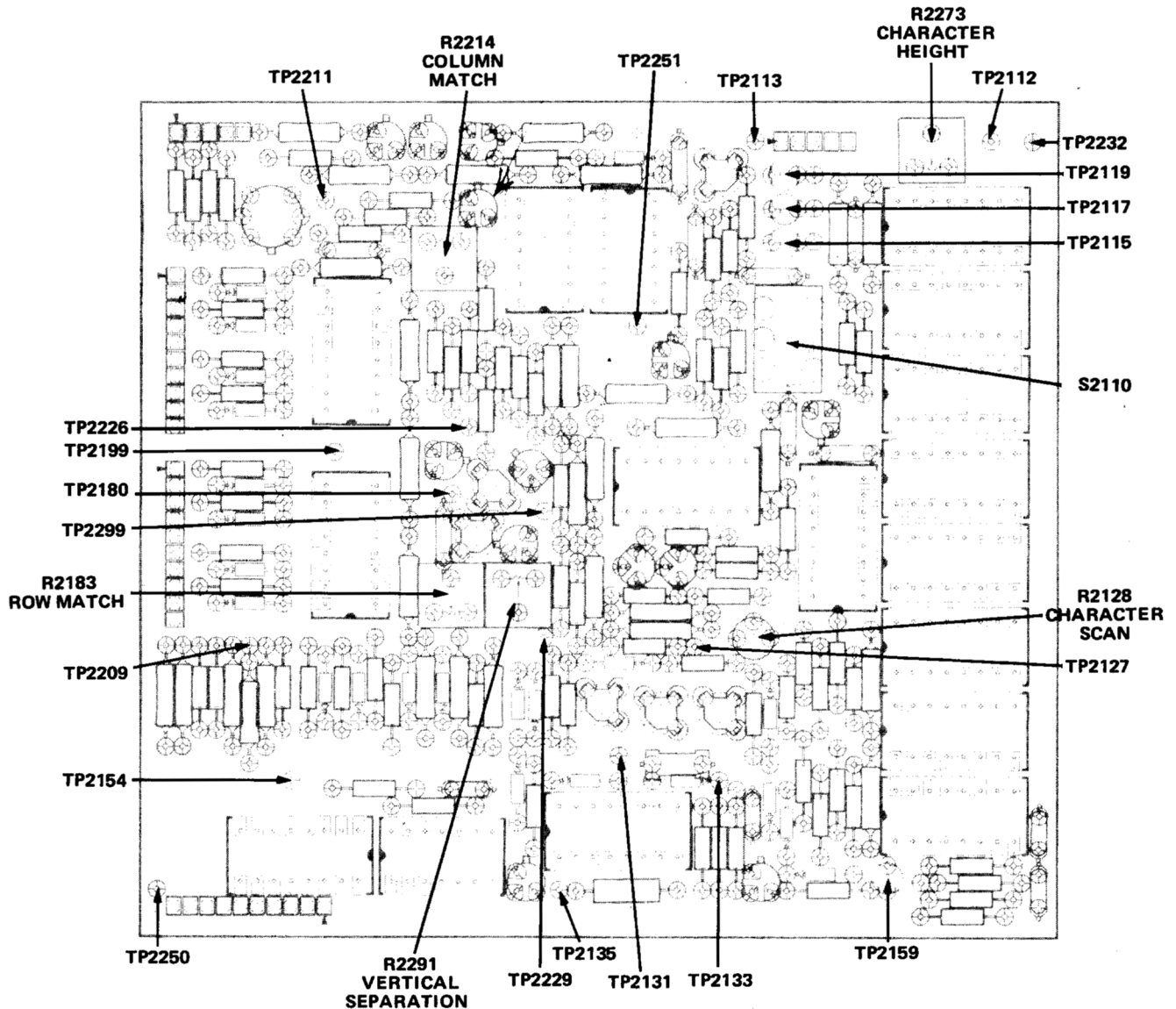
Figure 8-21. Readout board.
