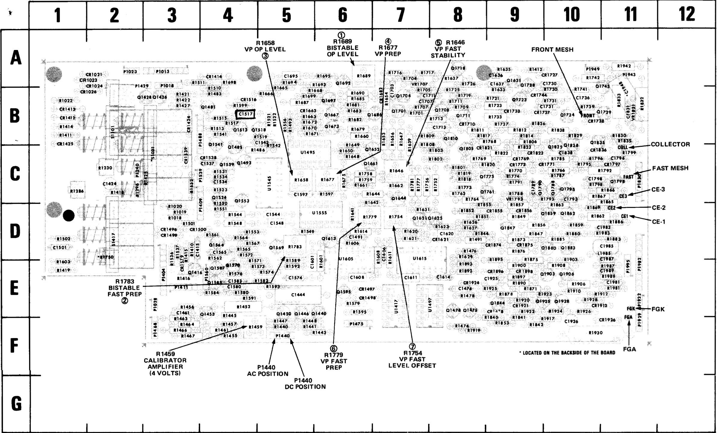
Figure 8-16B. A14-Storage board, SN B149999 — BELOW.
