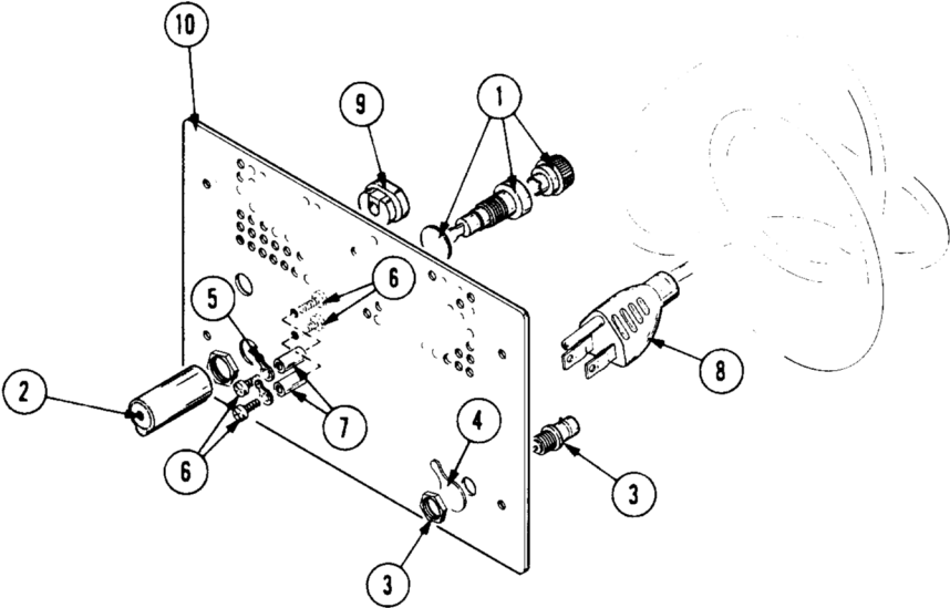
7633/R7633 OSCILLOSCOPE
