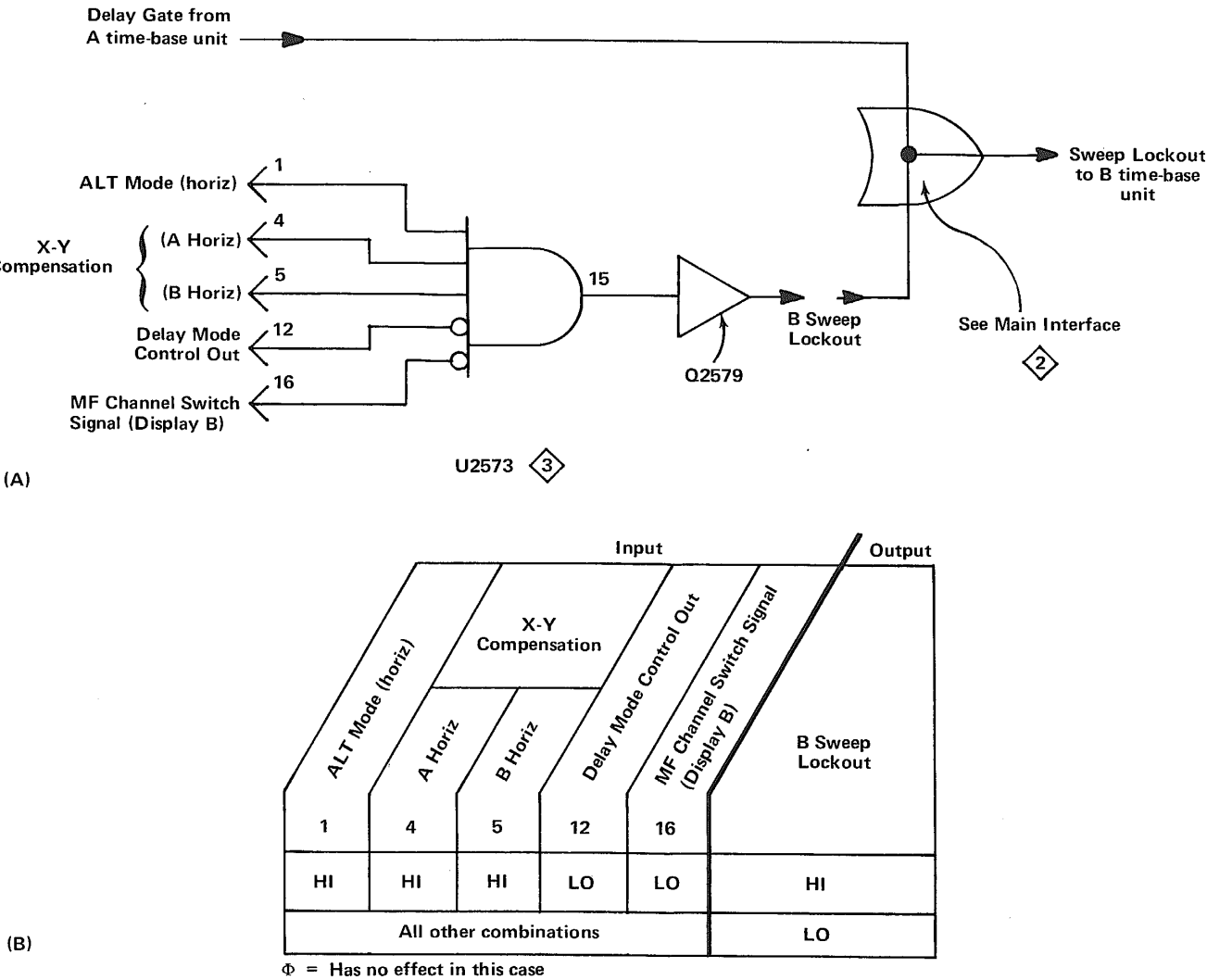
Fig. 2-6. (A) Logic diagram for B Sweep Lockout stage; (B) Table of input/output combinations.
