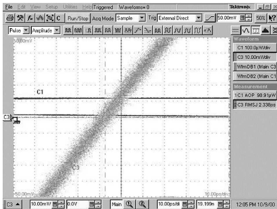
Figure 4- 52: Example of the display zoomed in to 10 mV/div and 10 ps/div at the crossing point (50%) on the recovered clock signal (C3).
