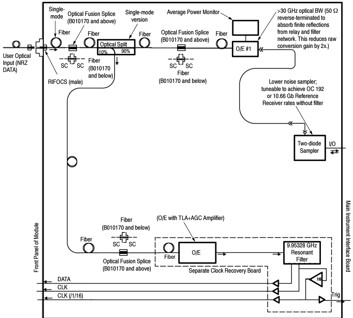
Figure 9- 10: 80C04 Optical sampling with CR-1 clock recovery block diagram
