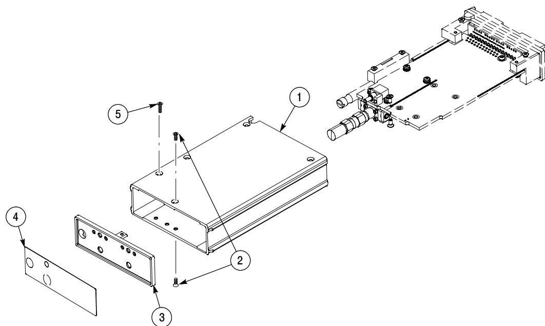
Figure 10-7: 80E06 module
