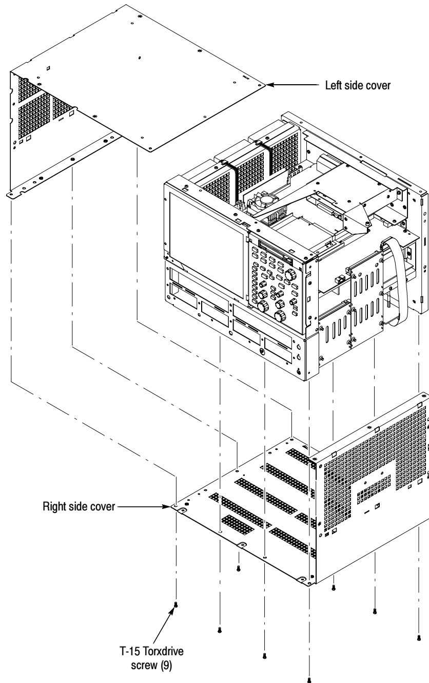
Figure 6-5: Cover removal
