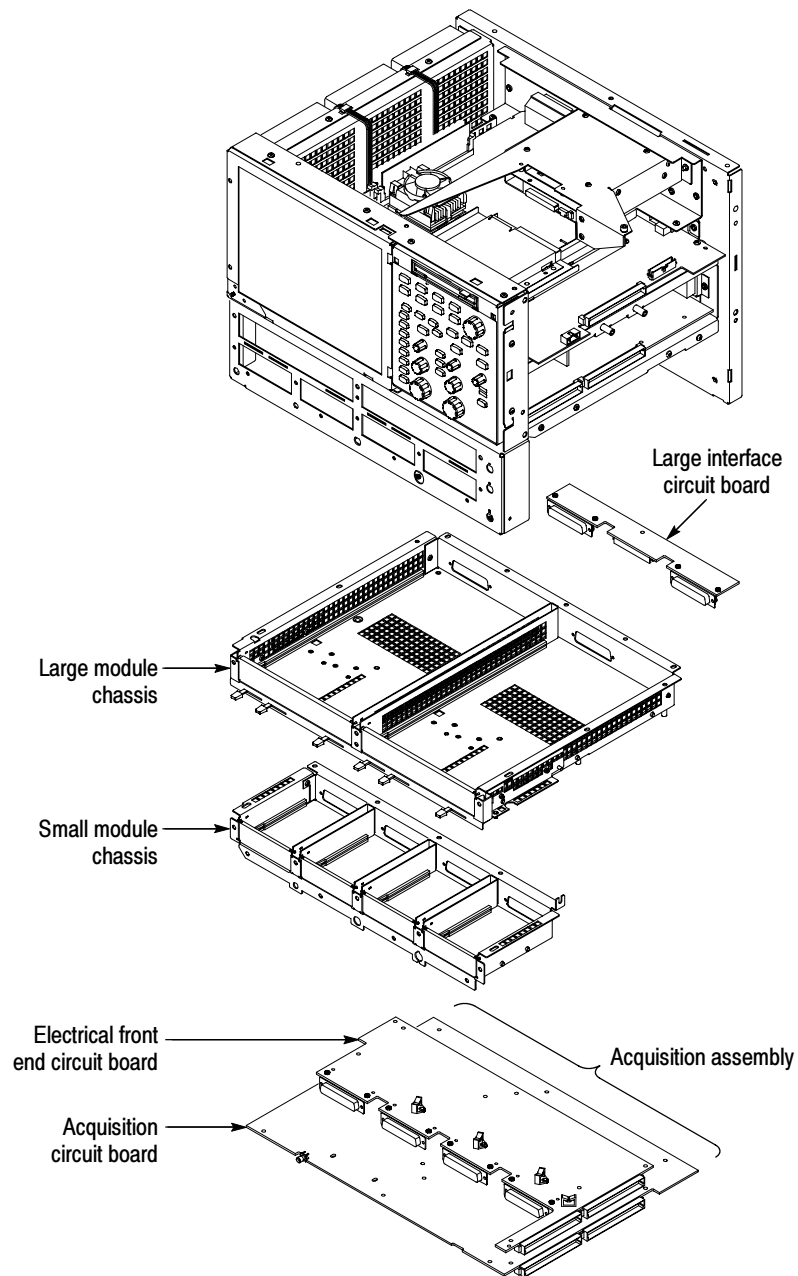
Figure 6-9: Acquisition modules
