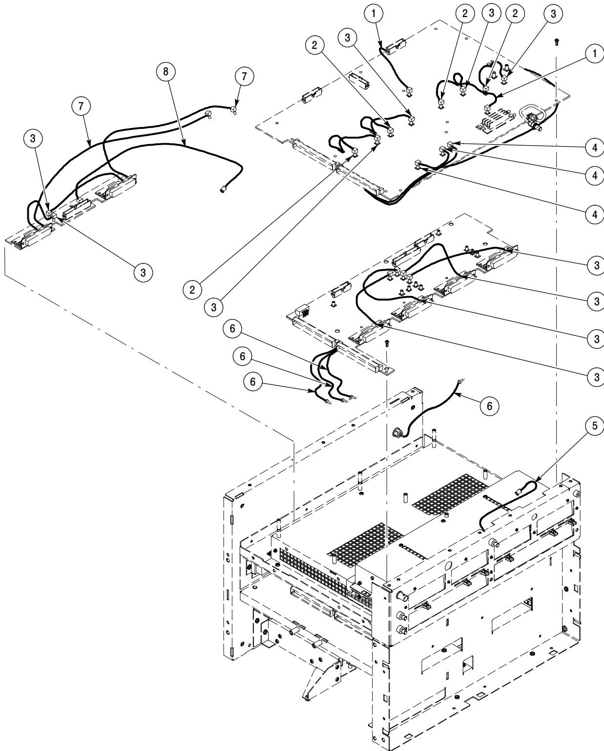
Figure 10-5: Coaxial cables
