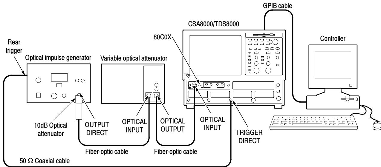
Figure 4-44: Minimum optical bandwidth and reference receiver frequency response hookup
