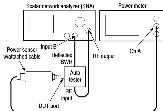
Figure 4-32: Hookup to measure Power in
