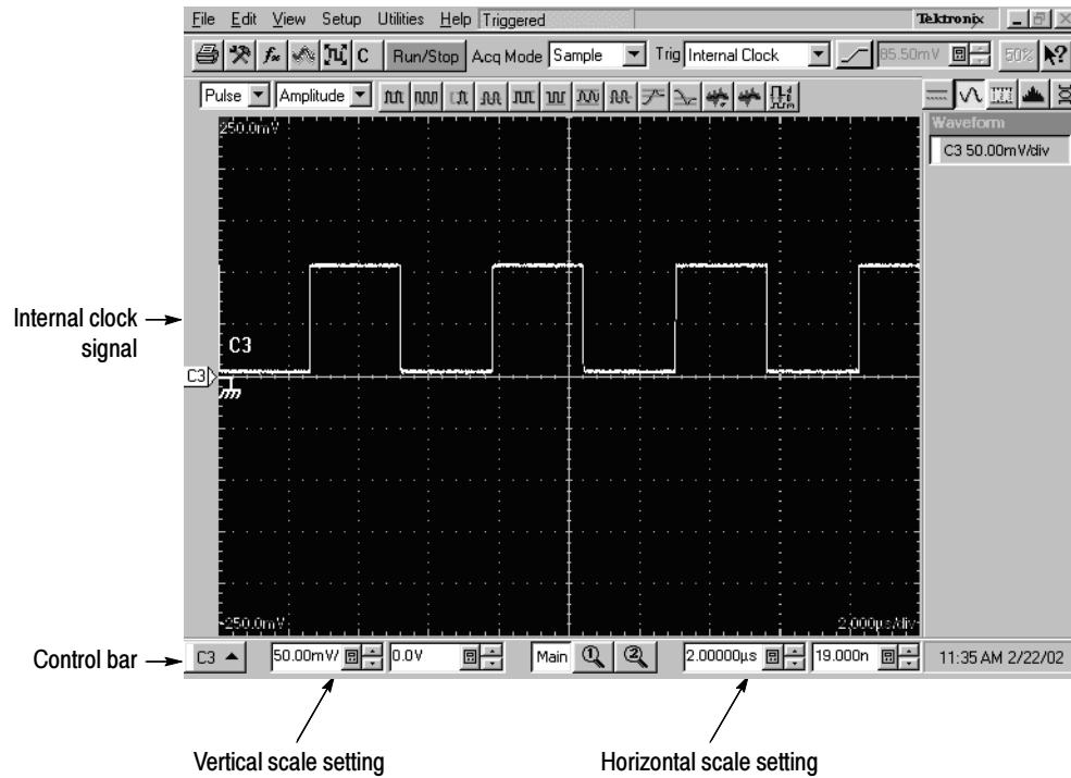
Figure 4-12: Signal triggered
