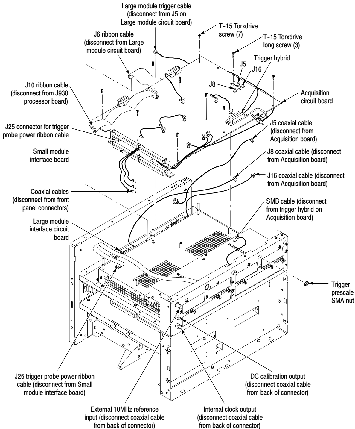
Figure 6-31: Acquisition circuit board assembly removal (8000B)
