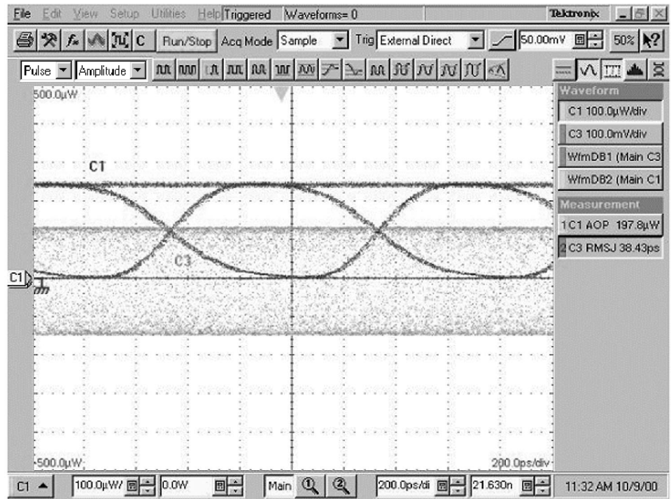
Figure 4-50: Example of the display when the clock signal from the 80C0X-CR Optical Sampling Module is not synchronous with the data rate input from the pulse pattern generator. Note the unstable (“washed out”) clock signal. Compare this with Figure 4-51, in which the clock signal is synchronized.
