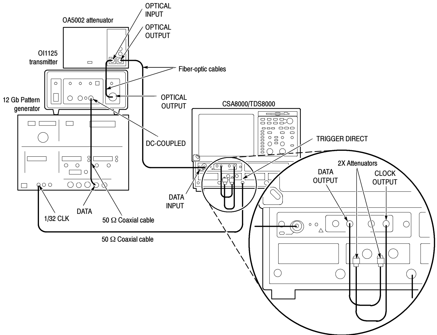
Figure 4-49: 80C01 and 80C03 clock recovery optical sensitivity range and recovered clock timing jitter hookup
