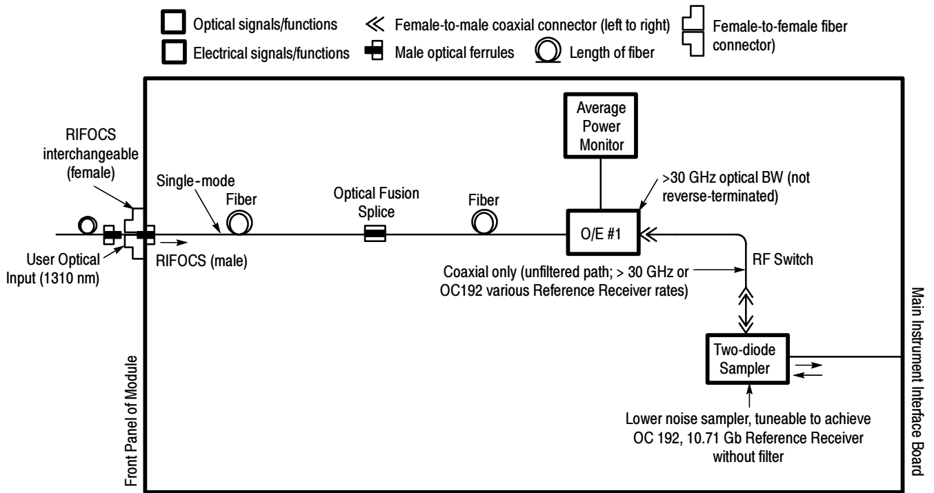
Figure 9-17: 80C09 Optical sampling block diagram (without clock recovery option)
