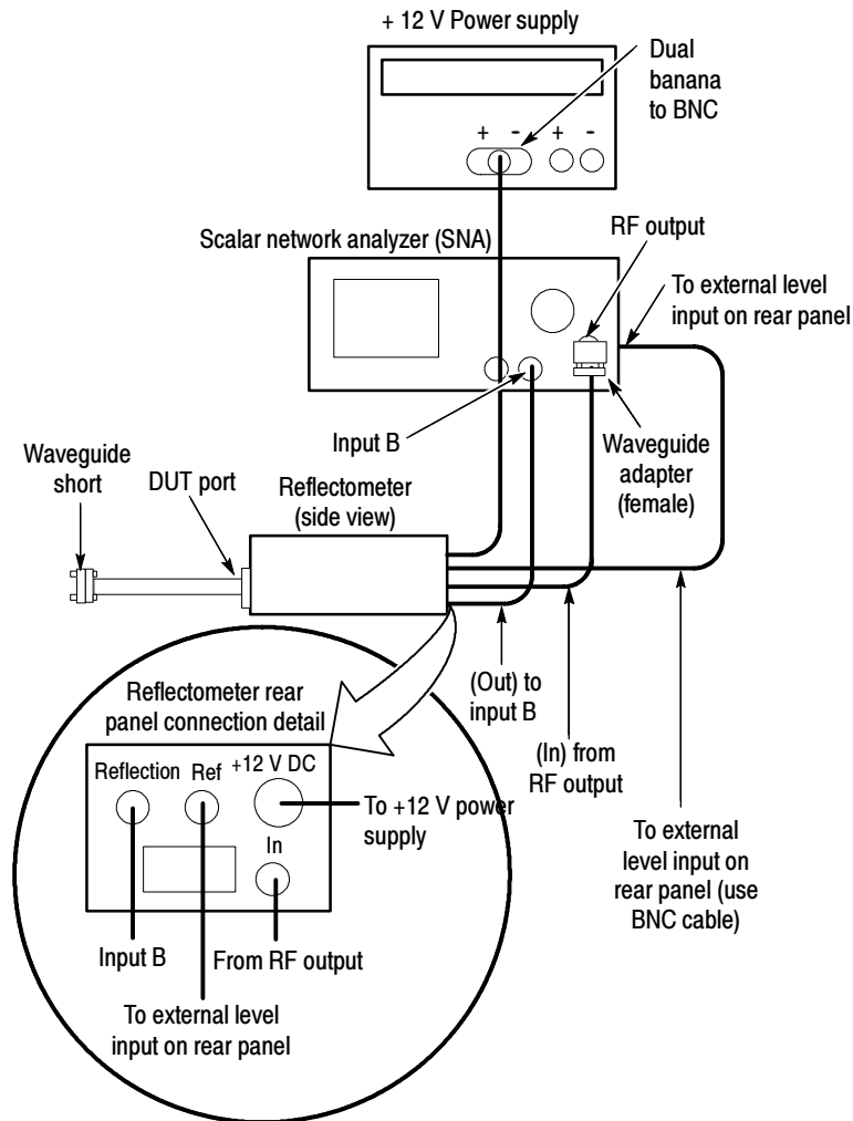
Figure 4- 36: SNA/Waveguide Characterization
