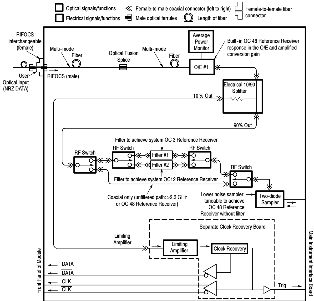
Figure 9- 14: 80C07- CR1 Optical sampling with clock recovery block diagram
