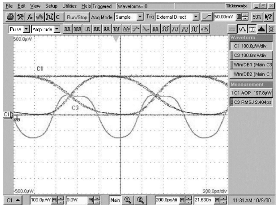
Figure 4-51: Example of the display when the clock signal from the 80C0X-CR Optical Sampling Module is synchronous with the data rate input from the pulse pattern generator. Note the stable clock signal waveform. Compare this with Figure 4-50, in which the clock signal is not synchronized.
