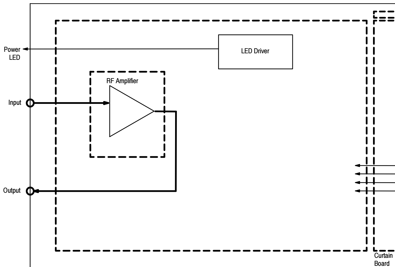
Figure 9-20: 80A01 block diagram
