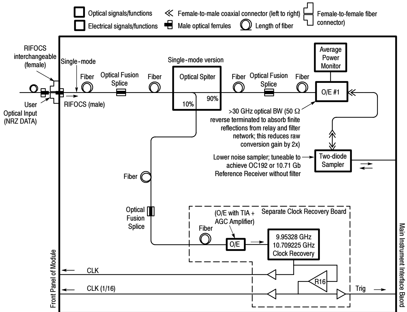
Figure 9-18: 80C09-CR1 Optical sampling with clock recovery block diagram
