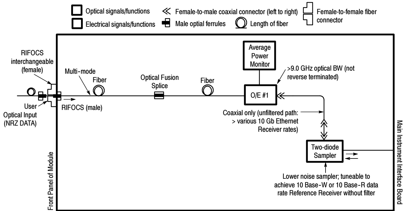
Figure 9-15: 80C08/80C08B Optical sampling block diagram (without clock recovery option)
