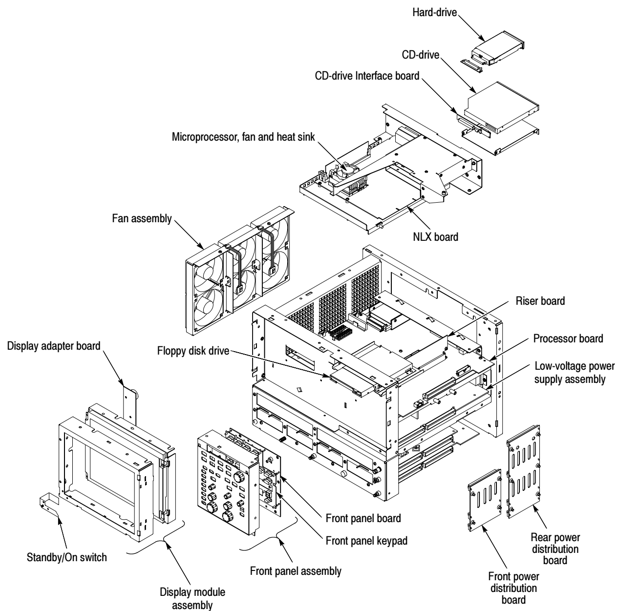
Figure 6-8: Internal modules
