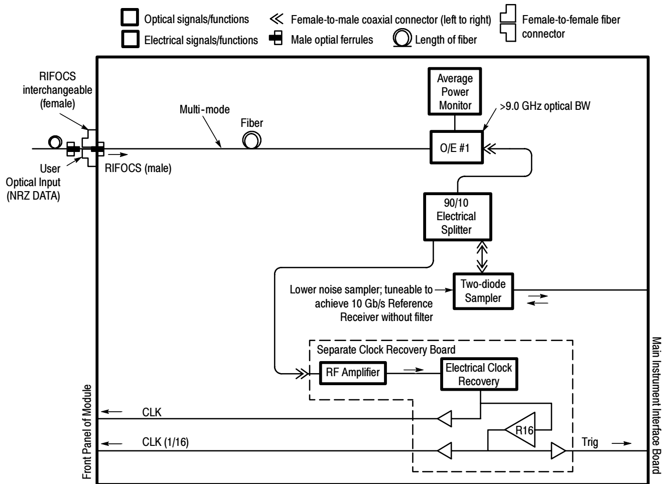
Figure 9- 16: 80C08/80C08B- CR1 & CR2 Optical sampling with clock recovery block diagram
