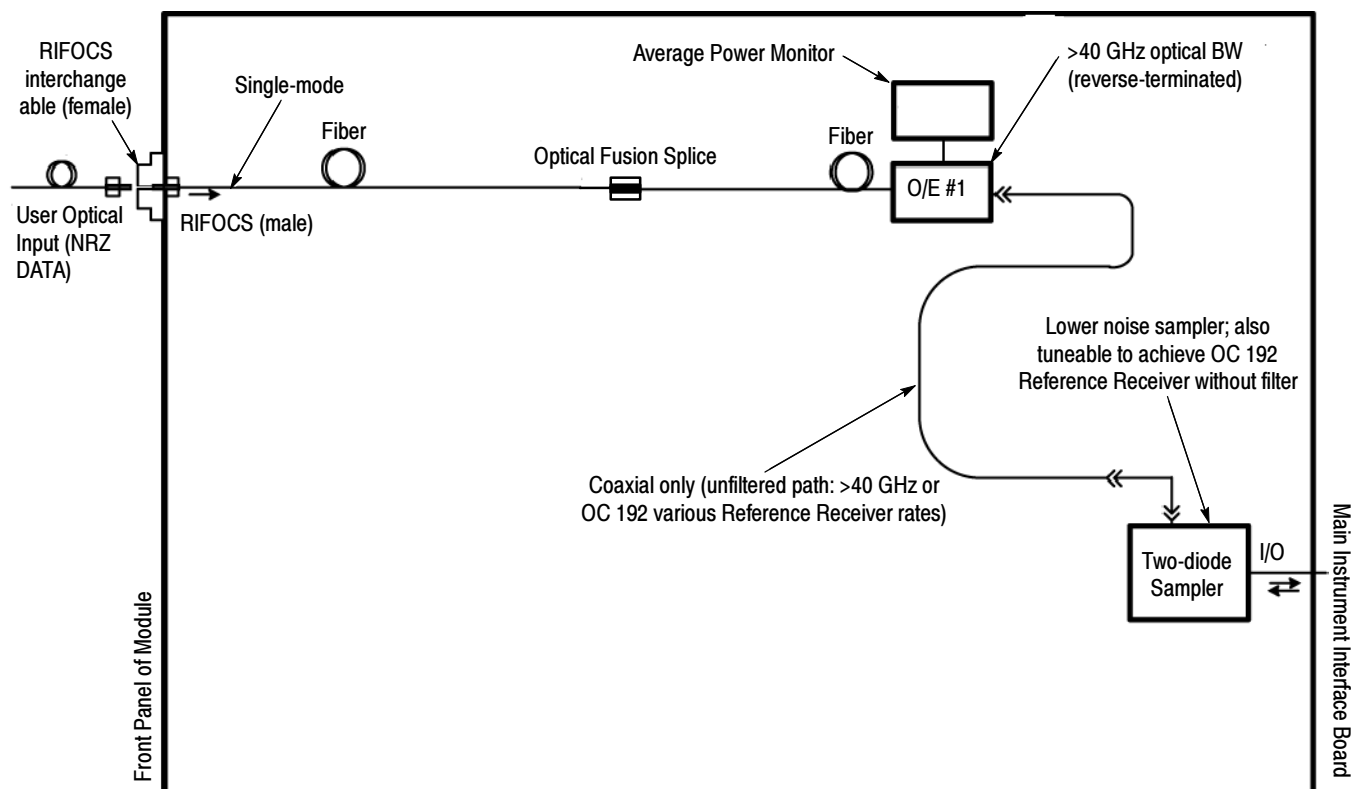
Figure 9- 11: 80C05 Optical sampling block diagram
