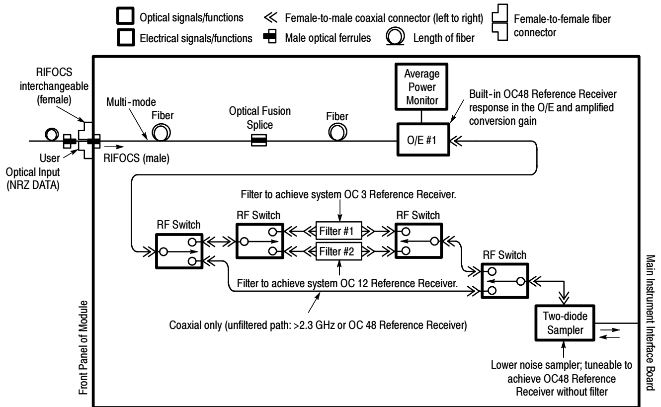
Figure 9-13: 80C07 Optical sampling block diagram
