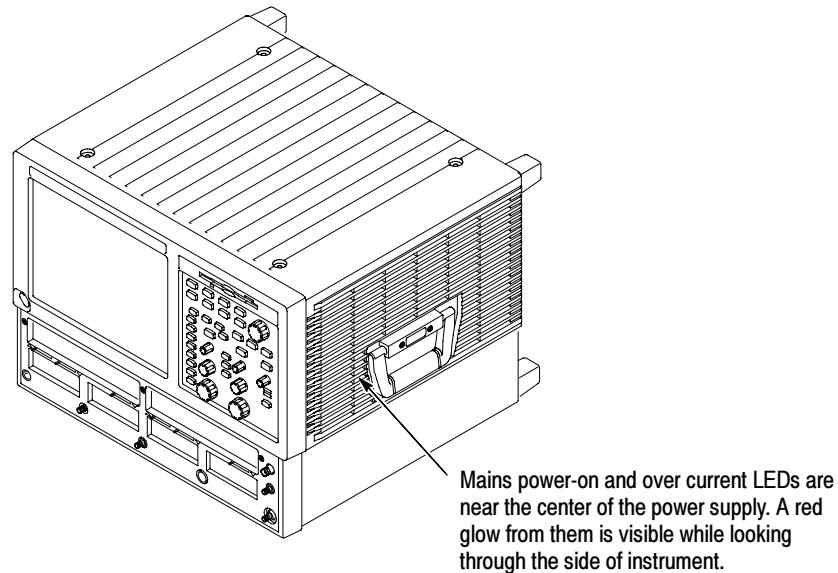
Figure 6-41: Location of power-on and over current LEDs
