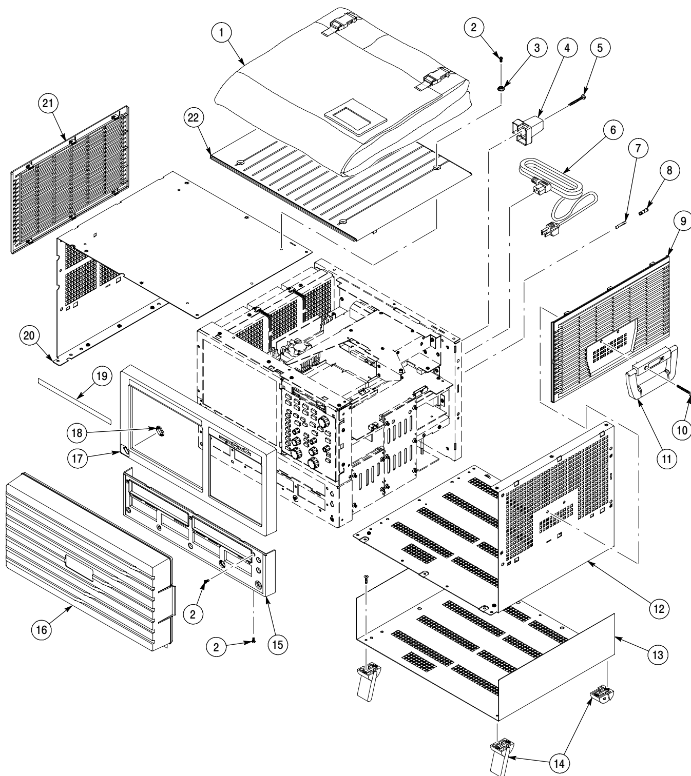
Figure 10-1: External parts
