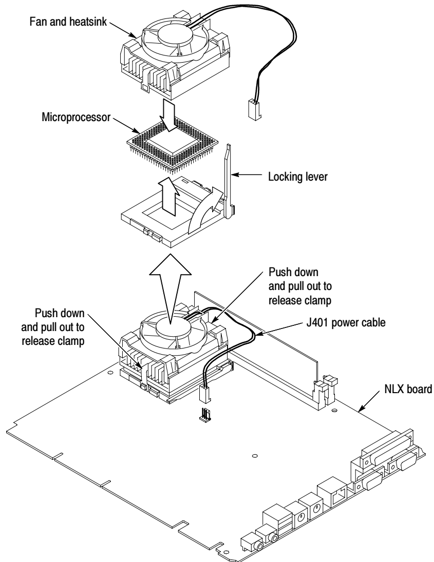
Figure 6-27: Microprocessor removal
