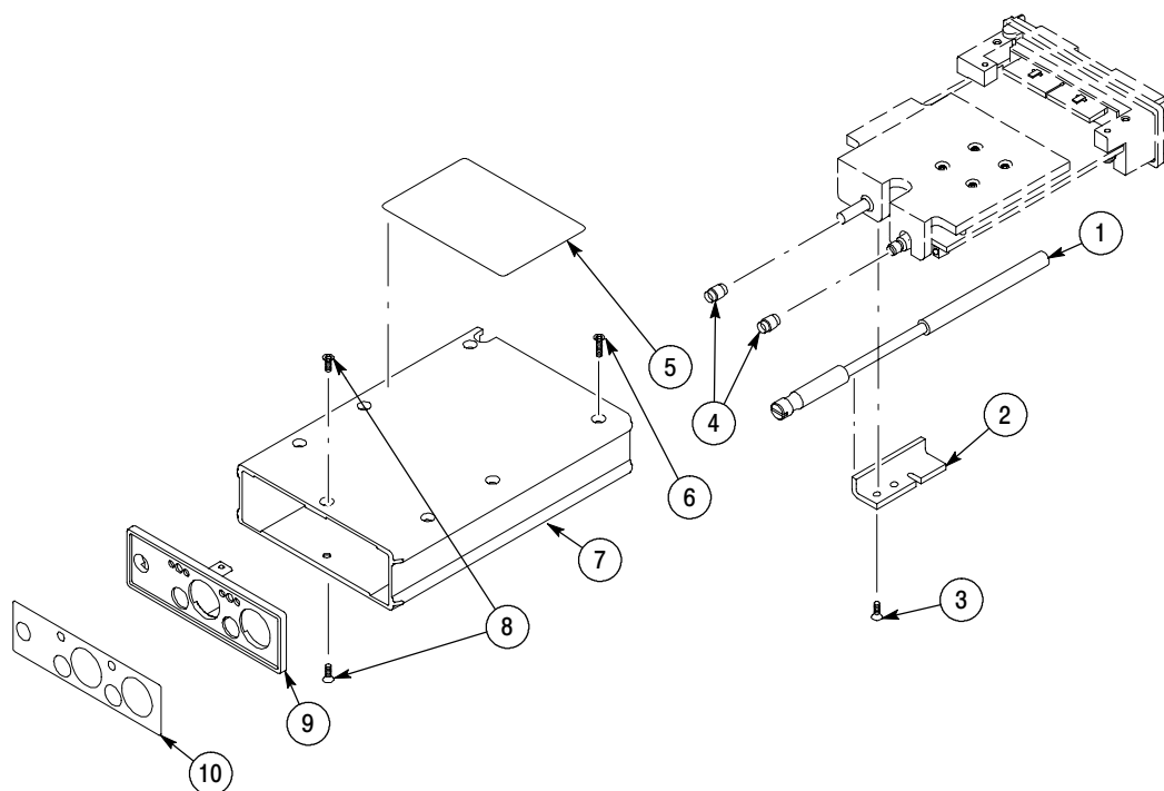
Figure 10-9: 80A01 module
