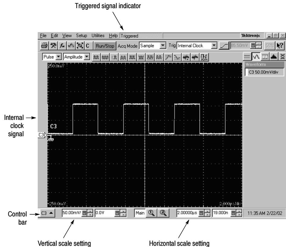
Figure 4- 15: Signal triggered
