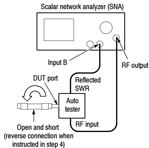
Figure 4- 30: SNA/Autotester Characterization
