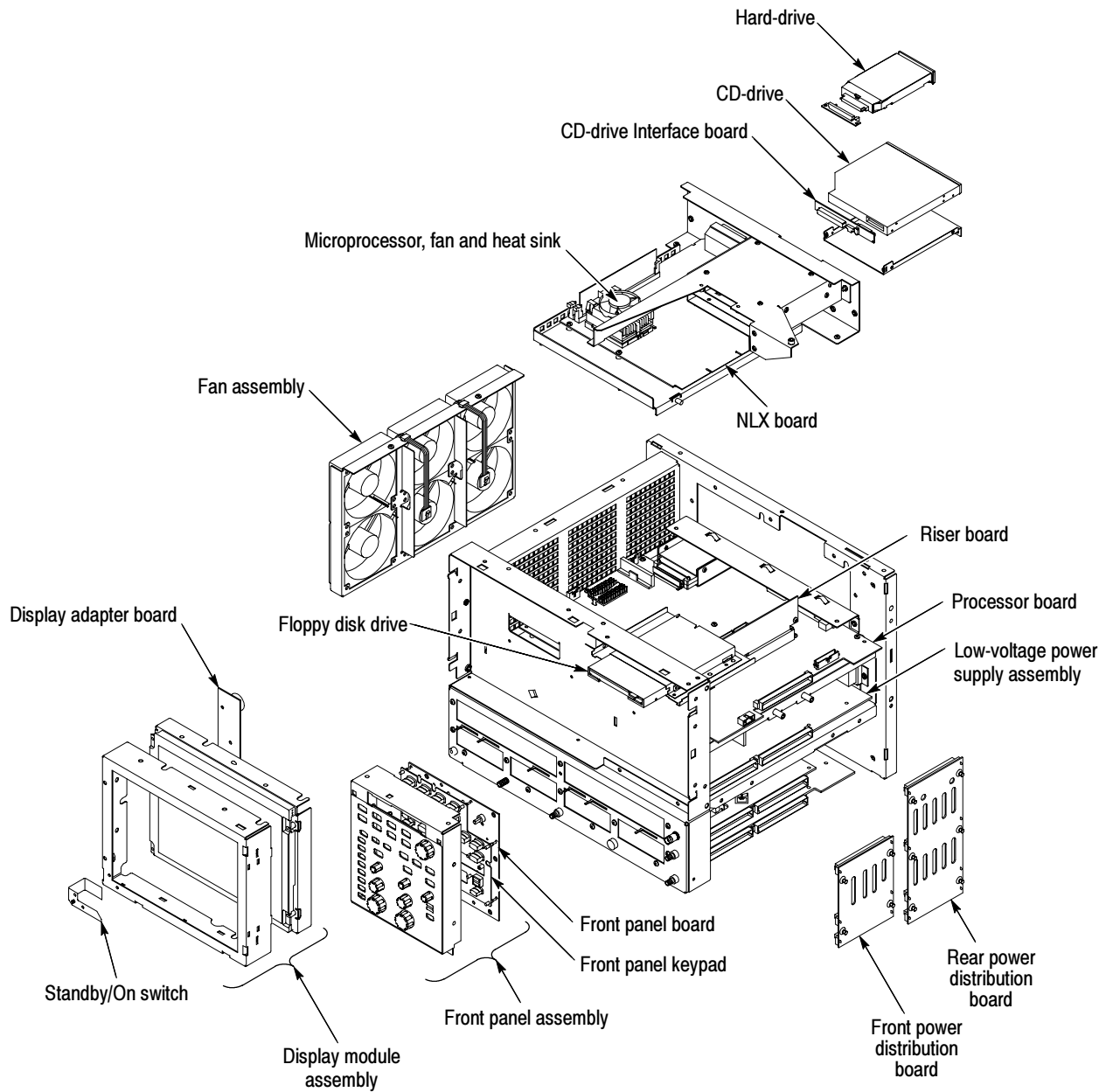
Figure 6-8: Internal modules
