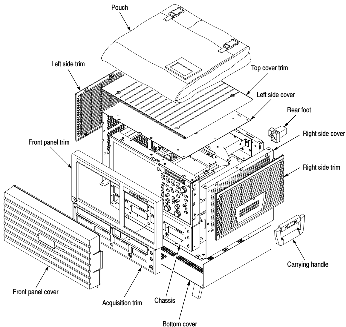
Figure 6-7: External modules
