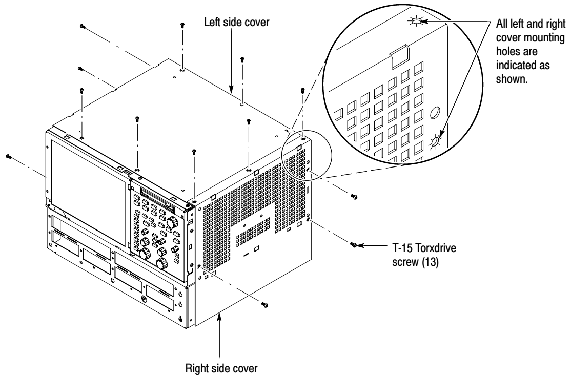
Figure 6-4: Cover removal
