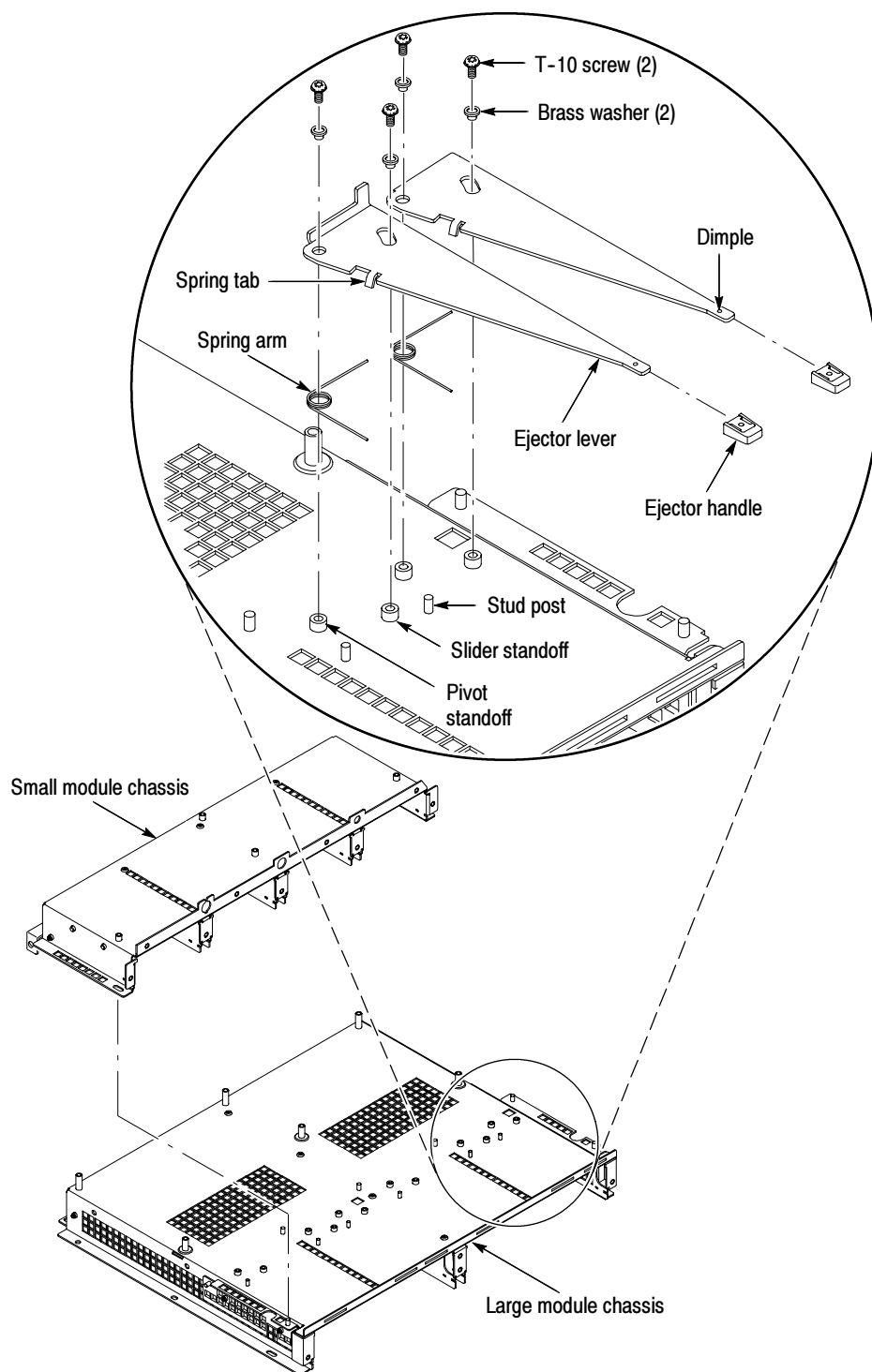
Figure 6-36: Module ejector handles removal
