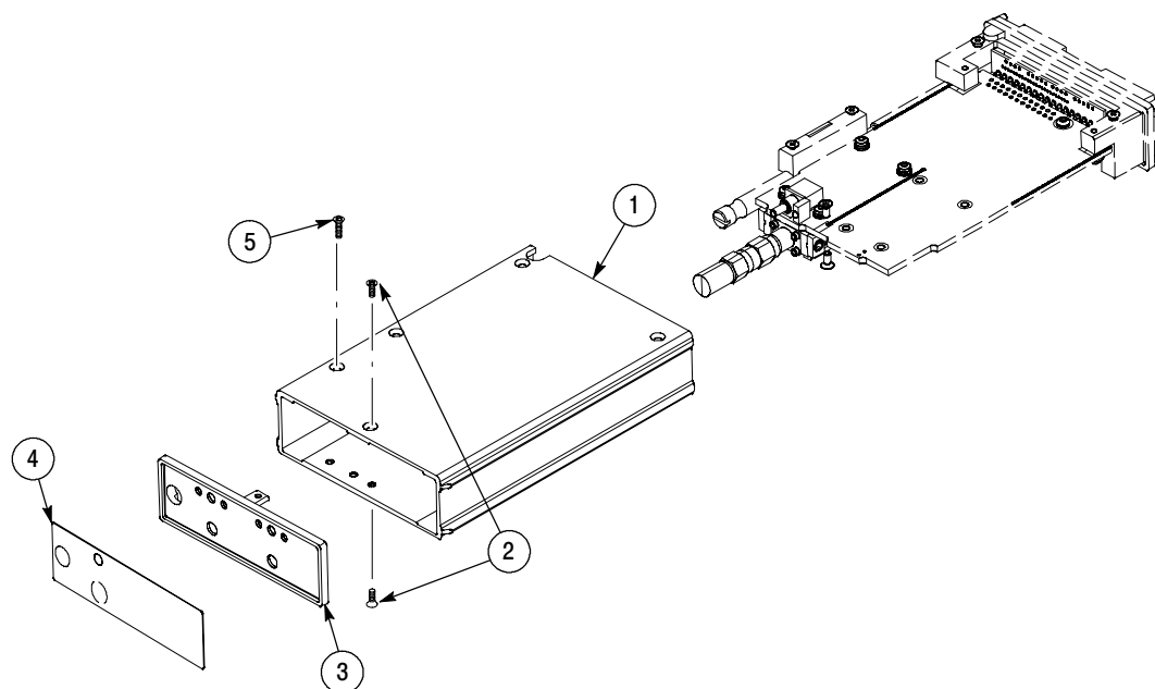
Figure 10-7: 80E06 module
