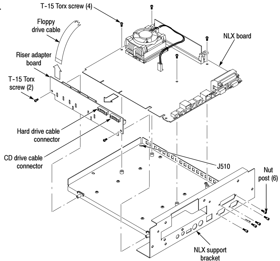
Figure 6-26: Riser adapter & NLX board removal
