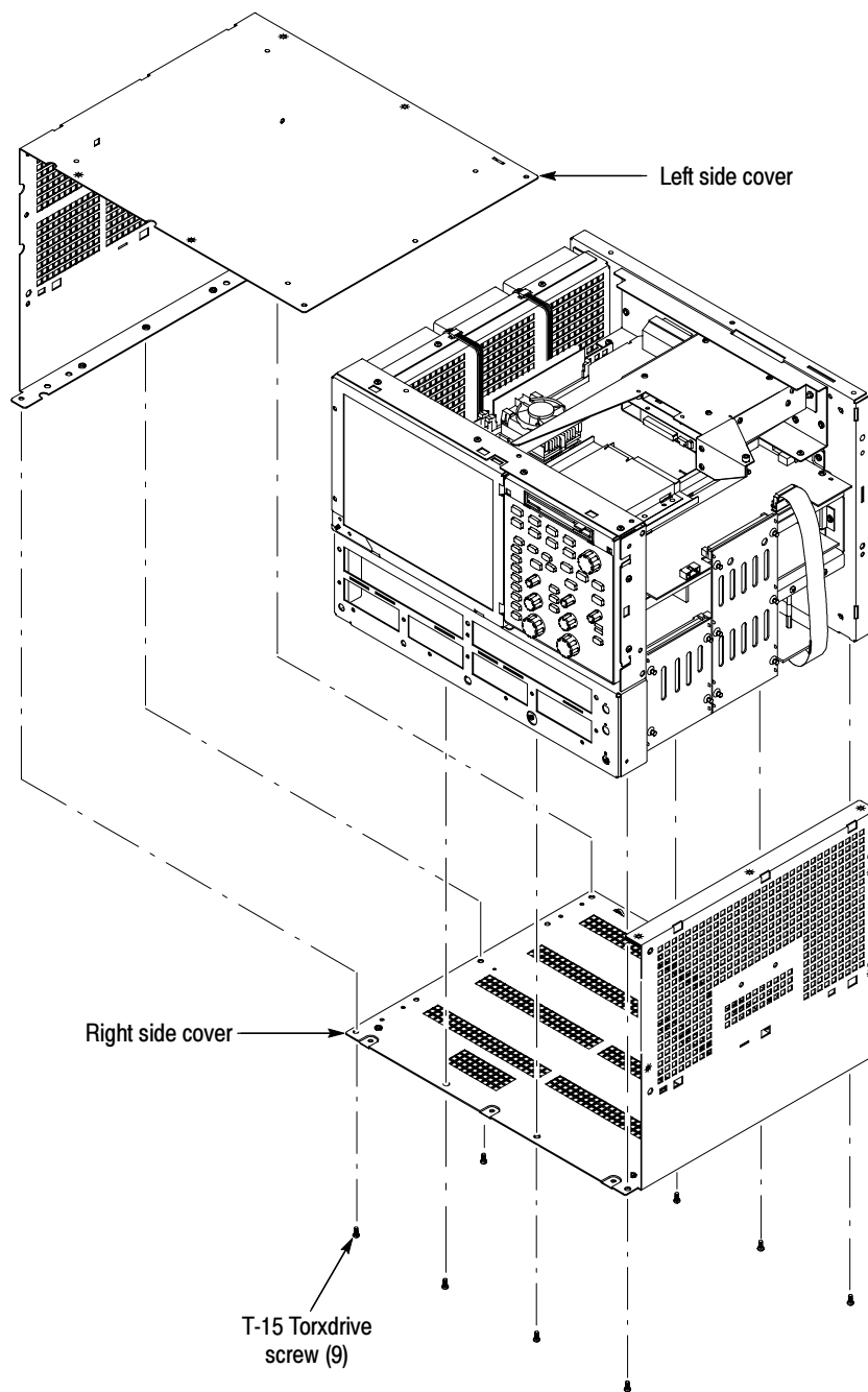
Figure 6-5: Cover removal
