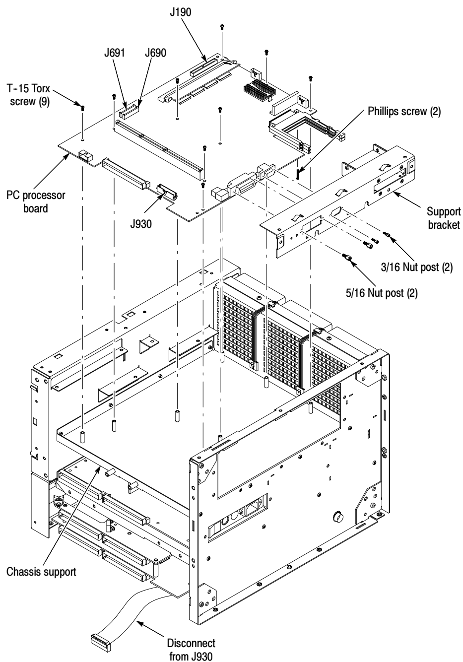
Figure 6-28: Processor board removal
