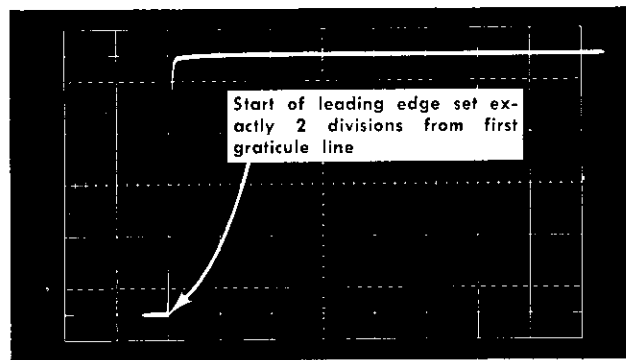
(A) Deflection factor 1 V/div (including Dual Attenuator Head); sweep rate 0.1 \mu s/div
