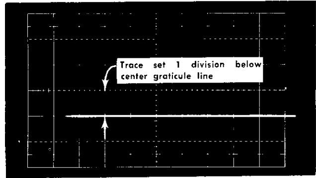
(B) Deflection factor 20 mV/div; sweep rate 0.1 \mu s/div
