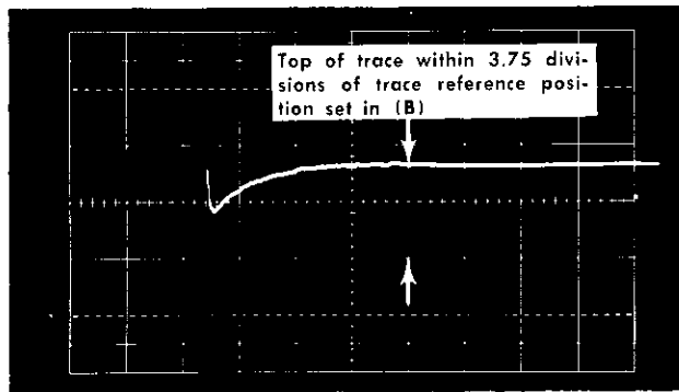
(C) Deflection factor 20 mV/div; sweep rate 0.1 \mu s/div
