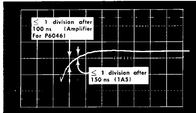
(E) Deflection factor 10 mV/div; sweep rate 0.1 \mu s/div
