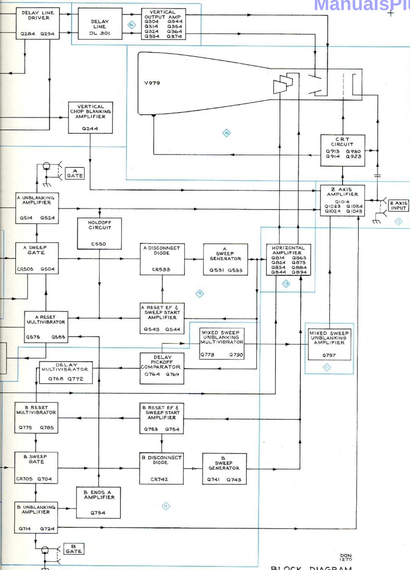
BLOCK DIAGRAM
