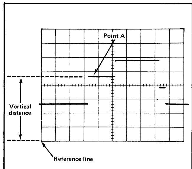
Fig. 2-18. Measuring instantaneous DC voltage with respect to a reference.
