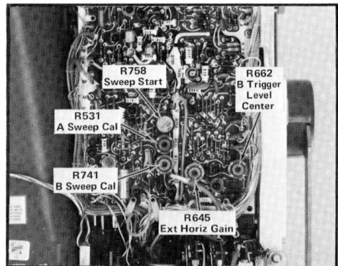
Fig. 5-13. Location of B Triggering and B Sweep Adjustments (B Sweep board).
