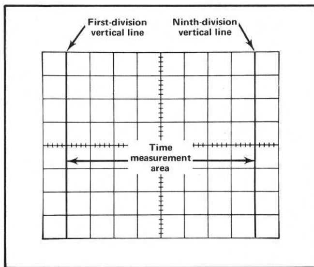
Fig. 2-11. Area of graticule used for accurate time measurements.
