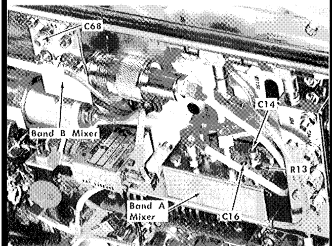
B. Band A and B mixer adjustment.
