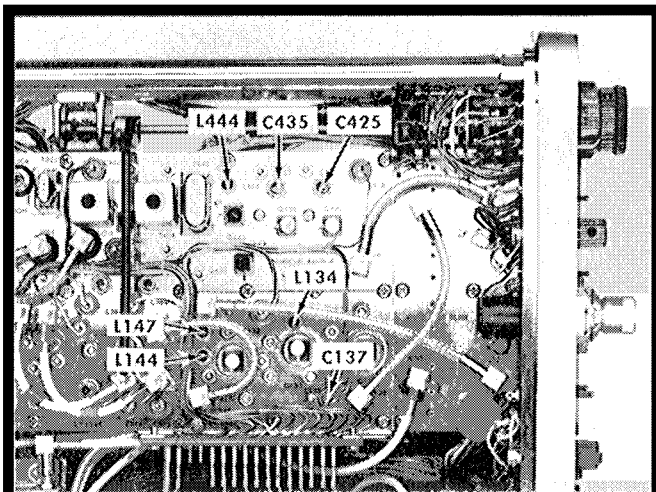
A. Wide band IF amplifier adjustments.
