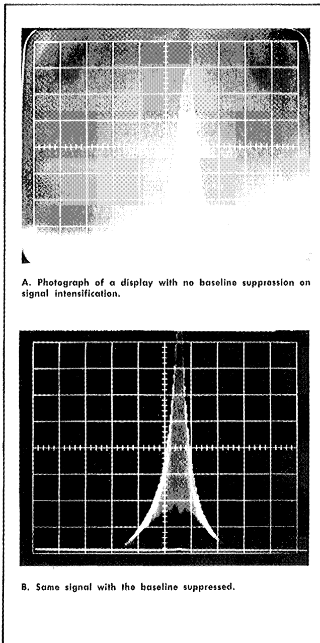
Fig. 2-6. INTENSIFIER operation.
