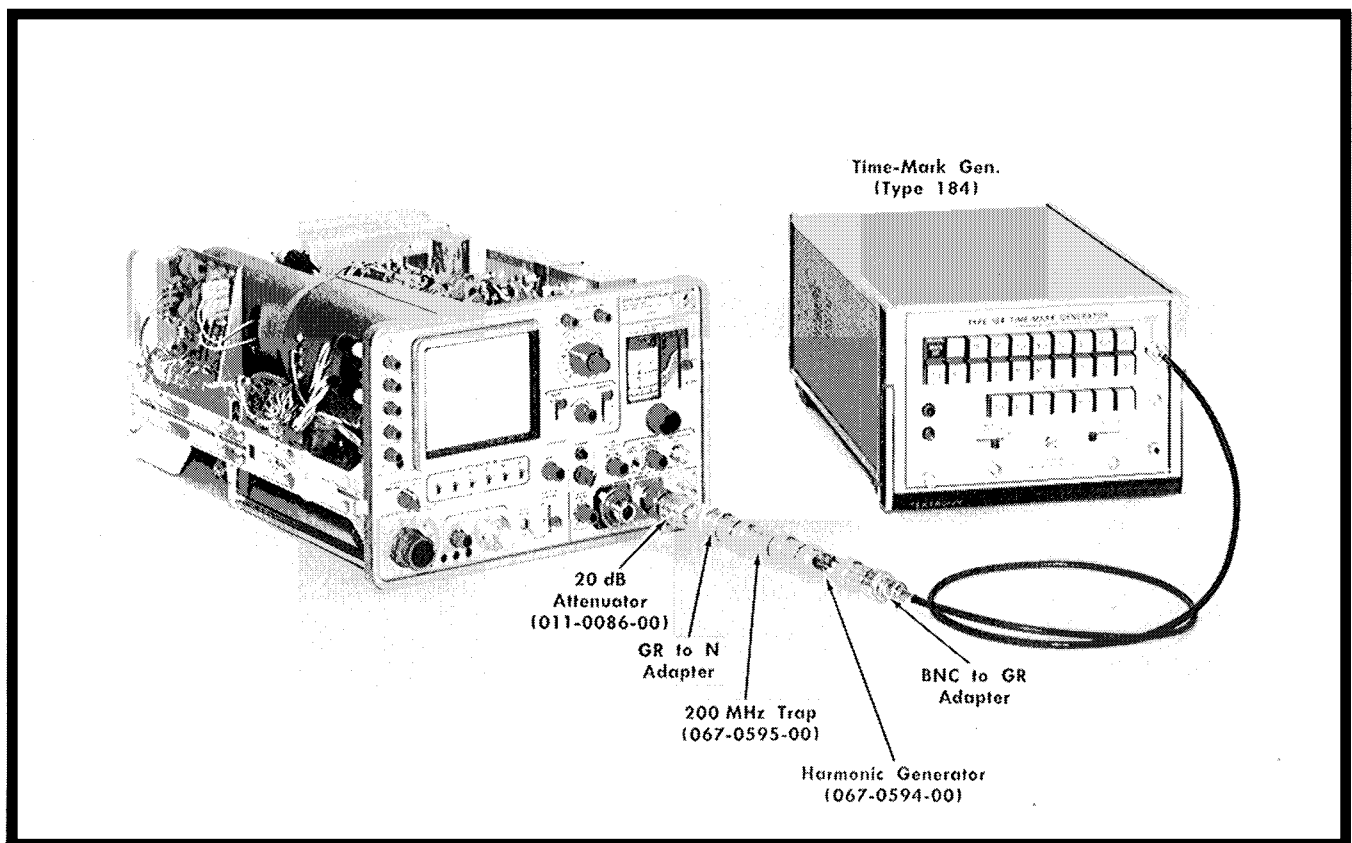
Fig. 6-45. Alternate equipment setup that will check dial accuracy, mixer and oscillator operation, and LO phase lock effectiveness.
