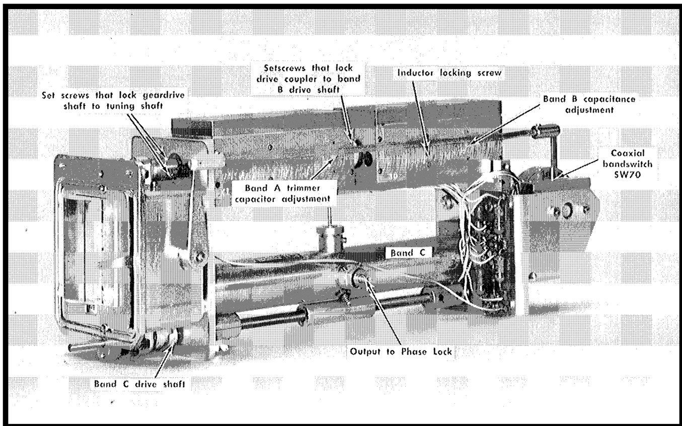
Fig. 6-48. Local oscillator assembly showing drive shaft coupling and tuning adjustments.
