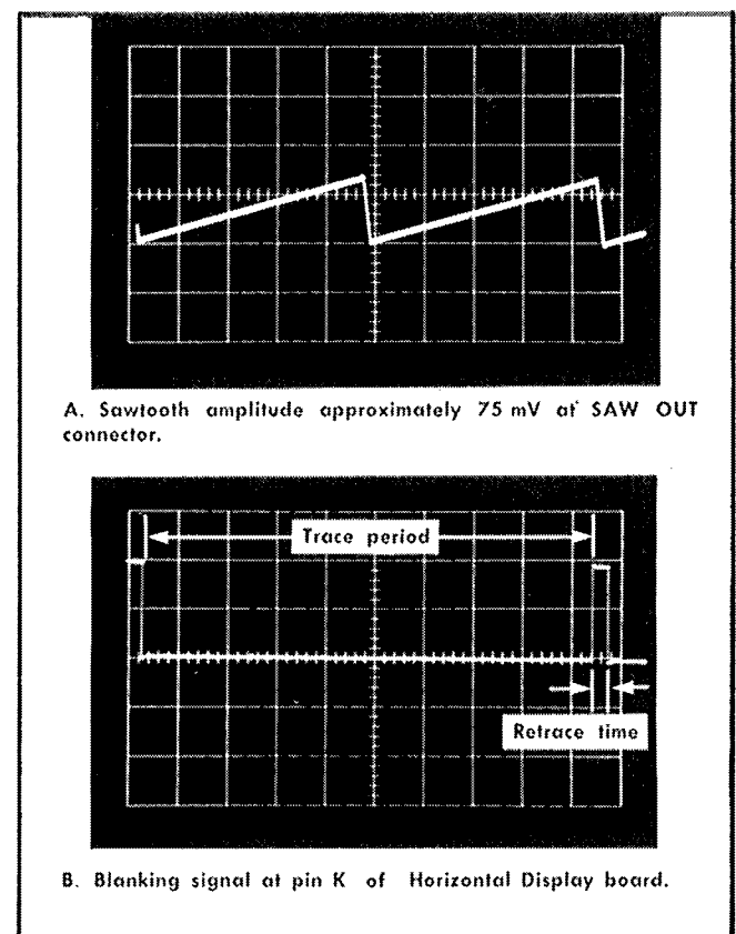
Fig. 6-16. Sawtooth waveform and blanking waveform.
