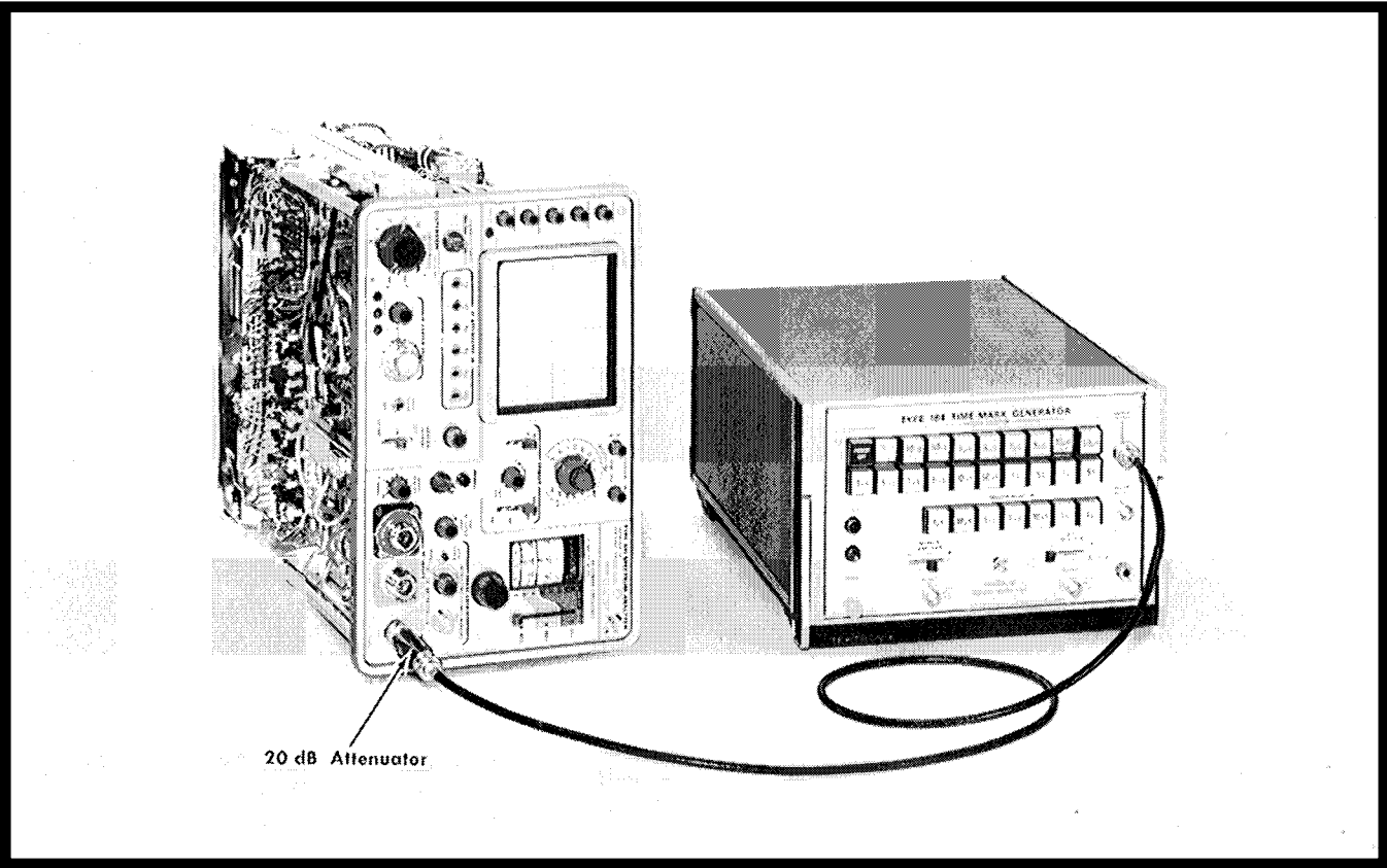
Fig. 6-29. Test equipment setup to adjust and check kHz/DIV dispersion accuracy.
