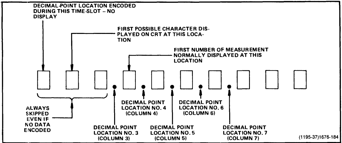
Fig. 3-35. Readout word relating 10 possible character locations to the decimal point instructions that can be encoded, and the resultant crt display.
