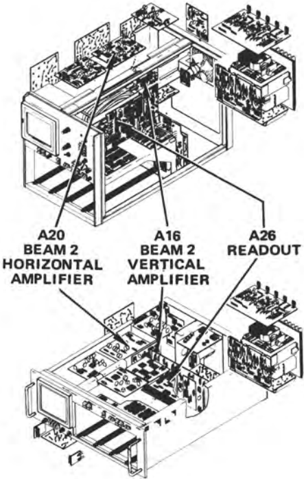
Fig. 9-48. A26—Location of Readout Mode Switch and adjustments.
