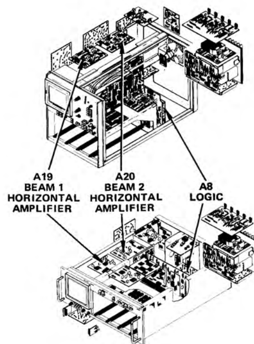
Fig. 9-33. A8—Location of Y-Axis Alignment adjustment.
