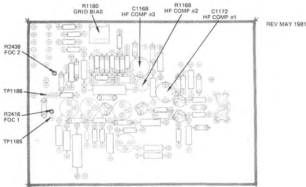
Fig. 9-30. A21—Location of Beam 1 Z-Axis test points and adjustments.
