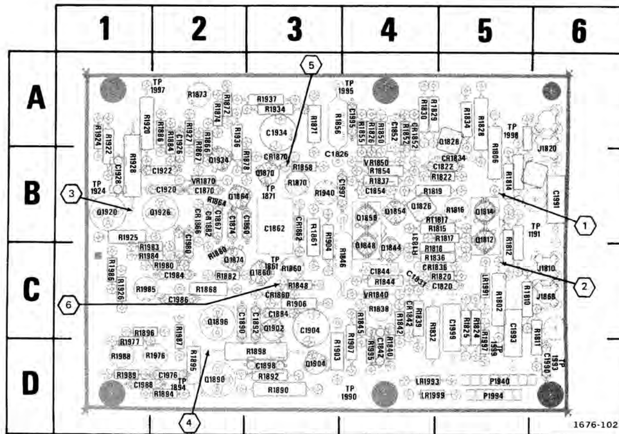
Fig. 9-14B. A19—Horizontal Amplifier circuit board assembly, Beam 1. (For instruments 7844 SN B109999-below; R7844 SN B099999-below).
