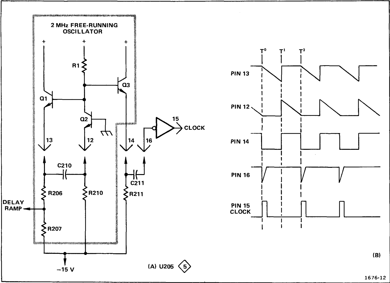
Fig. 3-6. (A) Diagram of Clock Generator stage; (B) Idealized waveforms for Clock Generator stage.
