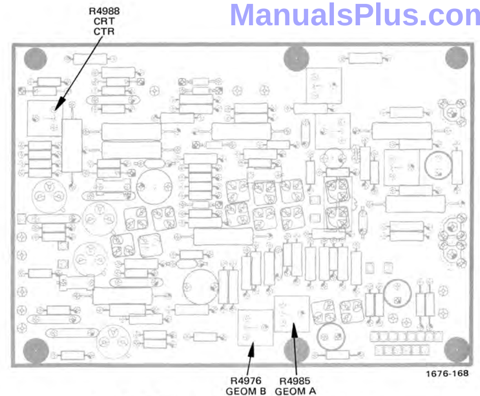
Fig. 9-34. A19—Location of Beam 1 Geometry adjustments. (7844 SN B110000 & up) (7844 SN B100000 & up)
