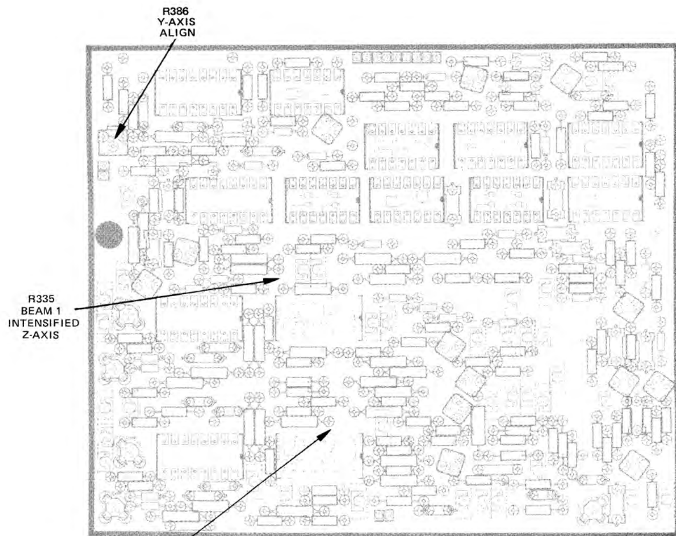
Fig. 9-33. A8—Location of Y-Axis Alignment adjustment.
