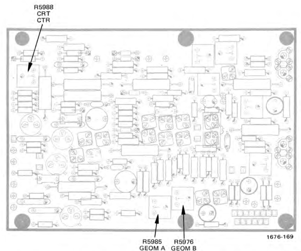
Fig. 9-35. A20—Location of Beam 2 Geometry adjustments. (7844 SN B110000 & up) (7844 SN B100000 & up)
