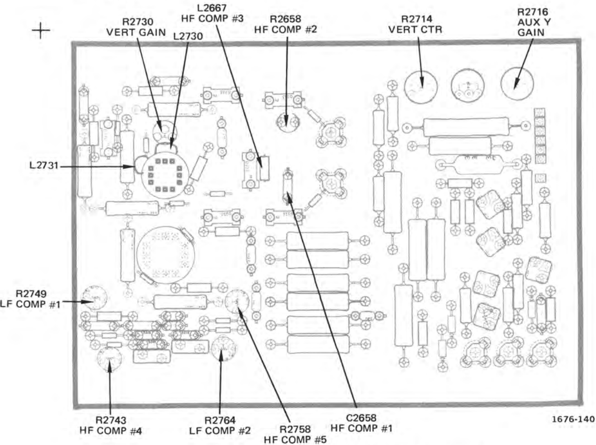
Fig. 9-46. A16—Location of Beam 2 Vertical adjustments.
