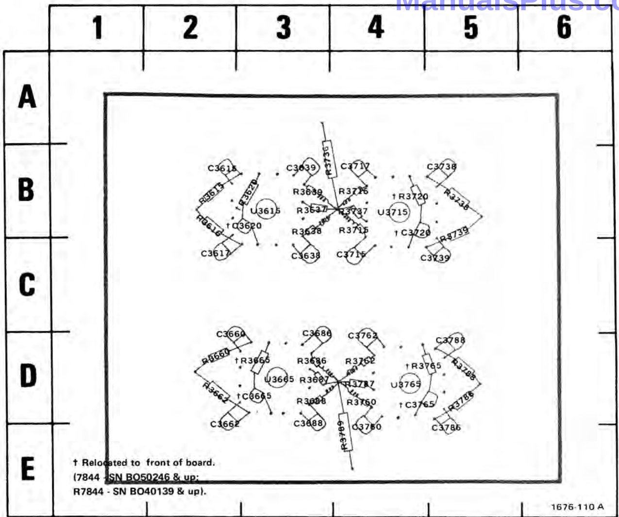
Fig. 9-9C. A10—Crossover Vertical Interface circuit board assembly (rear).
