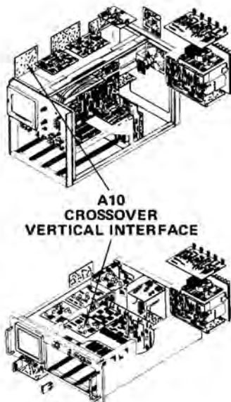
Fig. 9-9C. A10—Crossover Vertical Interface circuit board assembly (rear).
