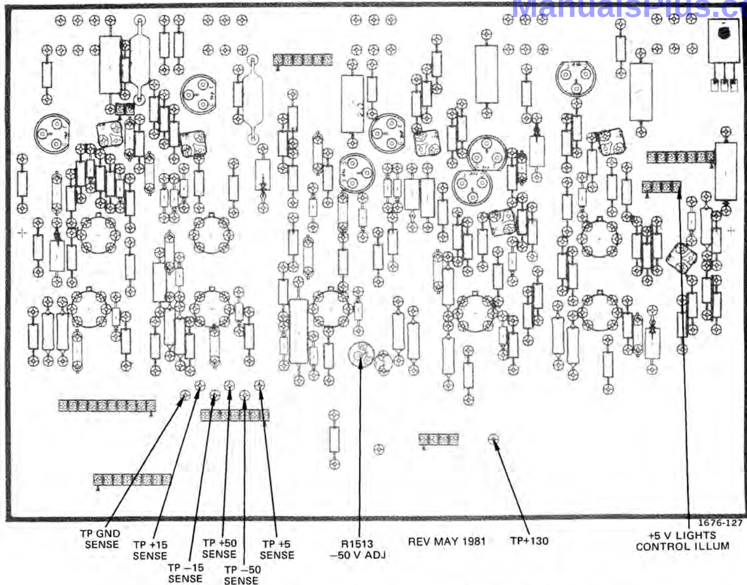
Fig. 9-28. A29—Location of Low-Voltage power supply test points and adjustments.
