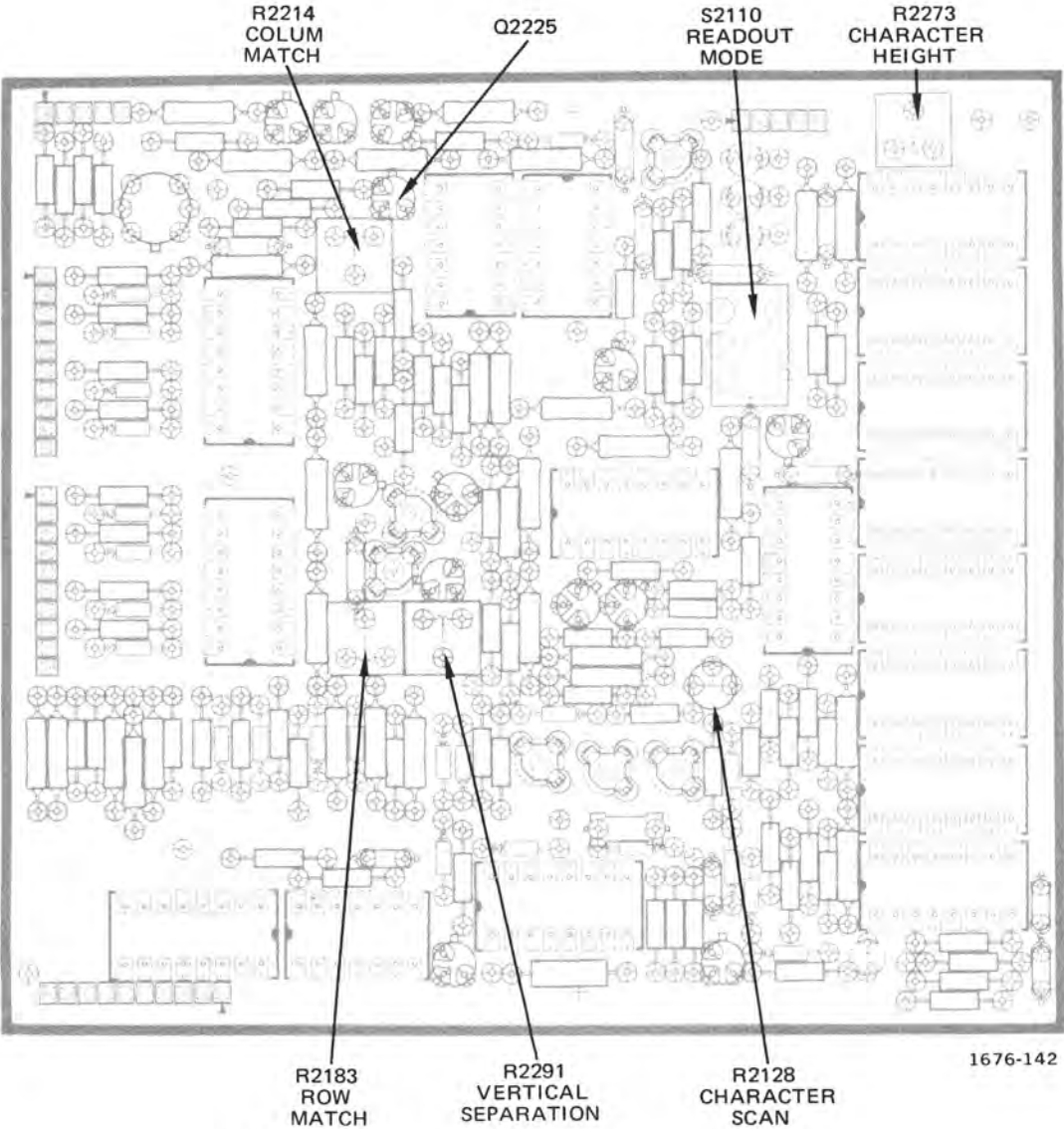
Fig. 9-48. A26—Location of Readout Mode Switch and adjustments.
