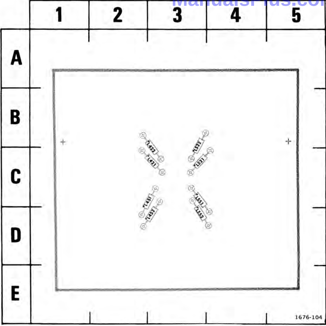
Fig. 9-8B. A9—Trigger Selector circuit board assembly (rear).
