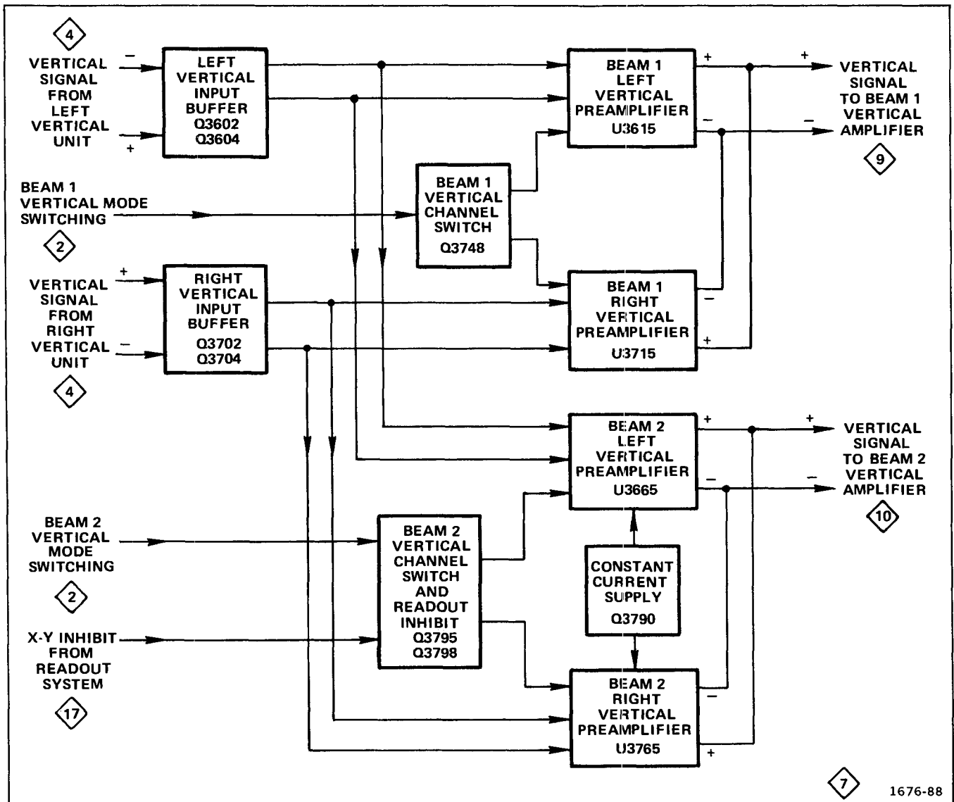
Fig. 3-14. Detailed block diagram of the Crossover Vertical Interface circuit.
