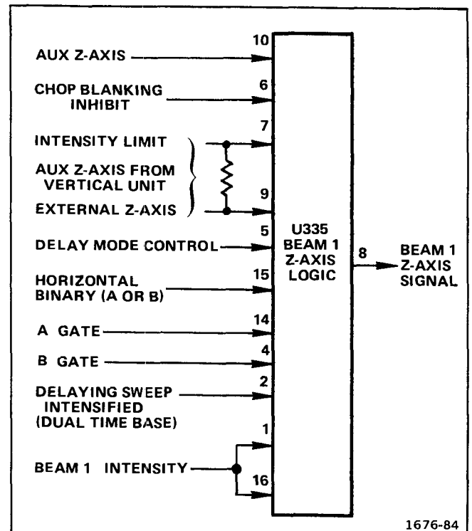
Fig. 3-11. Functional diagram of Beam 1 Z-Axis Logic (U335).
