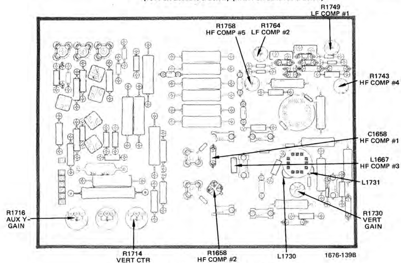
Fig. 9-45. A13—Location of Beam 1 Vertical adjustments.
