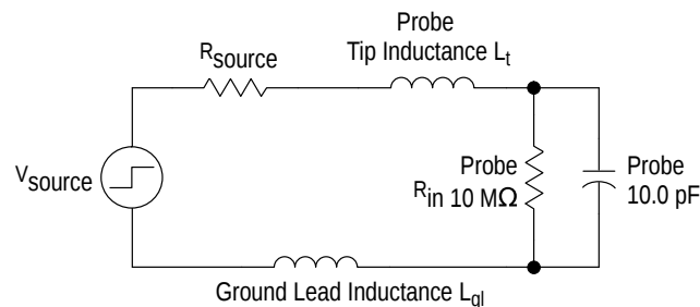
Figure 3–33: A Probe Adds Resistance, Capacitance, and Inductance
