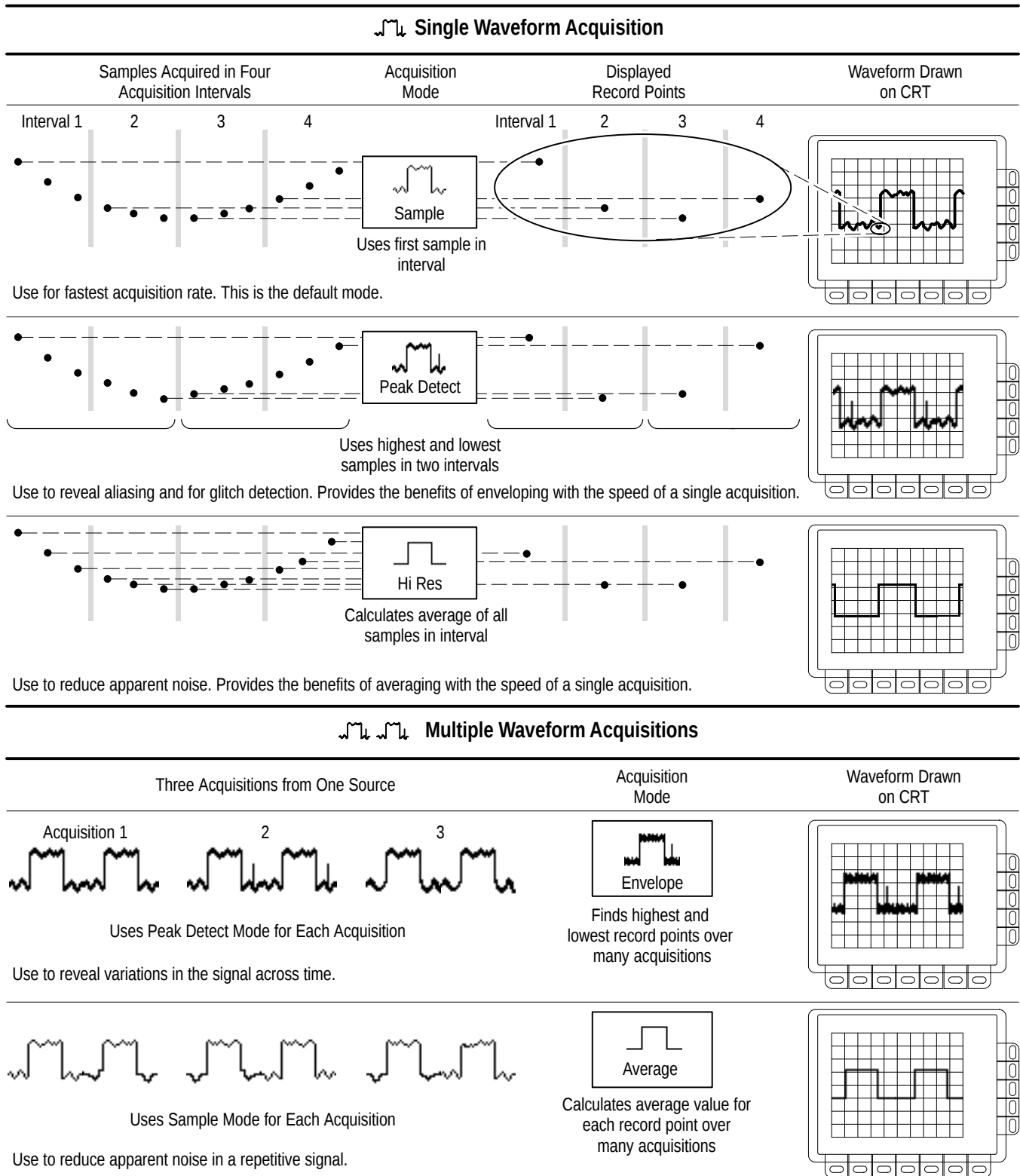
Figure 3-2: How the Acquisition Modes Work
