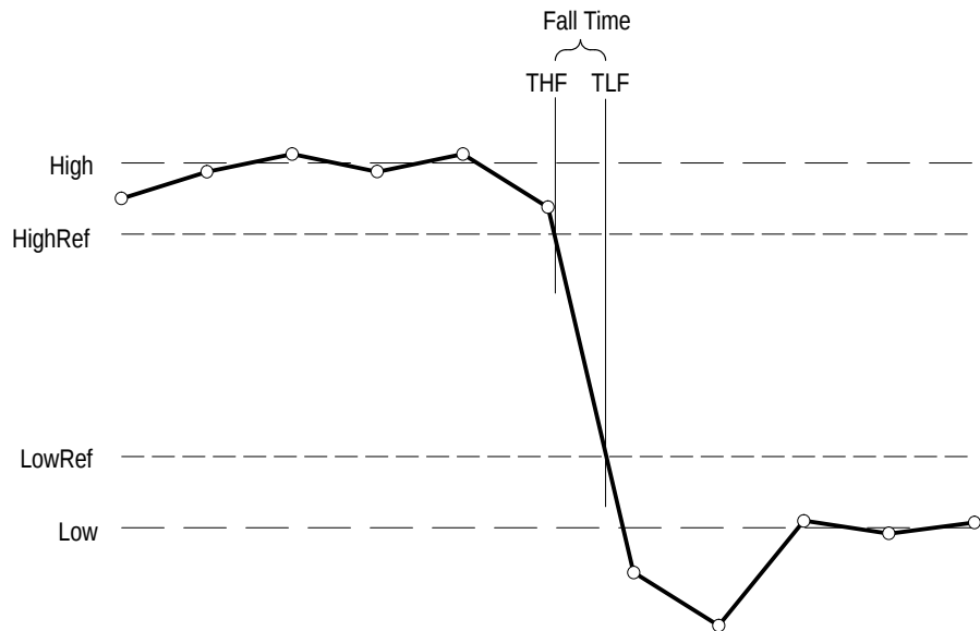
Figure C-2: Fall Time
