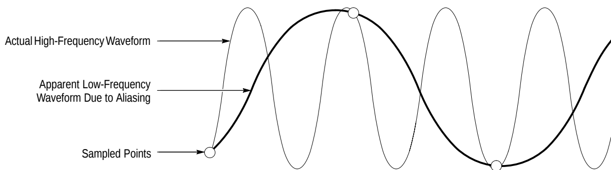
Figure 2–30: Aliasing
