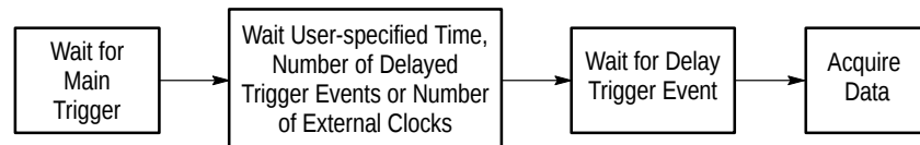
Figure 3–6: Delayed Triggerable
