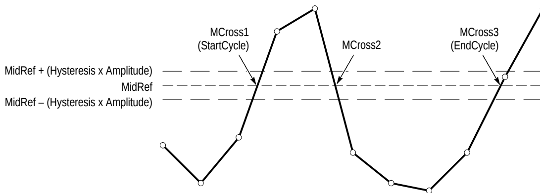
Figure C-1: MCross Calculations
