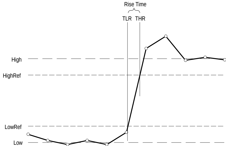
Figure C-3: Rise Time
