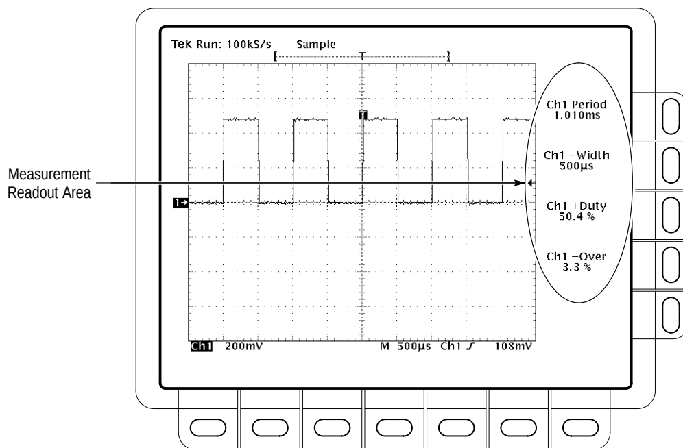
Figure 3-27: Measurement Readouts
