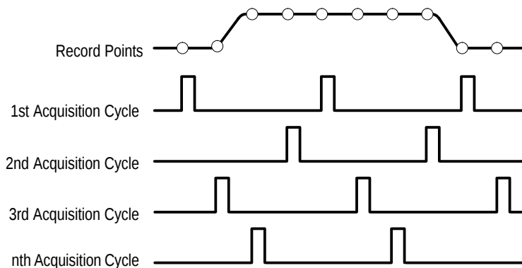
Figure 2-28: Equivalent-Time Sampling
