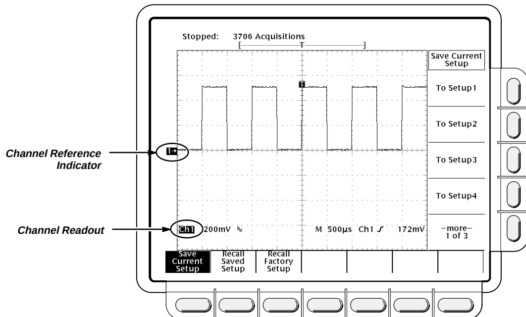
Figure 3-55: The Channel Readout
