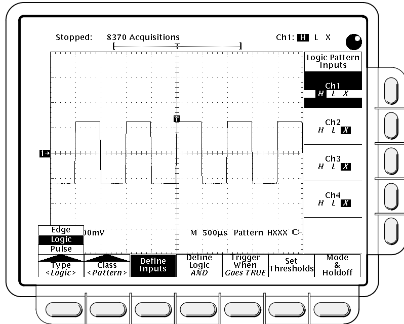
Figure 3-27: Logic Trigger Menu
