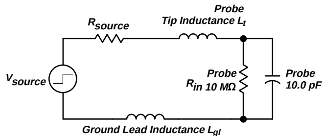
Figure 3-35: A Probe Adds Resistance, Capacitance, and Inductance
