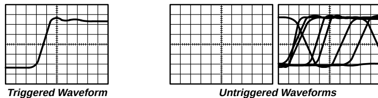
Figure 2-1: Triggered Versus Untriggered Displays
