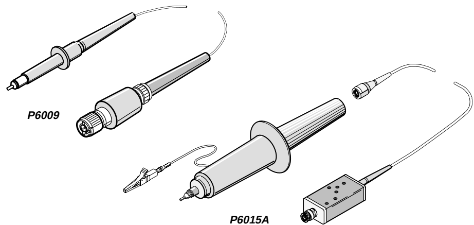
Figure 3-43: The P6009 and P6015A High Voltage Probes
