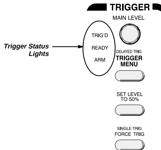
Figure 3-59: TRIGGER Controls and Status Lights
