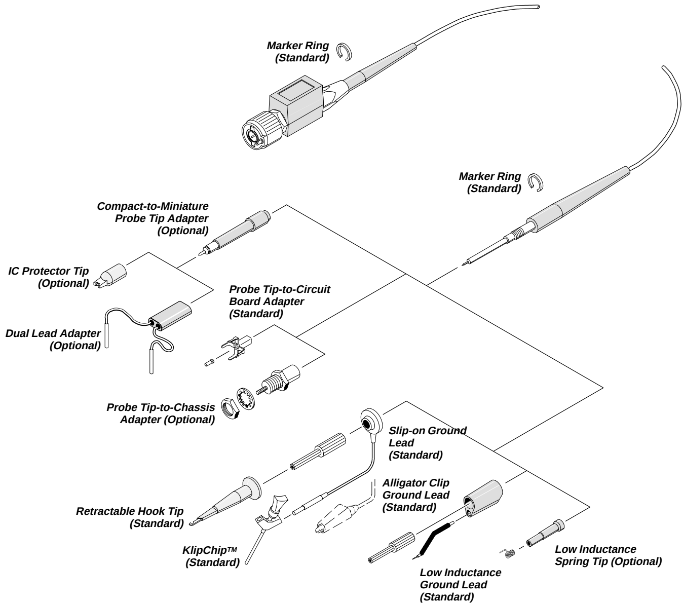
Figure 3-37: Probe Accessories
