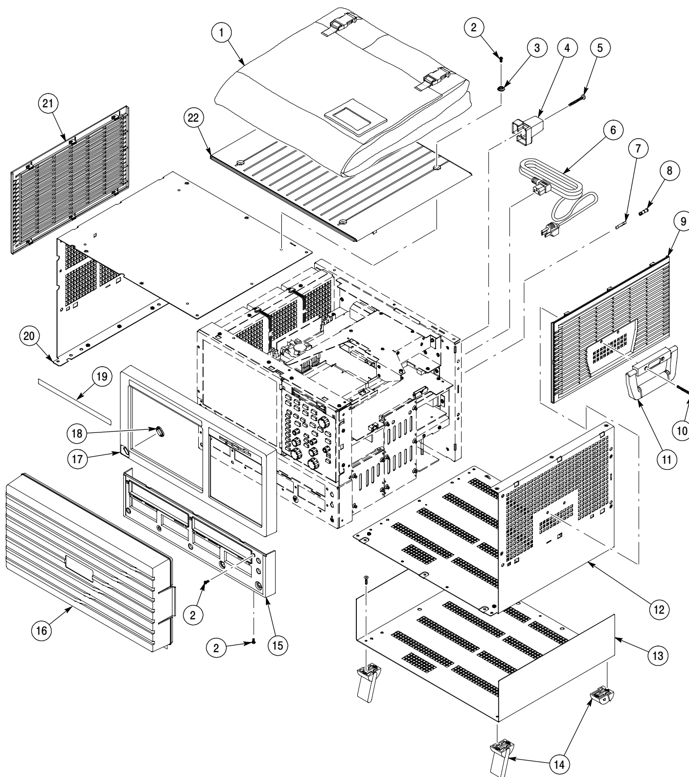
Figure 10-1: External parts
