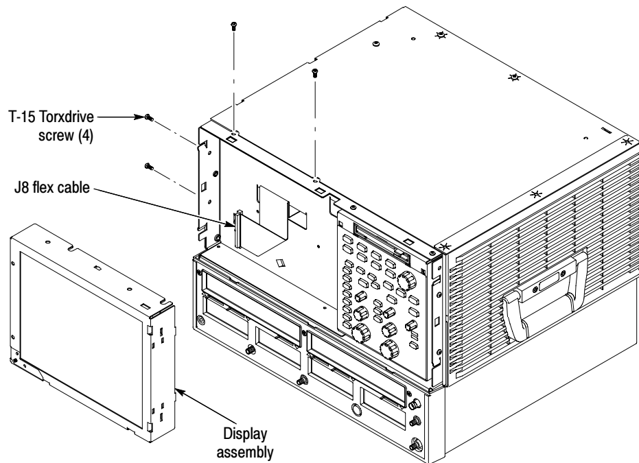
Figure 6-13: Display removal
