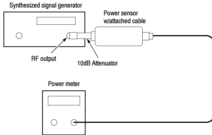
Figure 4- 26: Power-reference hookup
