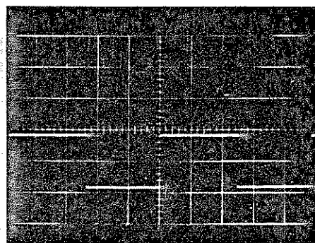
18- A8Q4 Collector FREQUENCY - 1 kc 5 V/CM; .2 \mu SEC/CM
