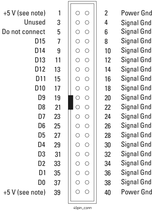
40-pin Connector Pinout
