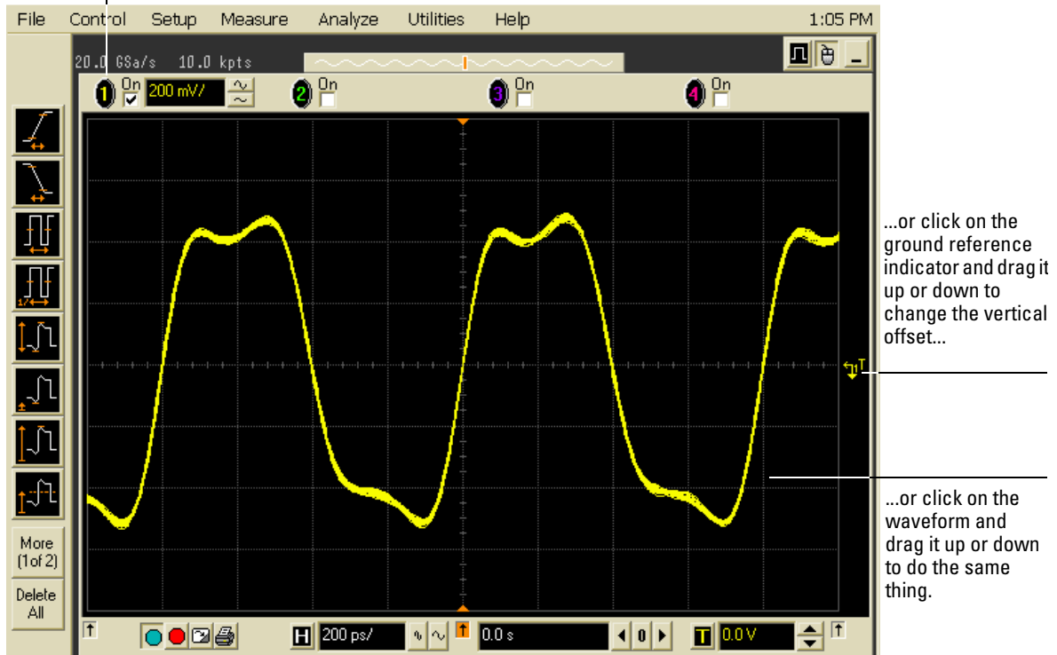
Adjusting Vertical Offset
