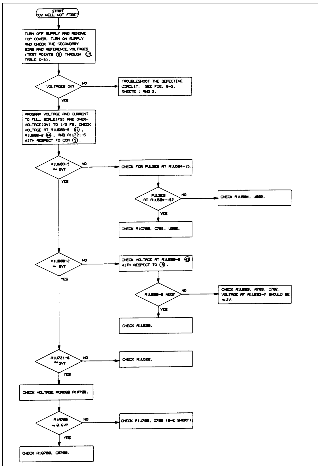
Figure 3-6. OV Will Not Fire Troubleshooting
