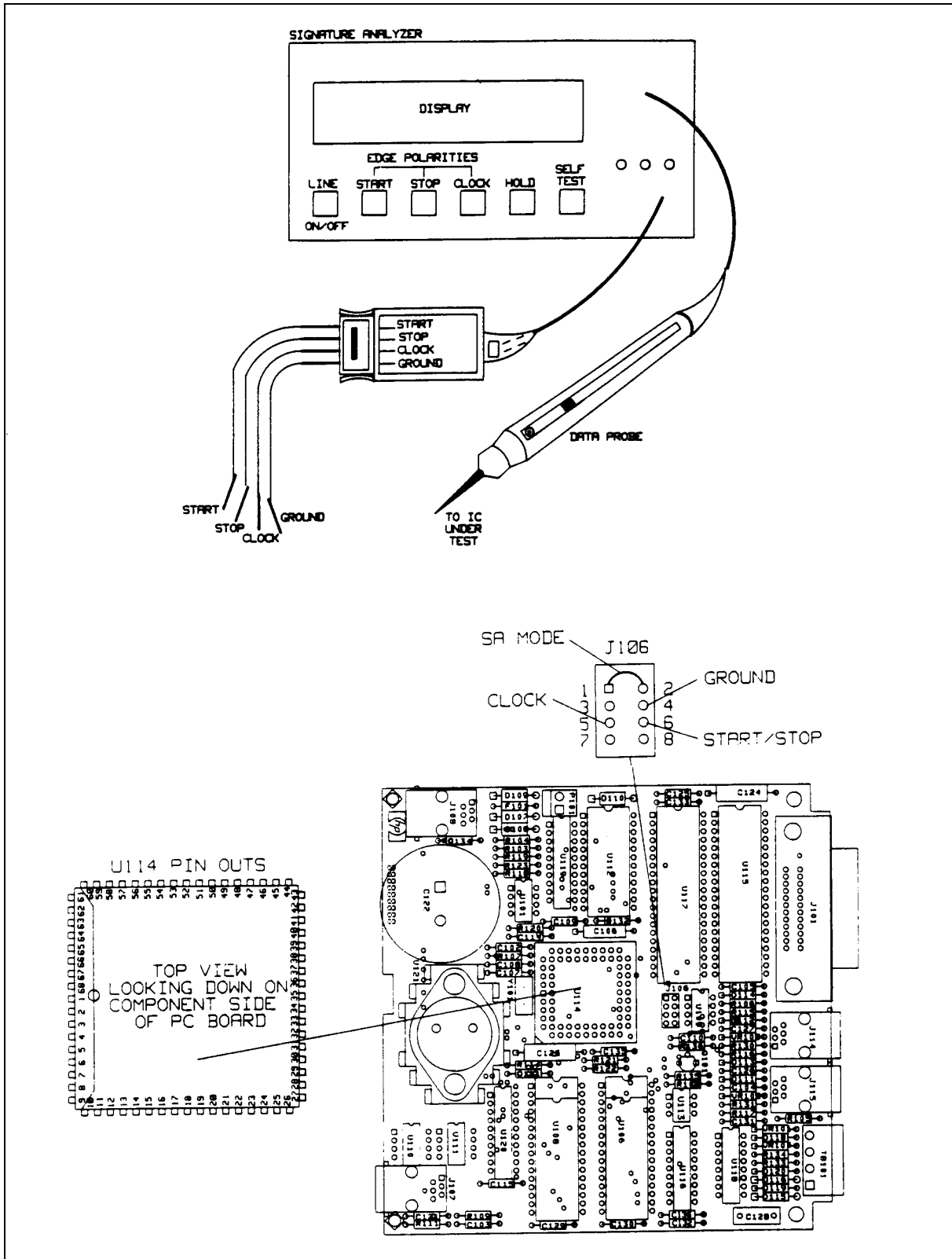
Figure 3-4. Connections For A2 GPIB Board Models 664xA &amp; 665xA Only (Sheet 1 of 3)
