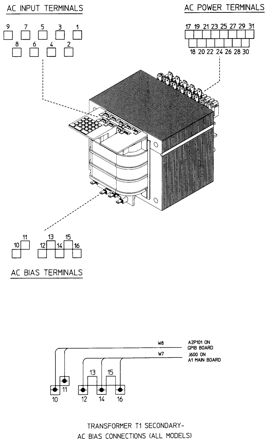
Figure 6-9. Power Transformer Wiring Diagram for Models 655xA and 665xA (Sheet 1 of 3)
