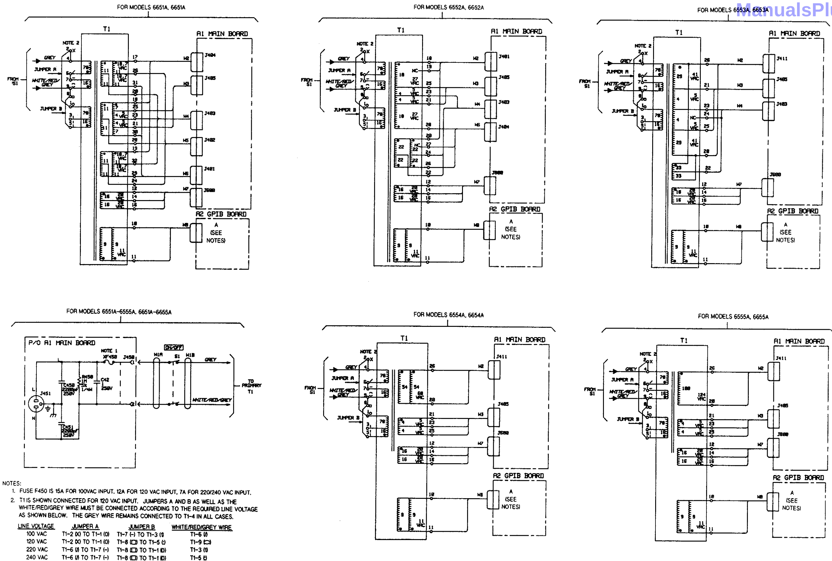
Figure 6-2. AC Power Distribution Diagram for 655xA &amp; 665xA Models
