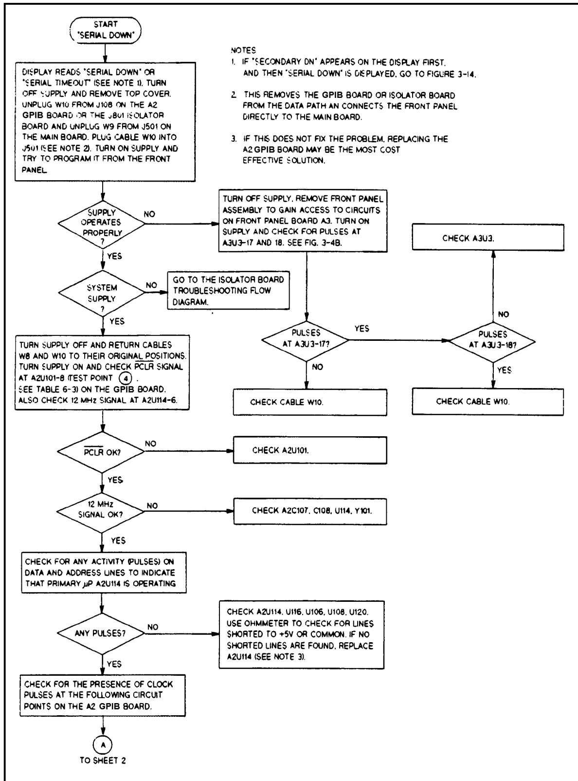
Figure 3-13. Serial Down Troubleshooting (Sheet 1 of 2)
