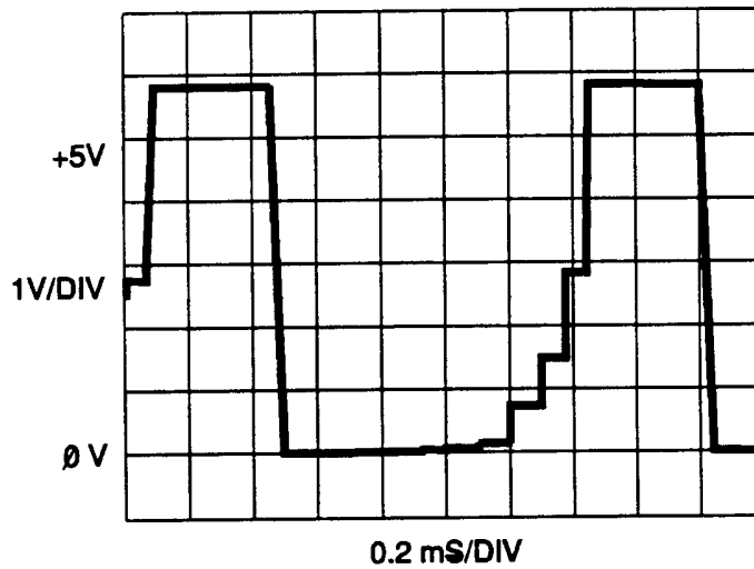
B. READBACK DAC (U512-6) OUTPUT
