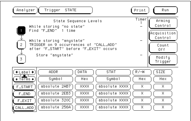
Triggering on the 10th call of a recursive function
