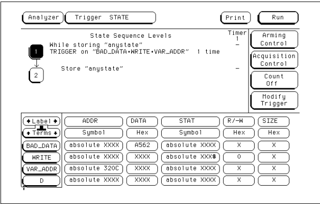
Capturing a bad write to a variable
