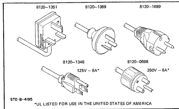
Figure 2-1. Power Receptacles.
