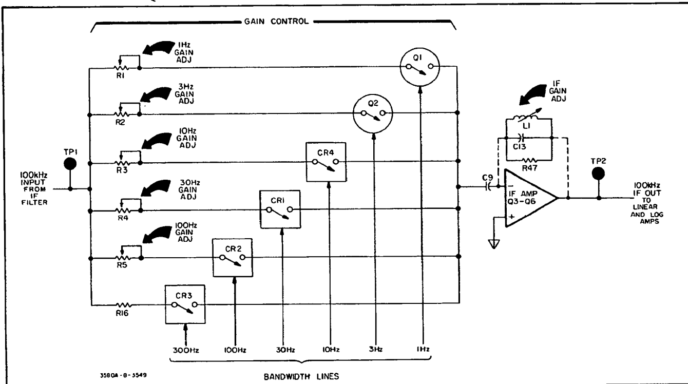
Figure 4-4. IF Amplifier.
