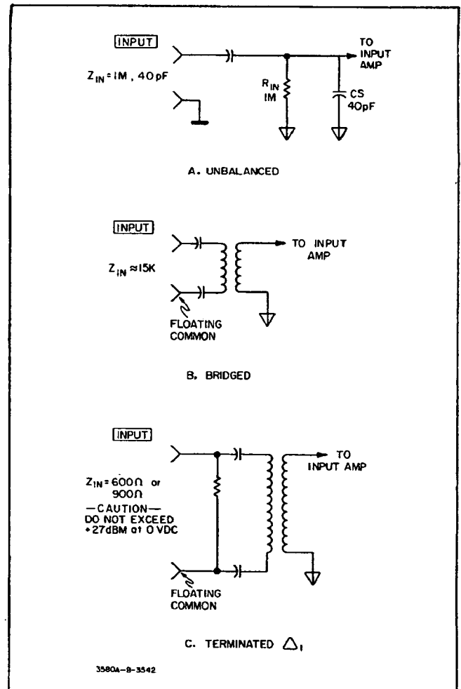
Figure 3-32. Input Configurations (Option 002).
