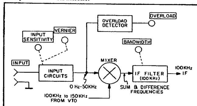
Figure 3-13. Frequency Tuning.
