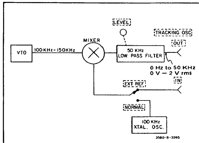
Figure 3-31. Tracking Oscillator.
