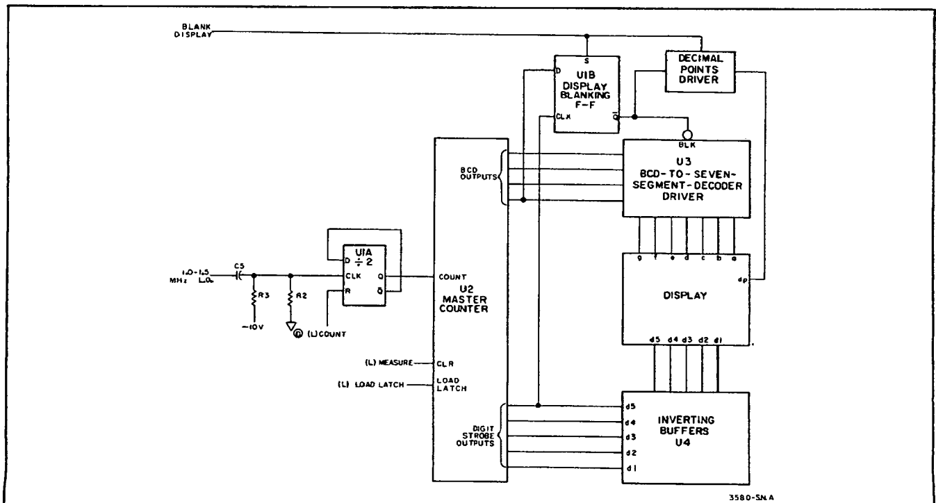
Figure 4-28. Counter and Display.
