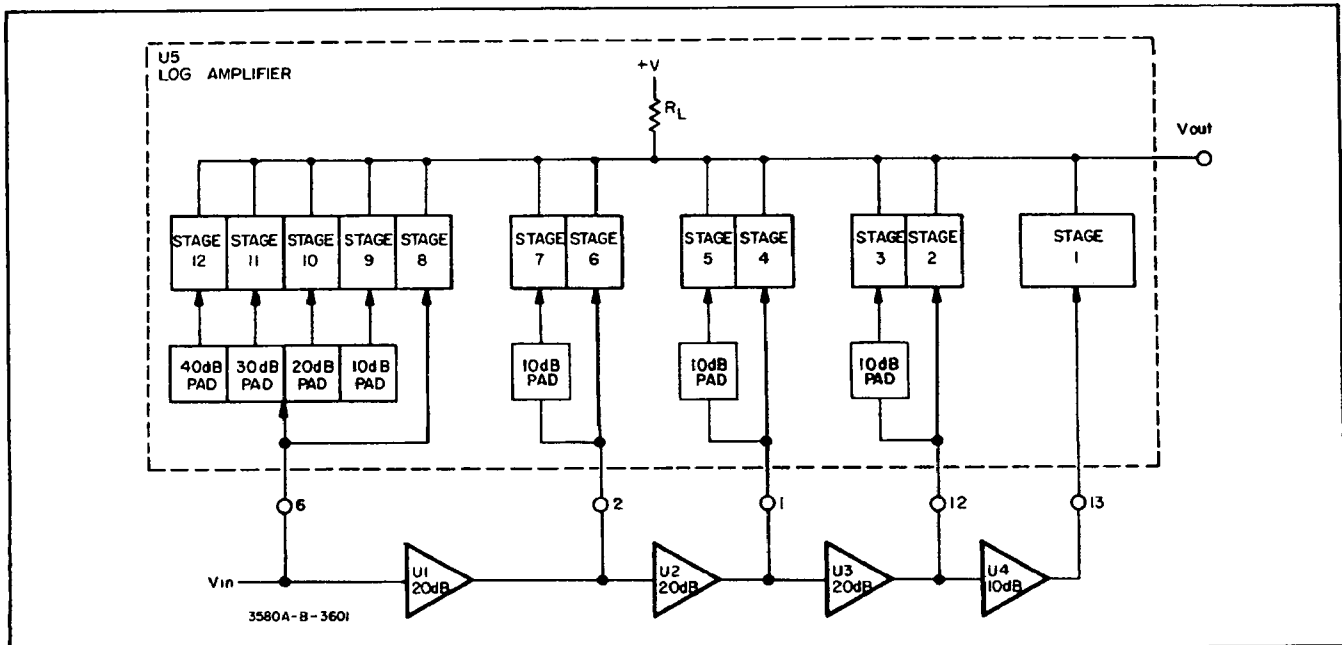
Figure 4-6. Log Amplifier.
