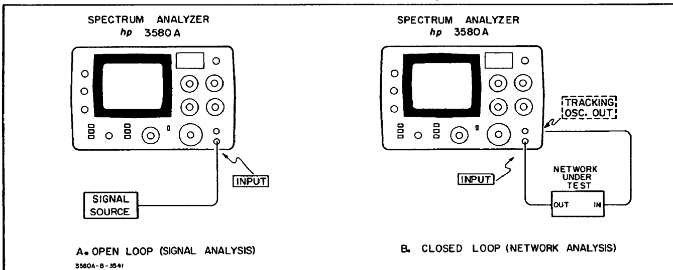
Figure 3-6. Measurement Configurations.
