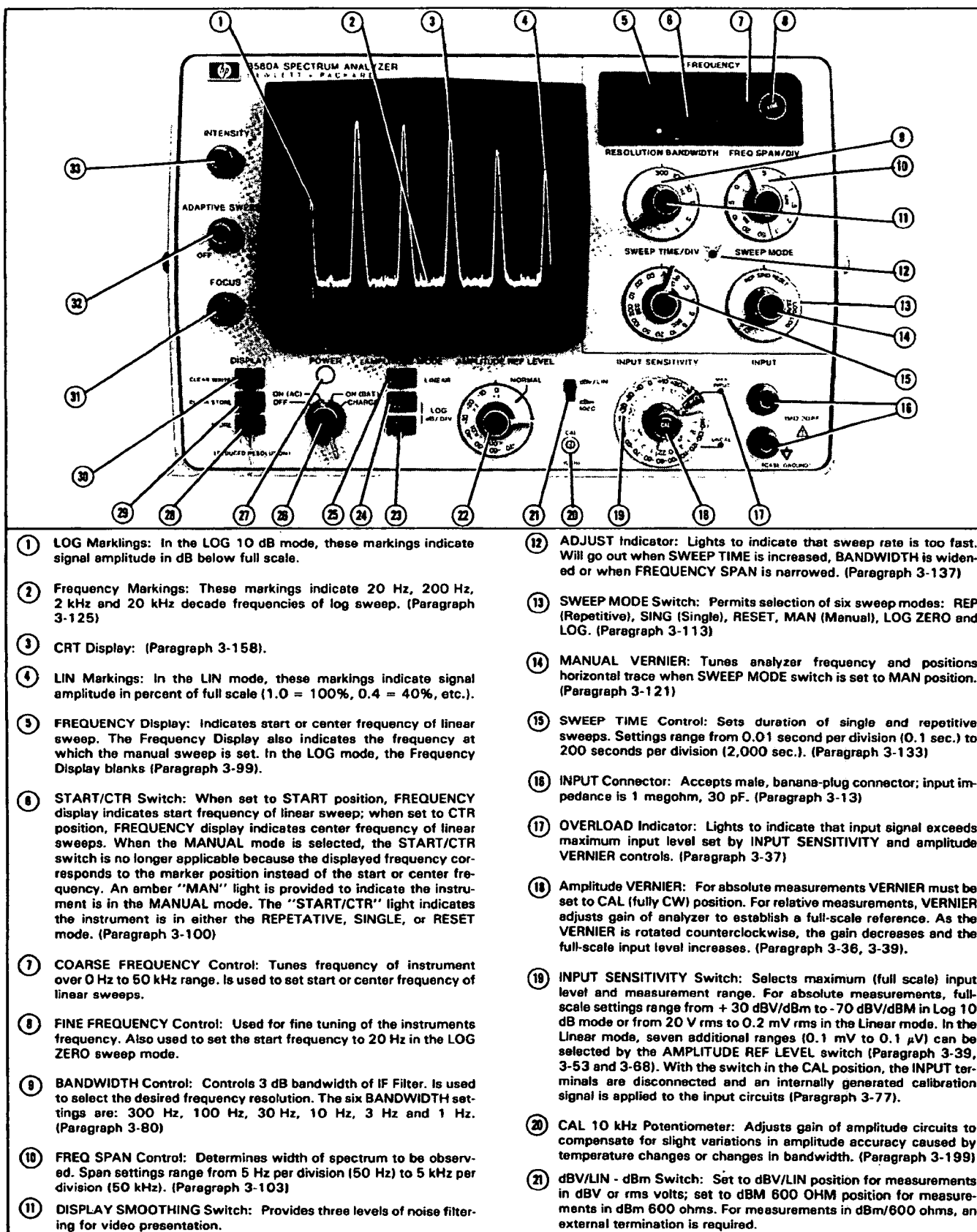
Figure 3-1. Front Panel.
