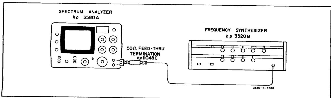
Figure 5-2. Proper Hookup.
