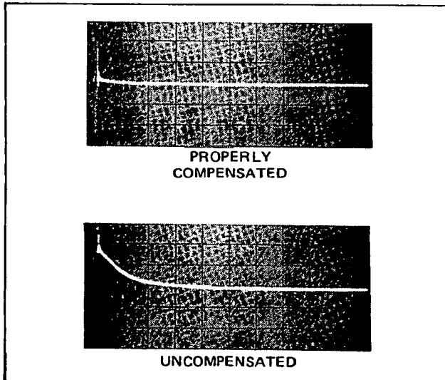
Figure 3-35. Probe Compensation.
