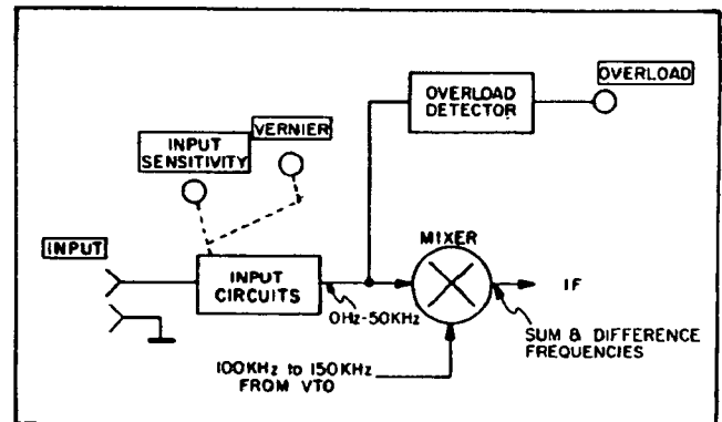
Figure 3-7. Input Section.
