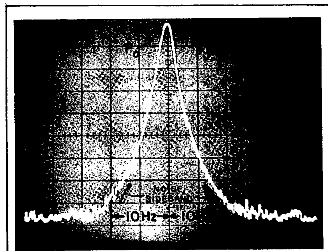
Figure 3-19. Noise Sidebands (1 Hz BW)
