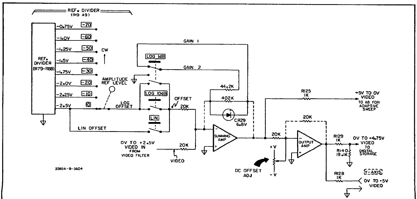
Figure 4-9. Video Output.
