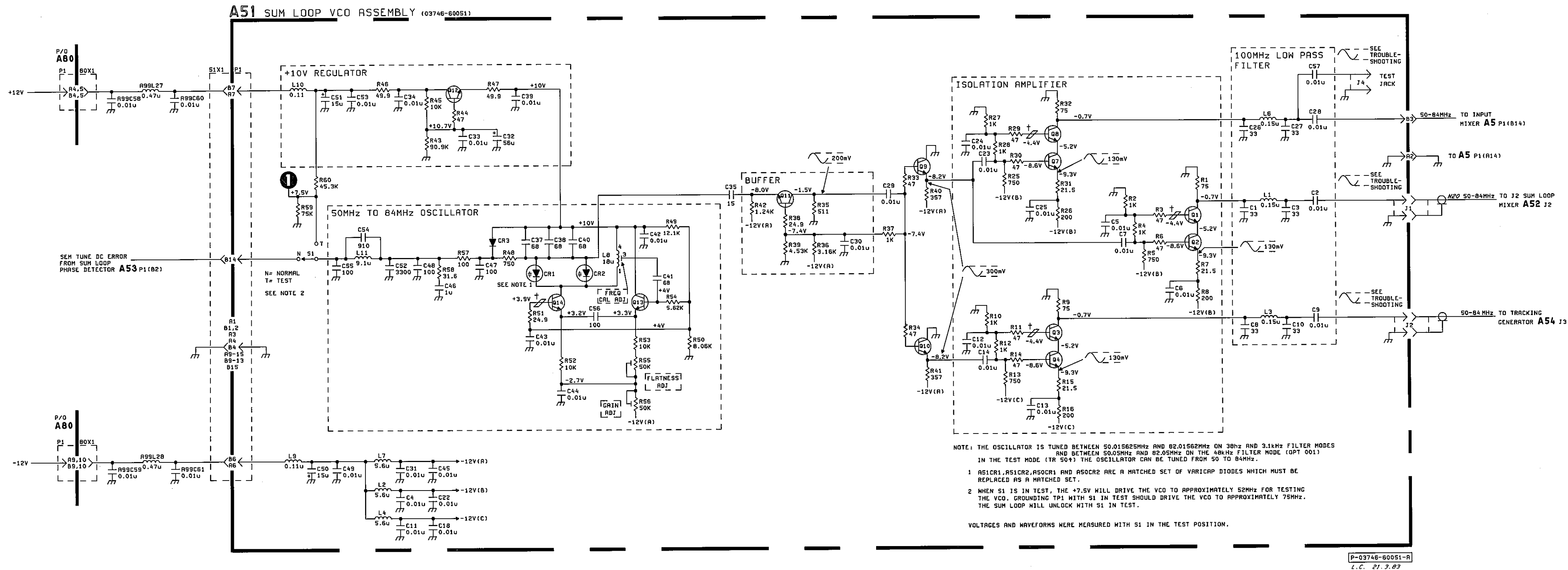
Figure A51-3 A51 Schematic Diagram
