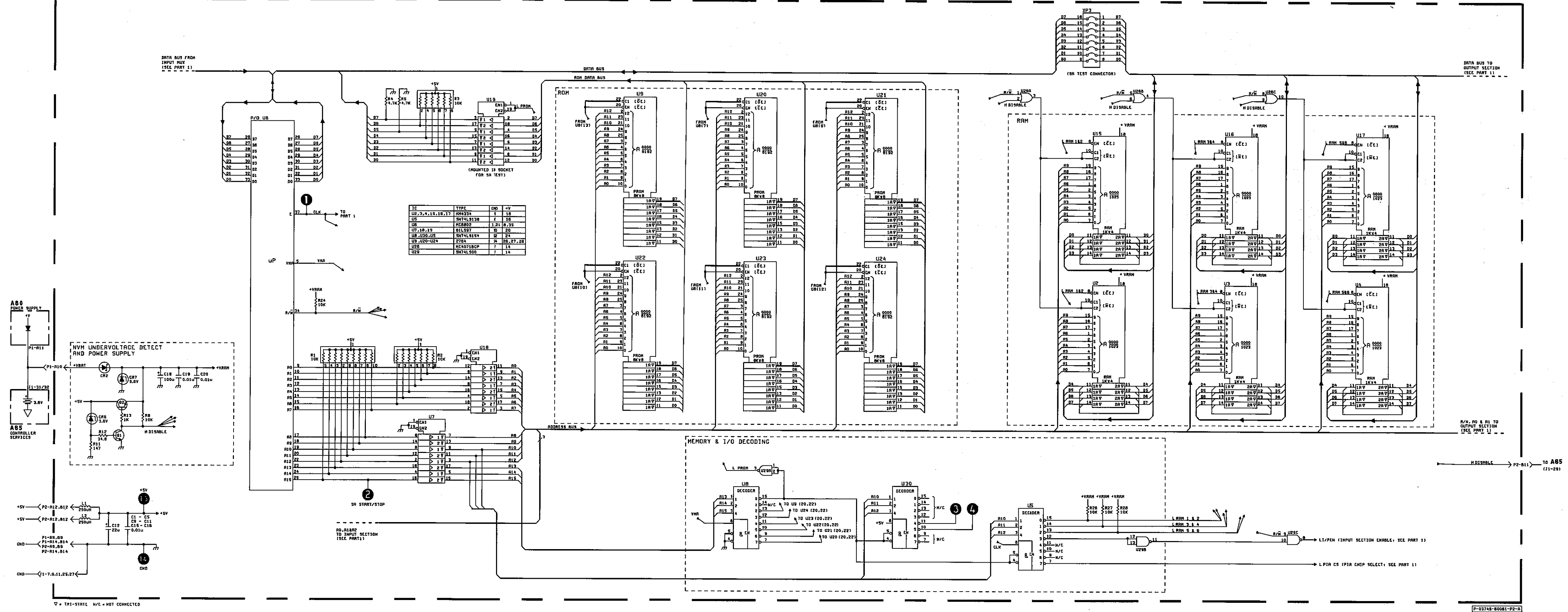
A60 CONTROLLER ASSEMBLY (03748-80081) PART 2
