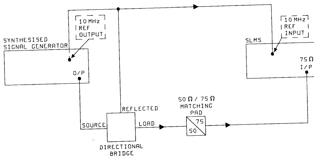
Figure 4-7 Intermodulation Test Setup
