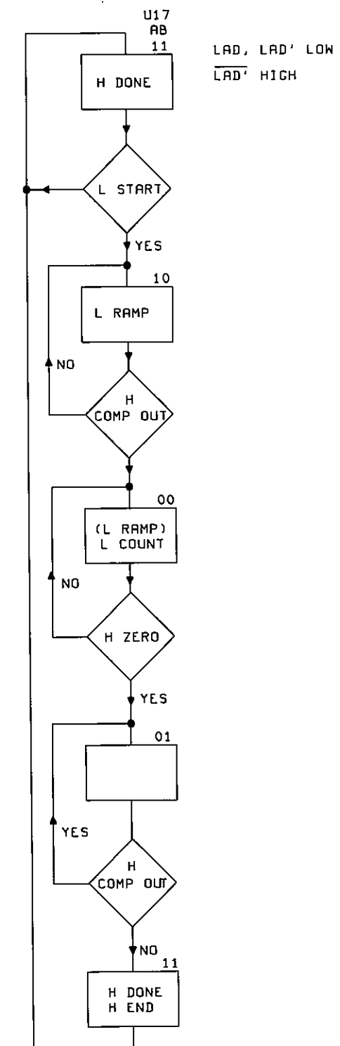
1. THE CONTROL LOGIC IS IN THE IDLE STATE. 2. THE PROCESSOR (ON ASSEMBLY A60) PULSES L START A/D LOW AND L START (AT U29B) GOES LOW TO RESET U17B. 3. U17B GOES LOW, FORCING L RAMP LOW, THE INTEGRATOR RAMP UP PERIOD BEGINS AND R22 C8 BEGINS TO CHARGE. 4. AS THE RAMP CROSSES THE THRESHOLD LEVEL OF THE COMPARITOR (IN U16) H COMP OUT GOES HIGH. 5. L COUNT GOES LOW AND SET INPUT (AT U23 PIN 2) OF THE COUNTER IS PULLED LOW (THIS BLANKS THE BCD OUTPUTS). ALSO THE COUNT INHIBIT AND COUNTER STORE LINES (U23 PIN 25, AND PIN 9) ARE PULLED LOW. THE COUNTER (U23) STARTS TO COUNT THE 500KHZ CLOCK PULSES. 6. THE COUNTER REACHES ZERO AND SETS H ZERO HIGH. 7. L RAMP GOES HIGH. THE INTEGRATOR NOW STARTS TO RAMP DOWN AS C8 DISCHARGES. 8. H COMP OUT GOES LOW AS THE RAMP CROSSES THE THRESHOLD LEVEL IN U16. 9. H END SWITCHES Q3 OFF. THE RAMP CONTROL VOLTAGE U16 (10) IS NOW DRIVEN BY THE VOLTAGE AT H COMP OUT TO MAINTAIN AN OSCILLATION ON THE RAMP CONTROL VOLTAGE.
