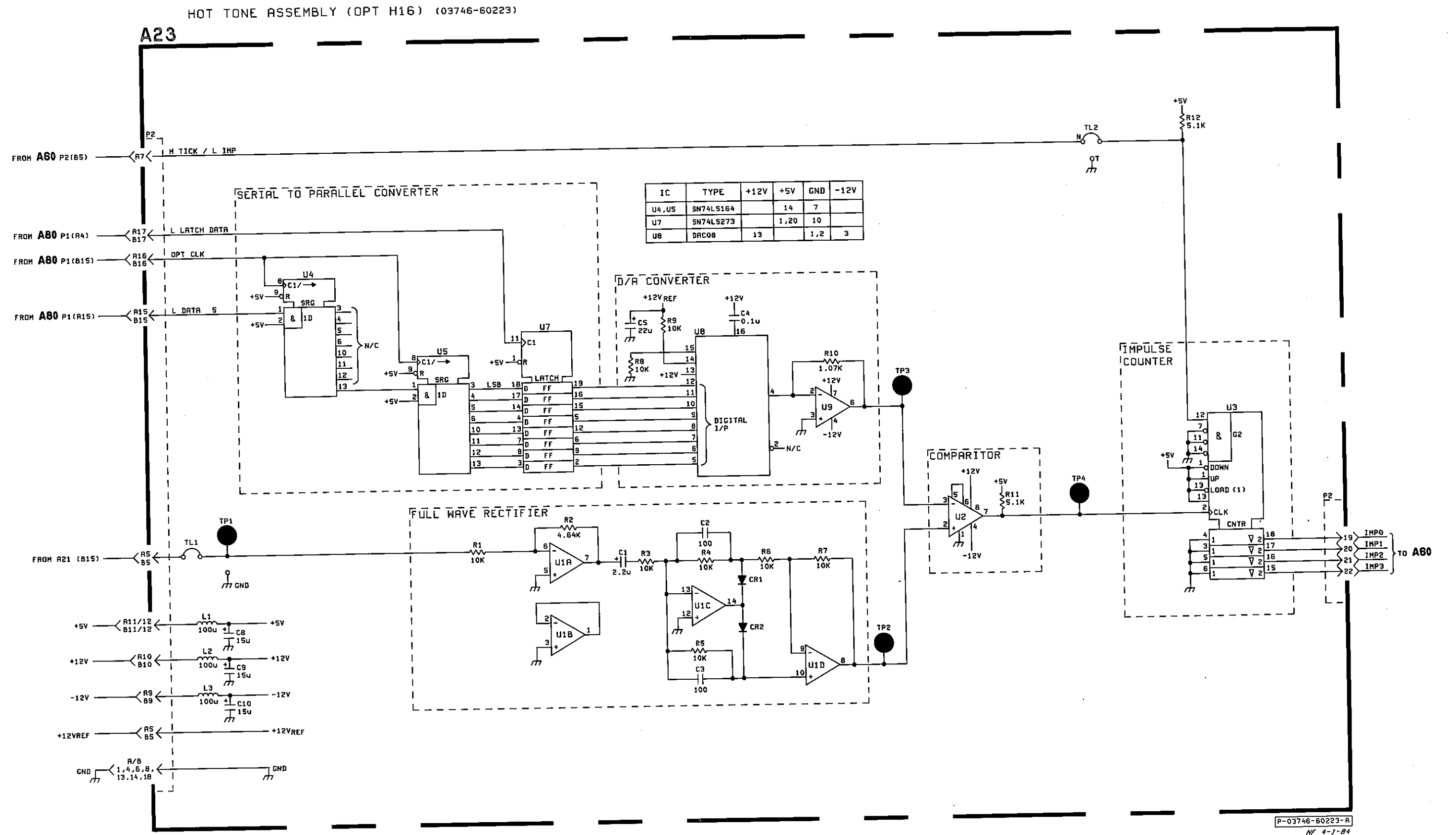
Figure A23-6 A23 Schematic Diagram
