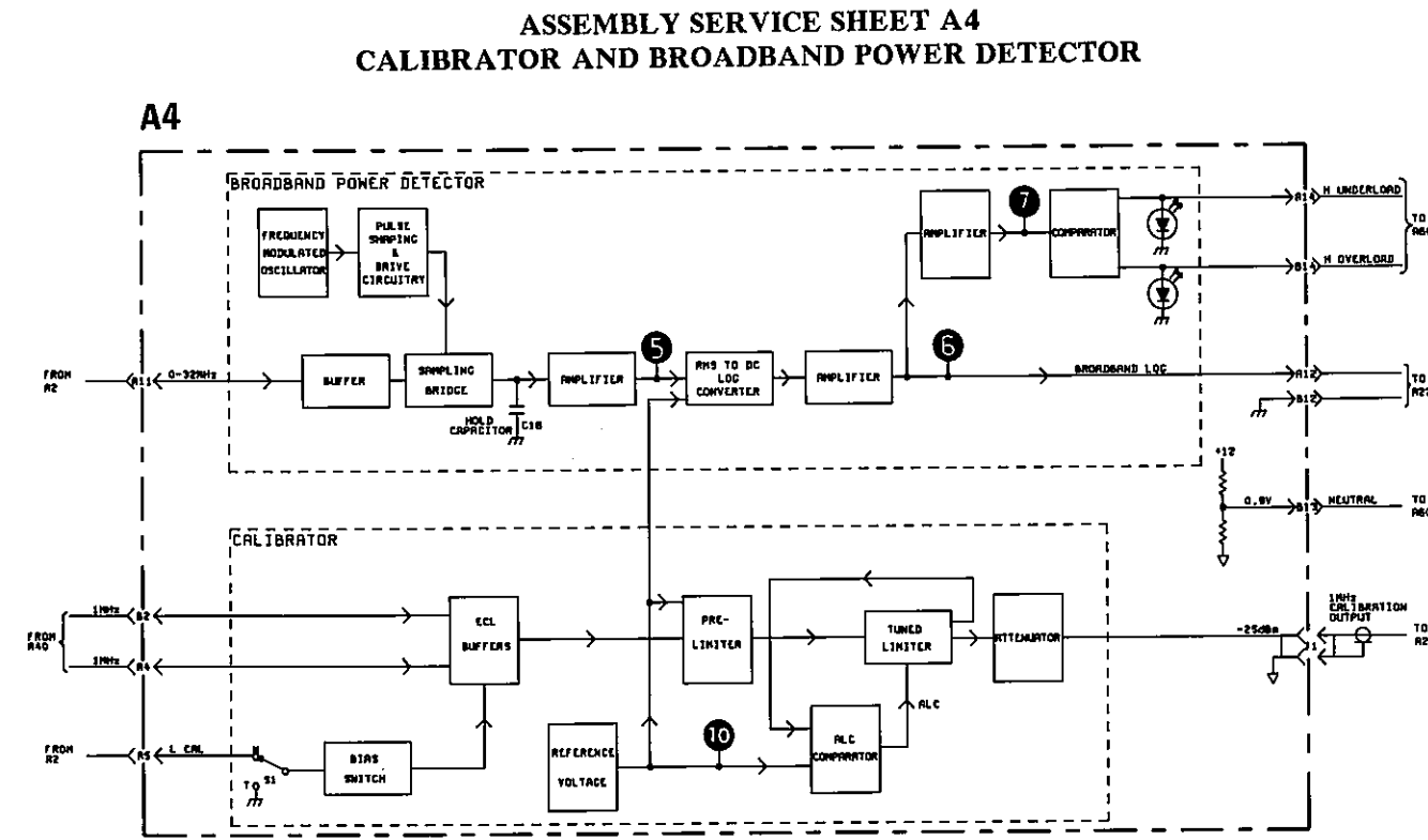
Figure A4-1 A4 Block Diagram
