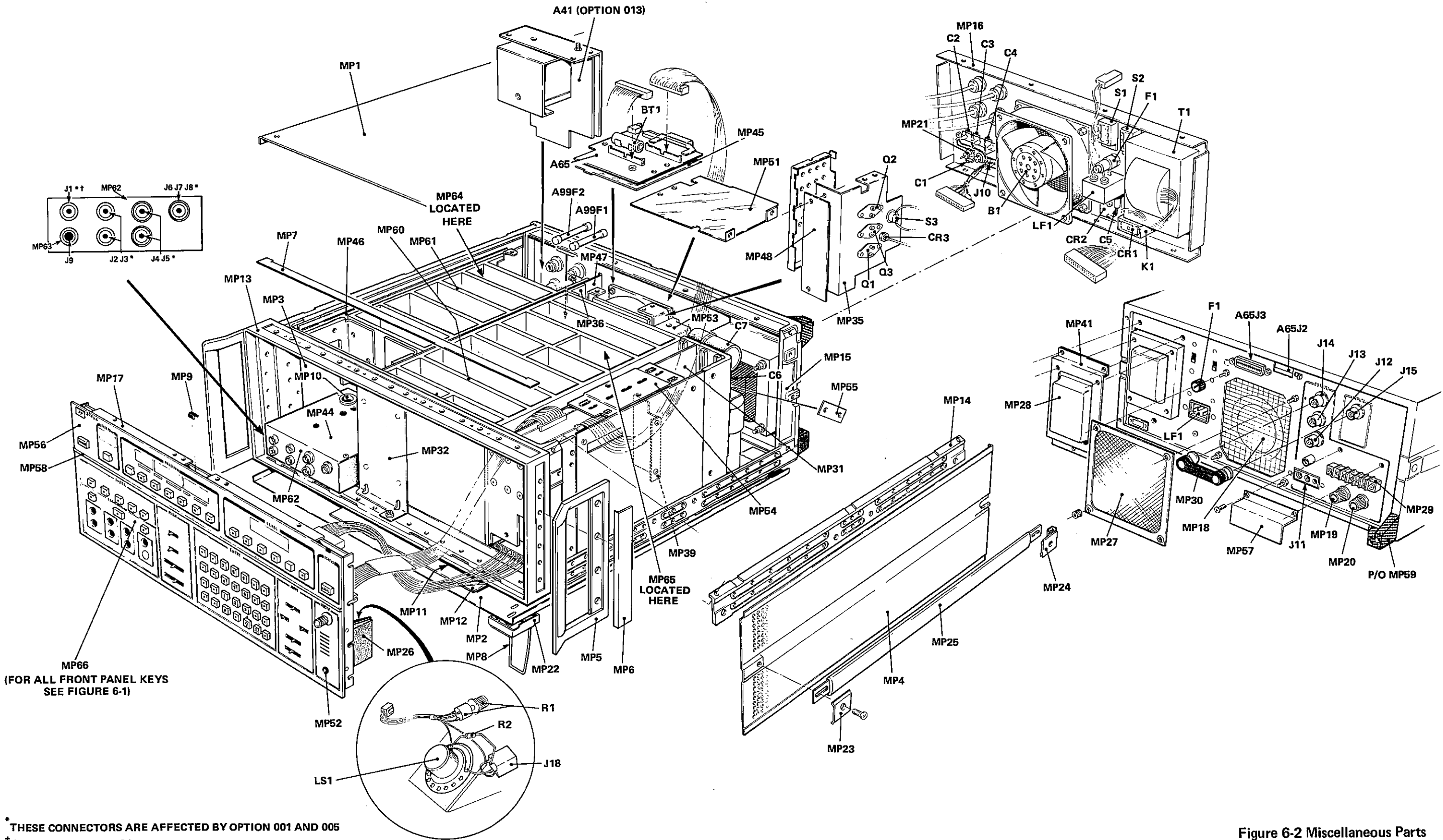
Figure 6-2 Miscellaneous Parts
