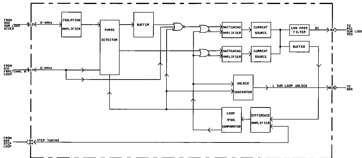
Figure A53-1 A53 Block Diagram
