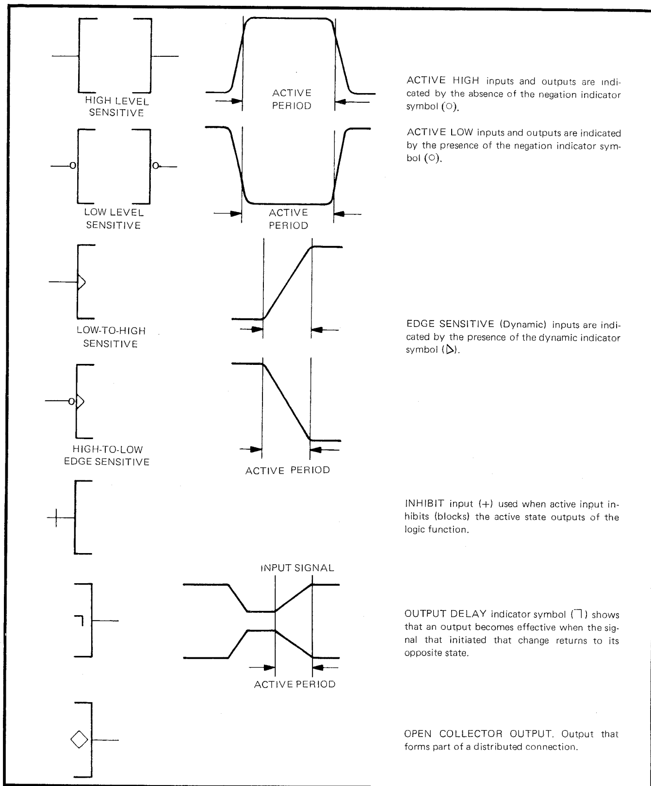
Figure 8-3 Indicator Symbols
