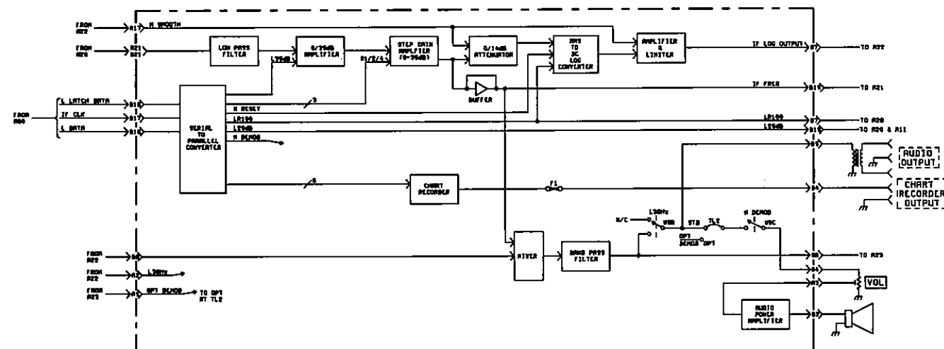
Figure A21-1 A21 Block Diagram
