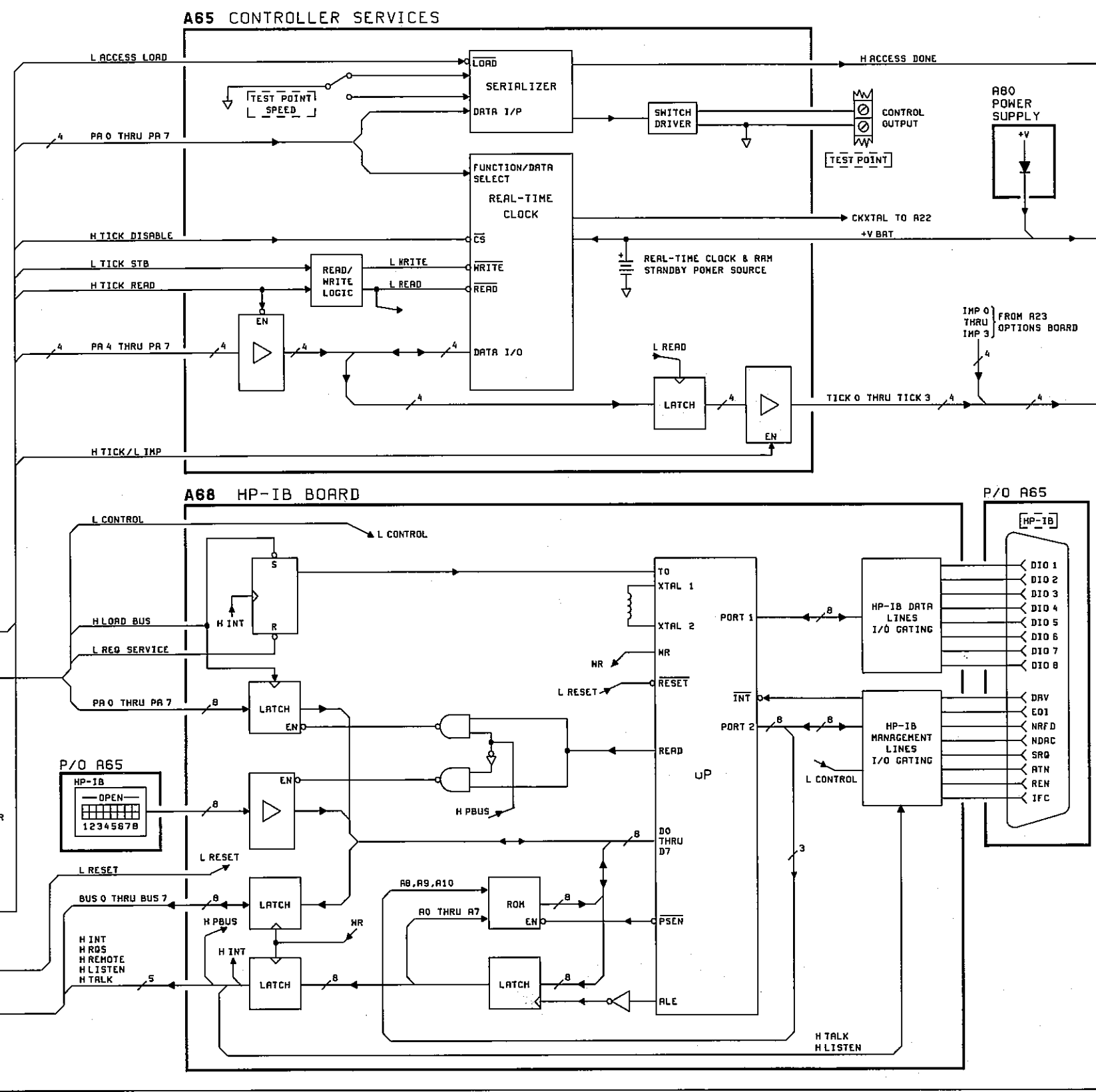
P-3746A-CONTROLLER- DC 28.7.81
