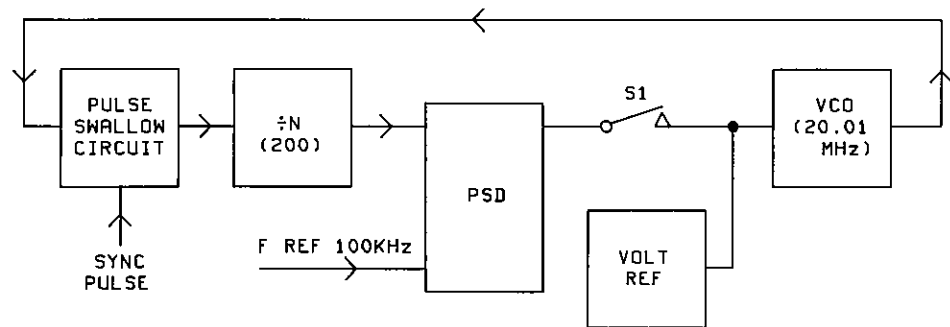
Figure A32-2 Simplified Fractional N Loop
