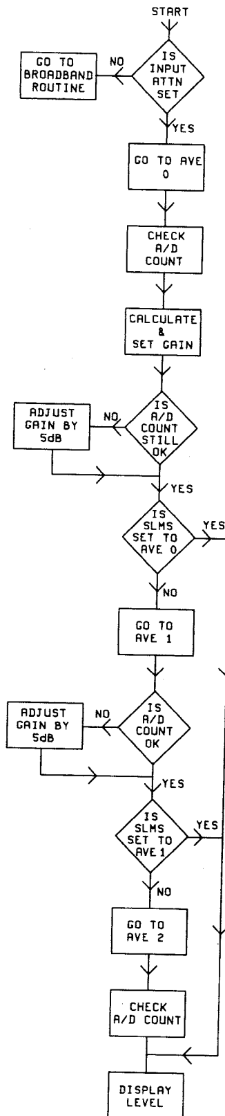
Figure 8R-6 Receiver Autoranging
