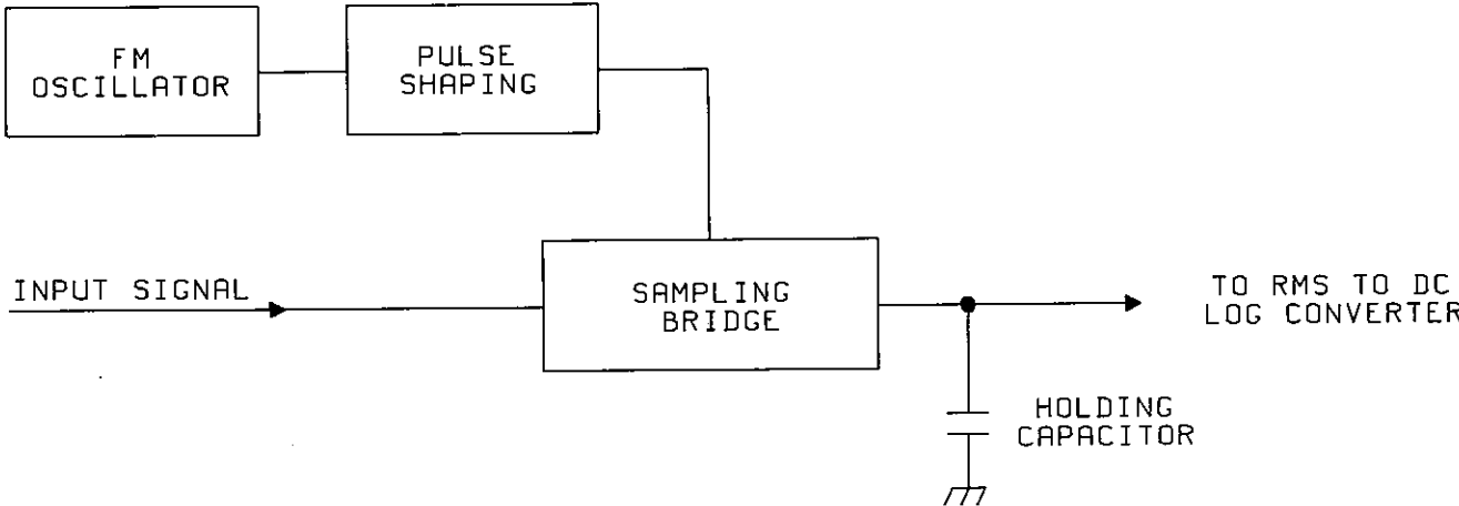
Figure A4-2 Simplified Broadband Power Detector
