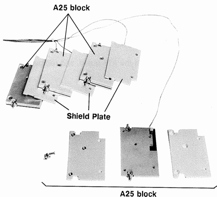
Figure 6. A25 Board Section Disassembly
