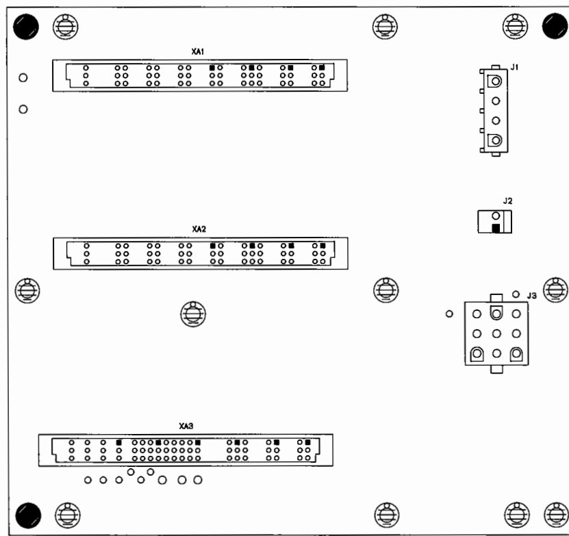
A14 Motherboard Power Supply Component Locations
