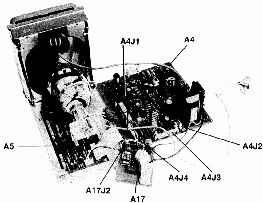
Figure 4. CRT Section Disassembly
