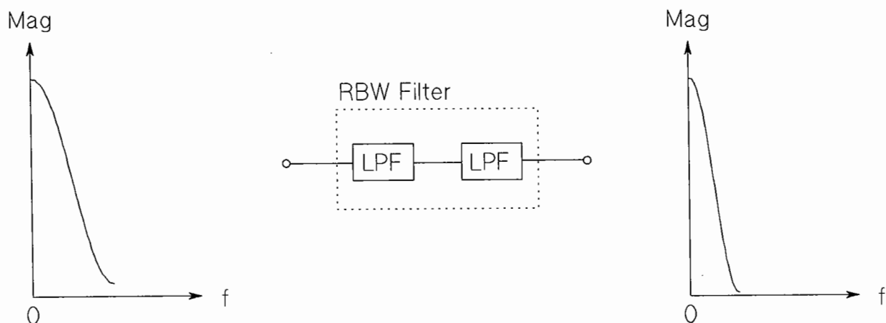
Figure 3. RBW Filter
