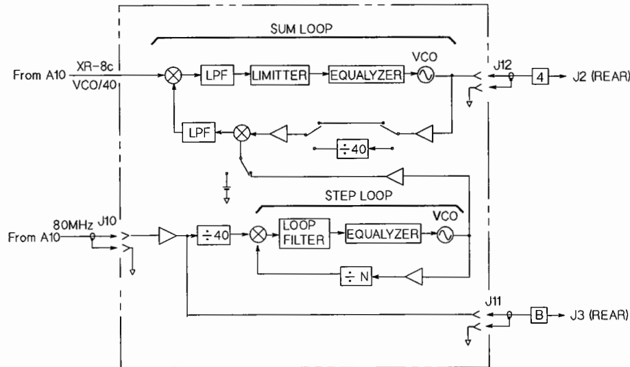
Figure 1. A18 Low Noise Oscillator Block Diagram
