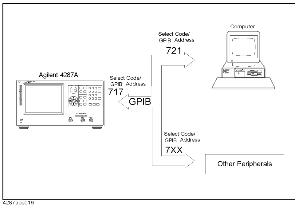
Setting up a GPIB remote control system
