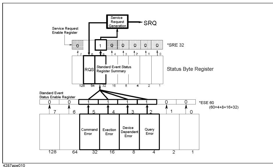
SRQ generation sequence (in response to an error)
