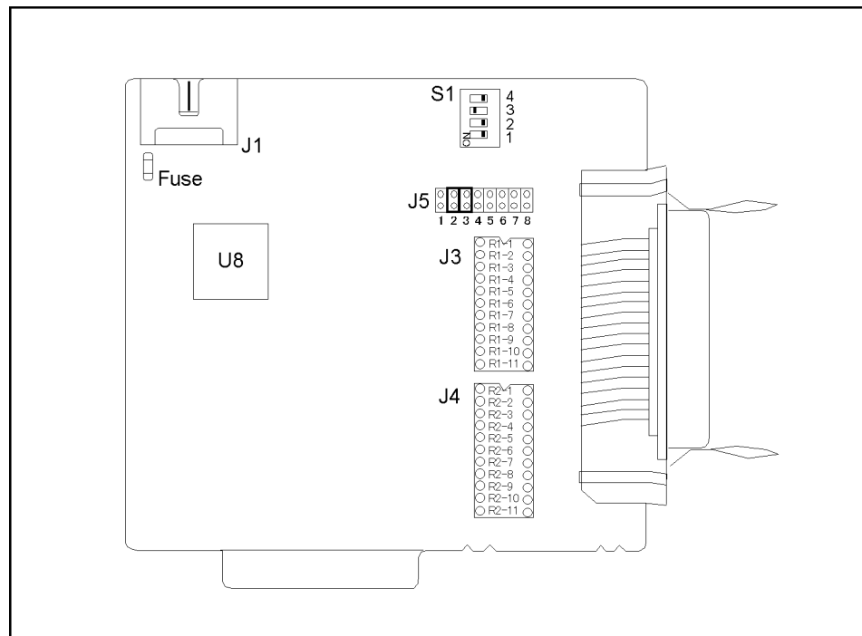
A23 Handler Interface Board
