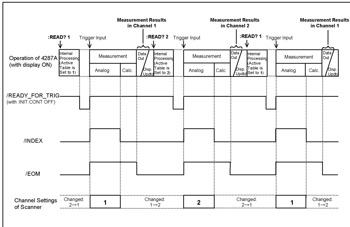
Figure 14-1 Timing Chart of Array Component Measurement (using 2 channels)
