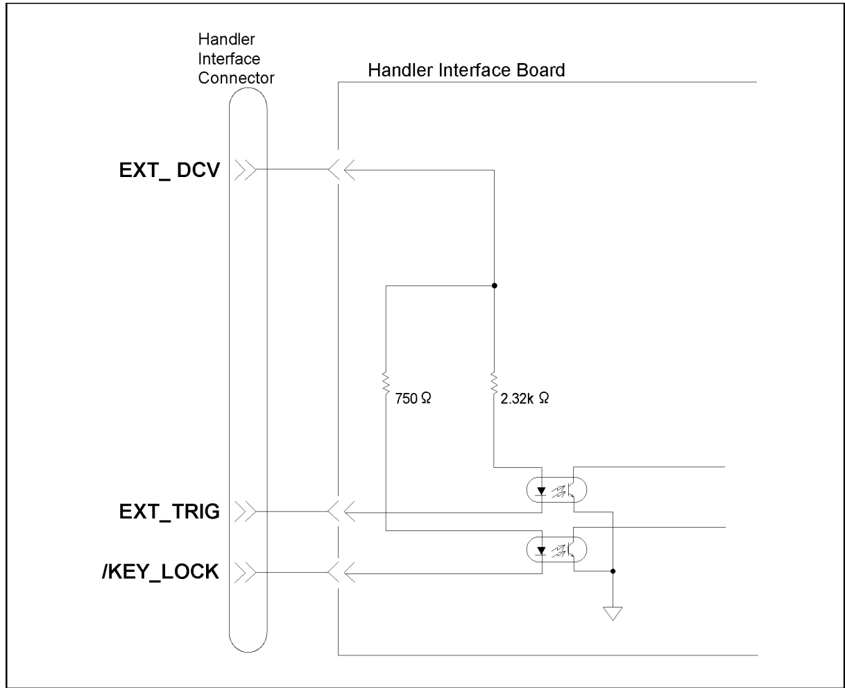
Figure 12-4 Circuit diagram for handler interface input signals
