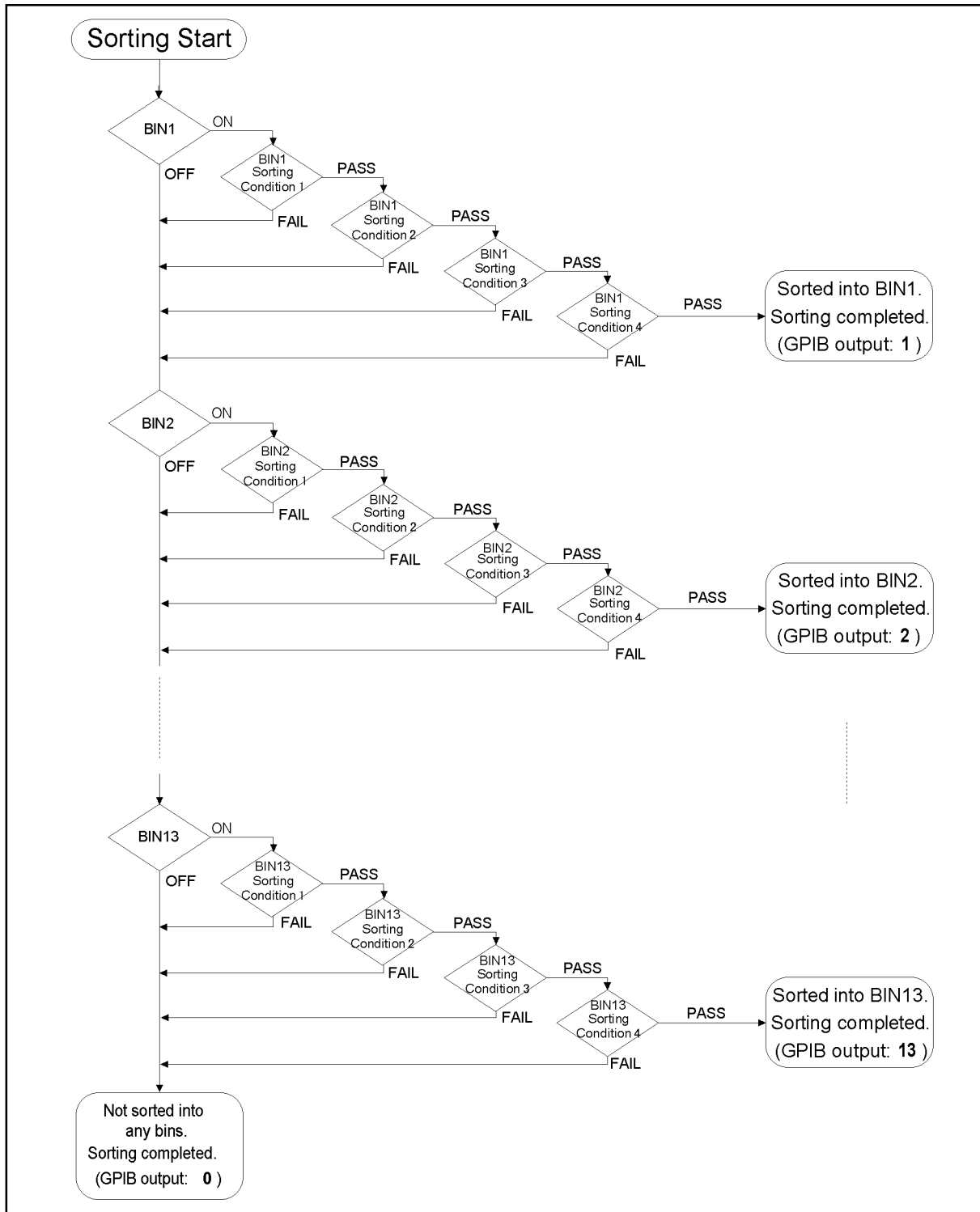
Figure 7-2 Sorting flow
