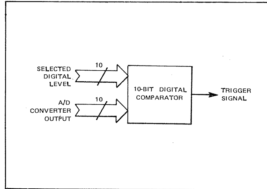
Figure 3-8. Digitized Samples Compared with Selected Trigger Level
