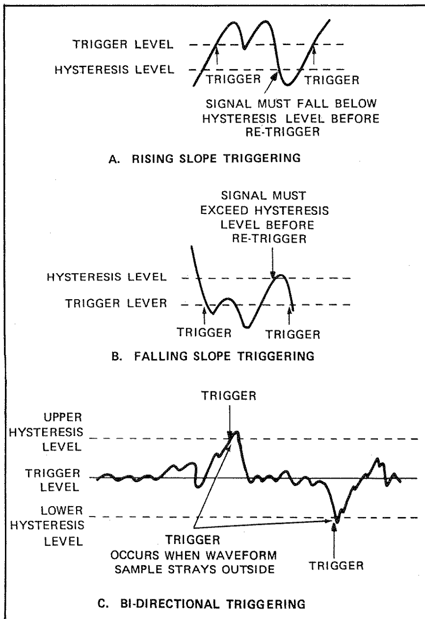
Figure 3-10. Selectable Hysteresis
