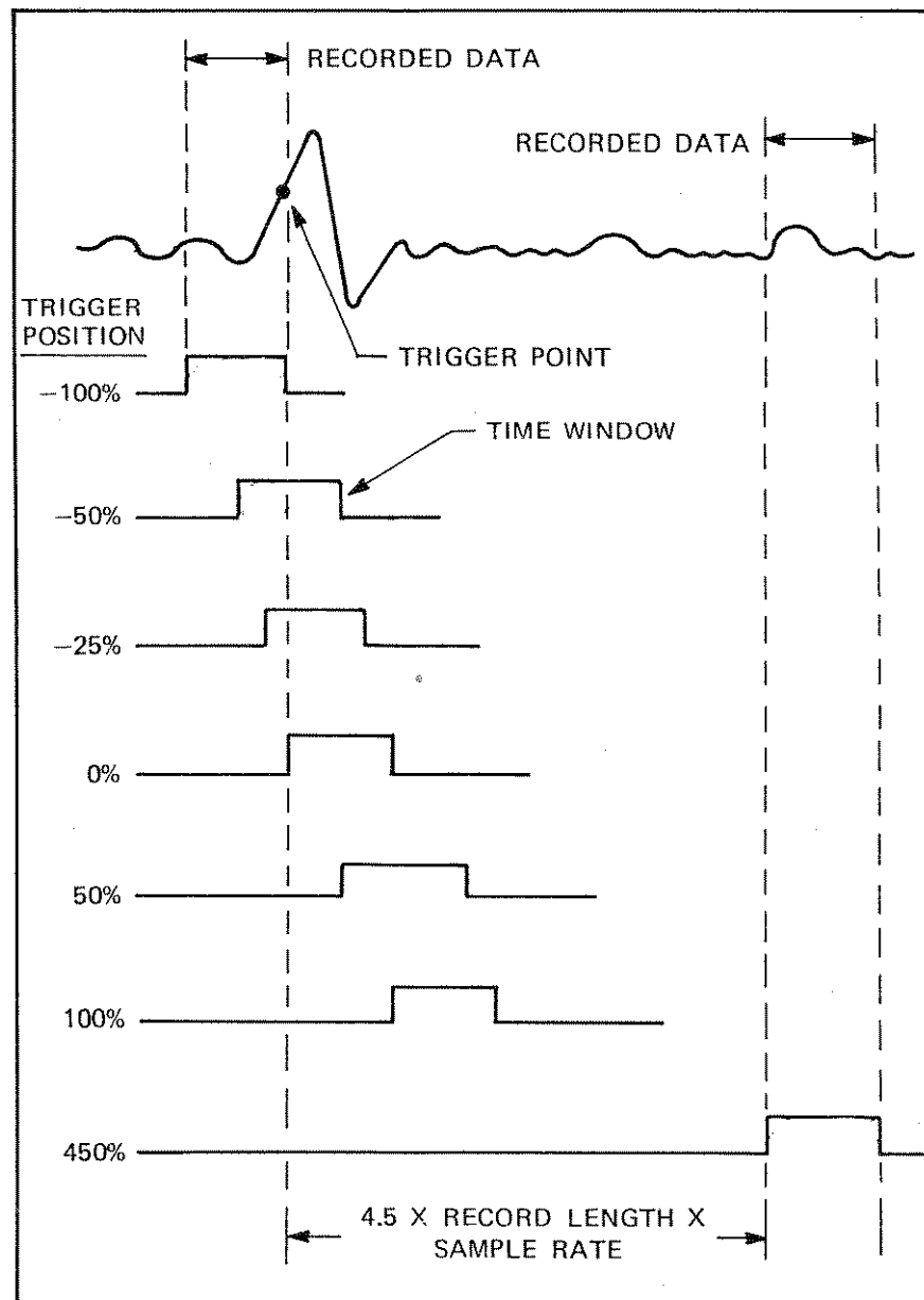
Figure 3-9. Trigger Position Selection of Recorded Data
