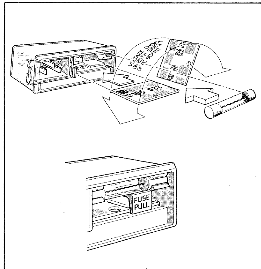
Figure 2-1. Voltage Selection with Power Module PC Board
