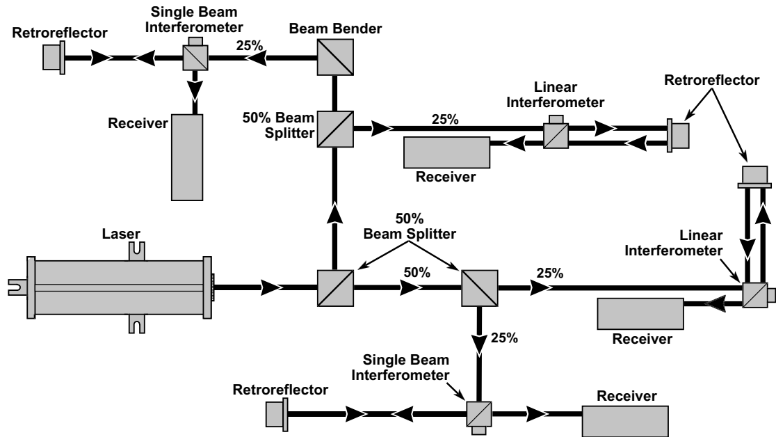
Figure 3-9. Four-axis configuration
