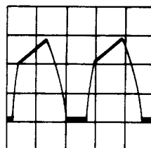
WAVEFORM 5 Ip MONITOR 0.4V/DIV 20 \mu s/DIV OUTPUT SHORTED ISET = 17A (6030A) ISET = 120A (6031A) ISET = 50A (6032A) ISET = 5A (6035A)
