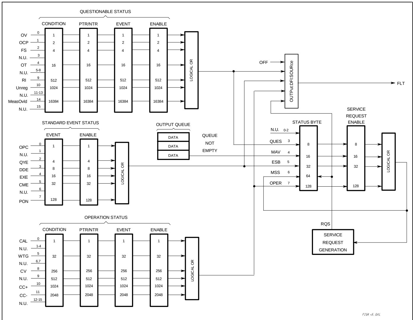
Figure 3-7. DC Source Status Model
