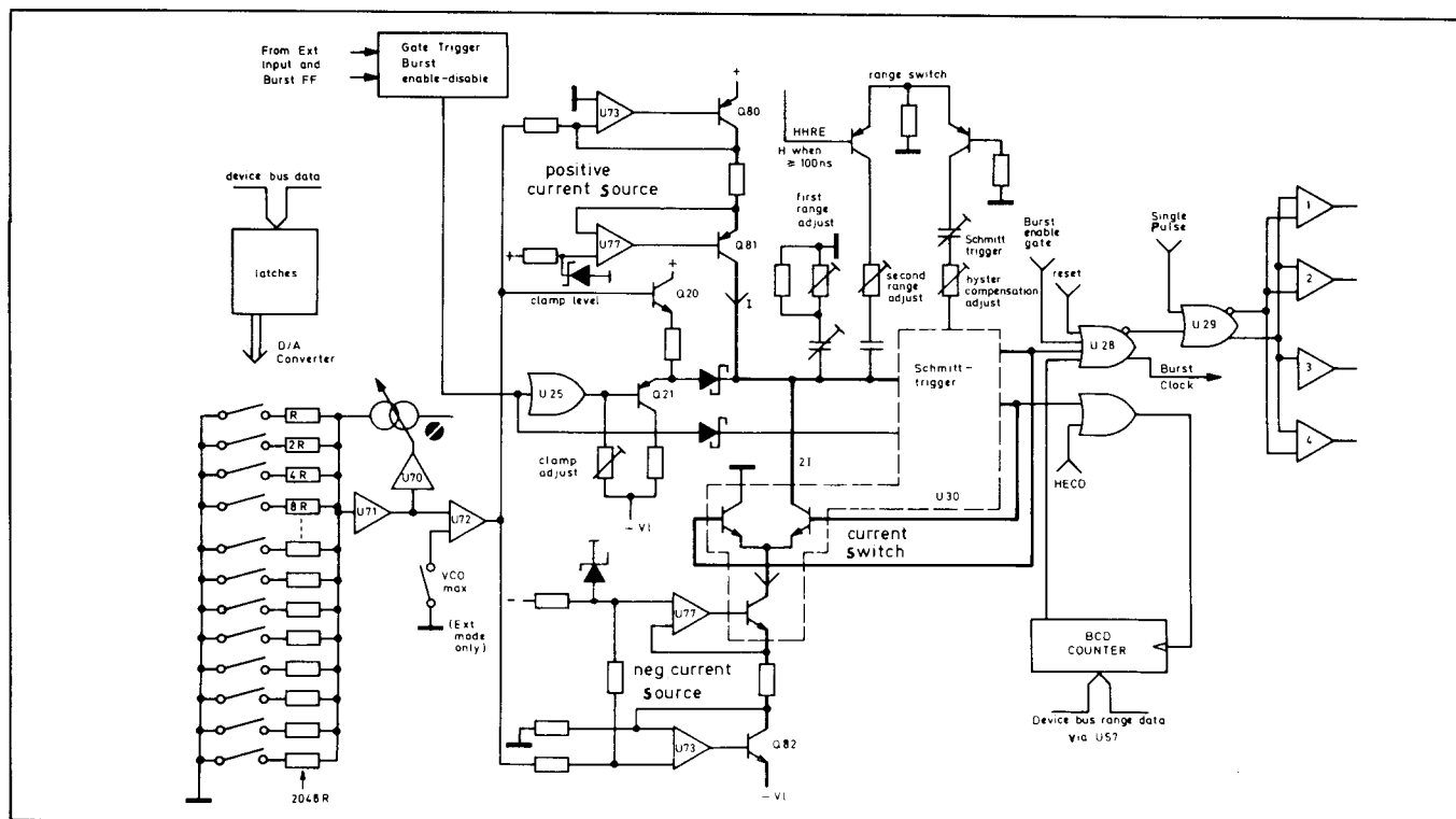
Figure 8—9—1. Rate control
