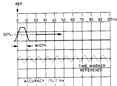
FIGURE 4-12 WIDTH MEASUREMENTS
