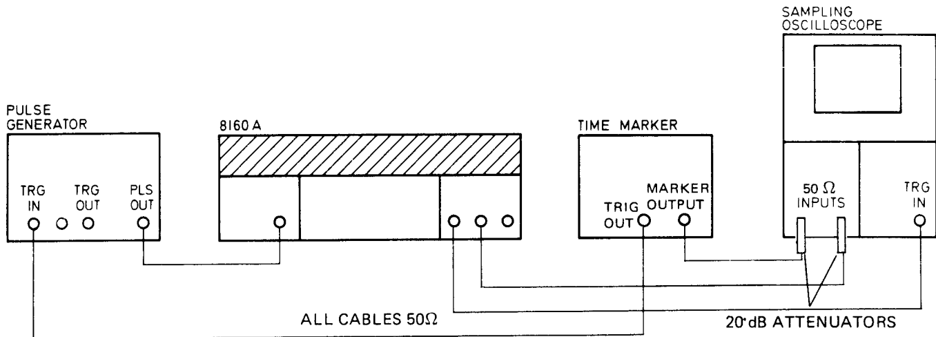
Figure 4-14. Transition Time – Fast Test Set-up
