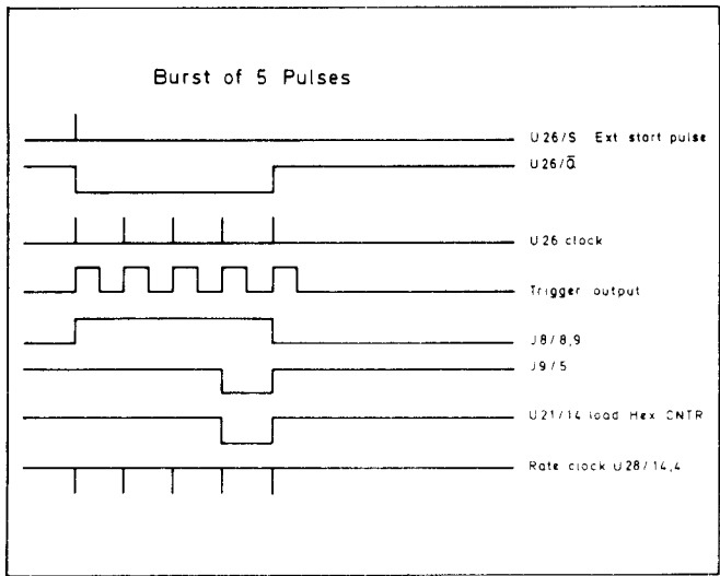
Figure 8–8–2. Timing Diagram
