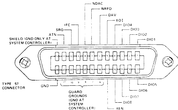
Figure 2-3. HP-IB Connector
