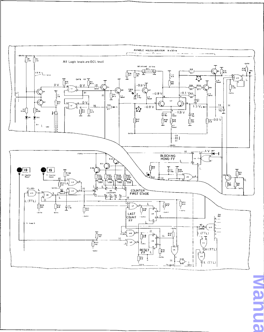
Figure 8-10-15. Astable multivibrator
