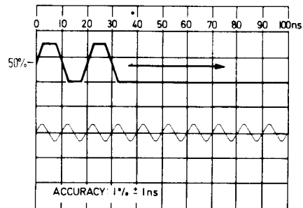
FIGURE 4-9 DOUBLE PULSE
