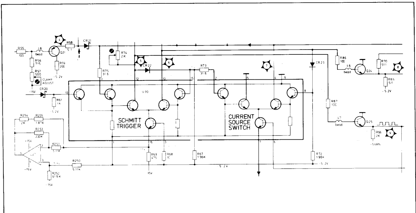
Figure 8–9–5. VCO voltages
