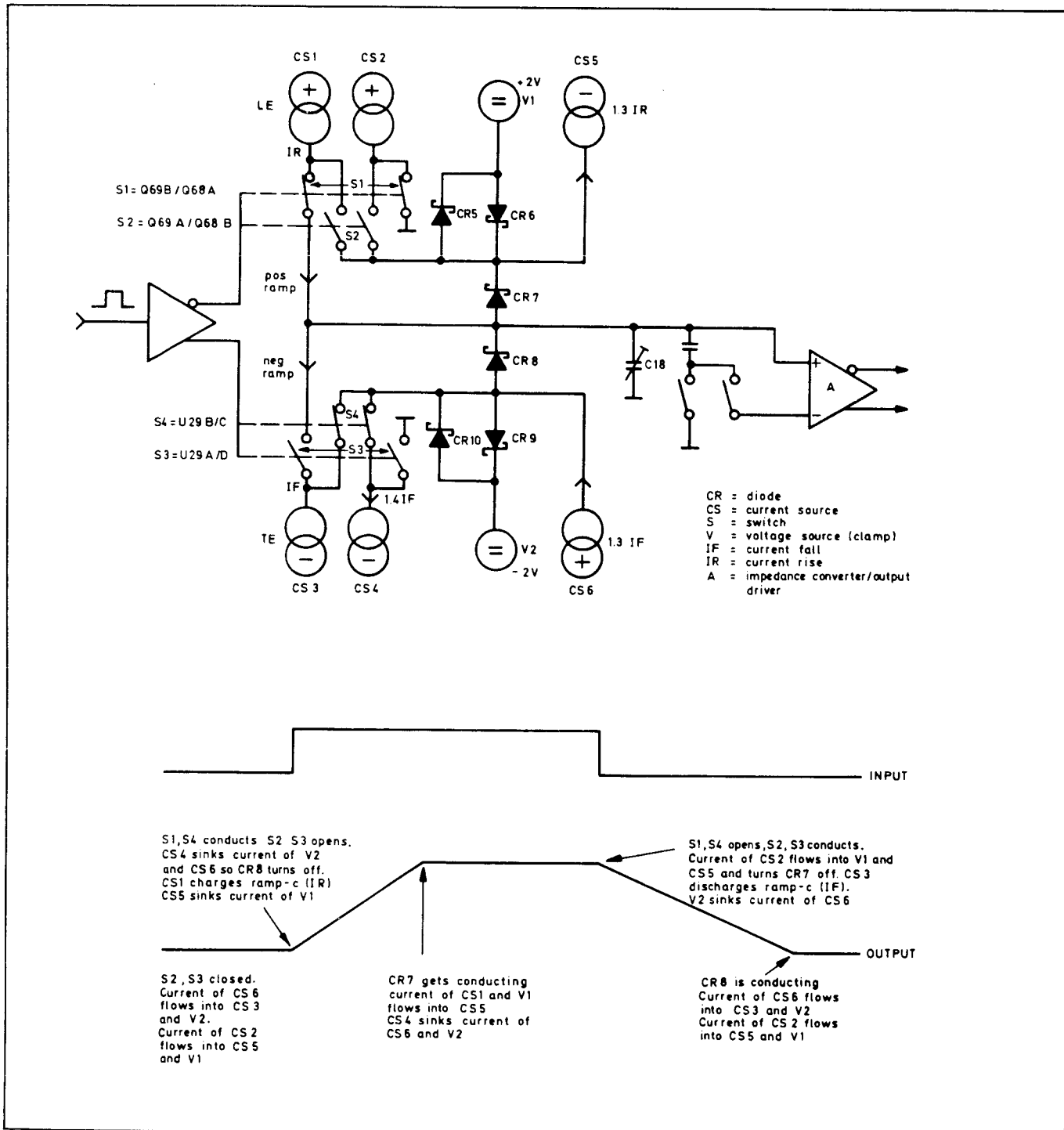
Figure 8-11-2. Integrator functional diagram
