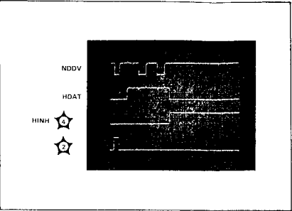
Slope Data Acceptor (All signals are TTL level) Timebase: 50 \mu s/div.
