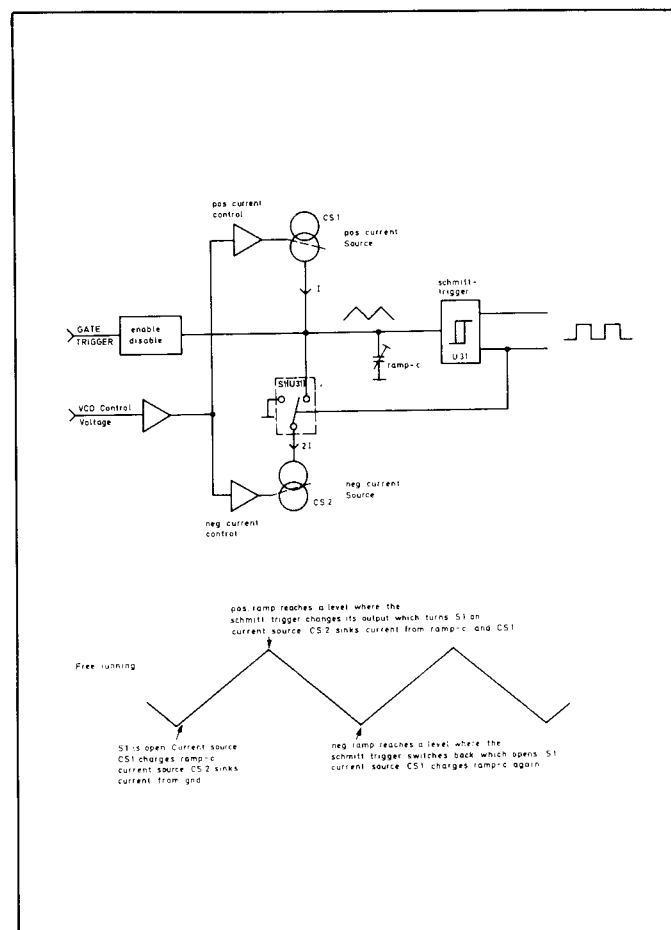
Figure 8—9—2. VCO-Rate generator
