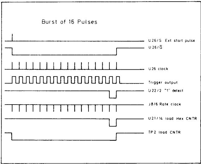
Figure 8- 8-3. Timing Diagram
