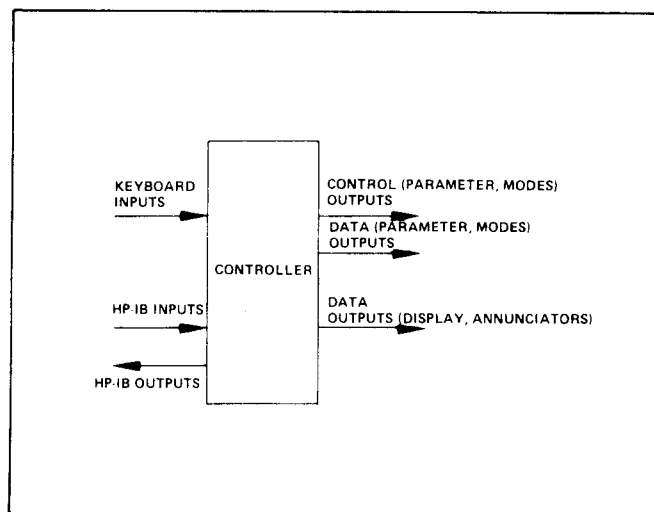
Figure 8-7-1. Controller Inputs and Outputs
