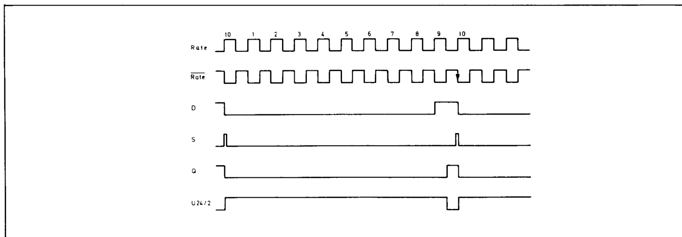
Figure 8—9—4. Timing Diagram
