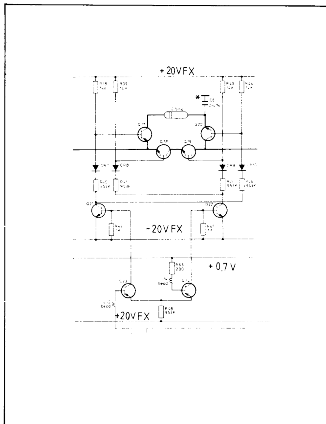
Figure 8–10–4. Delay line switch
