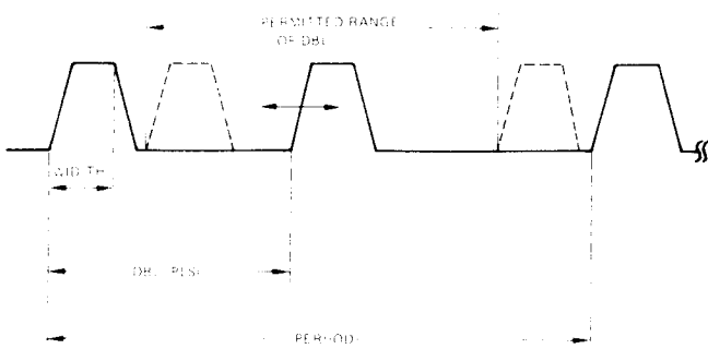
Figure 3-3. Double Pulse Limits
