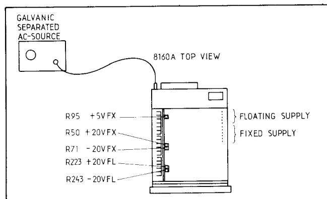
Figure 8–3–2. Test Setup
