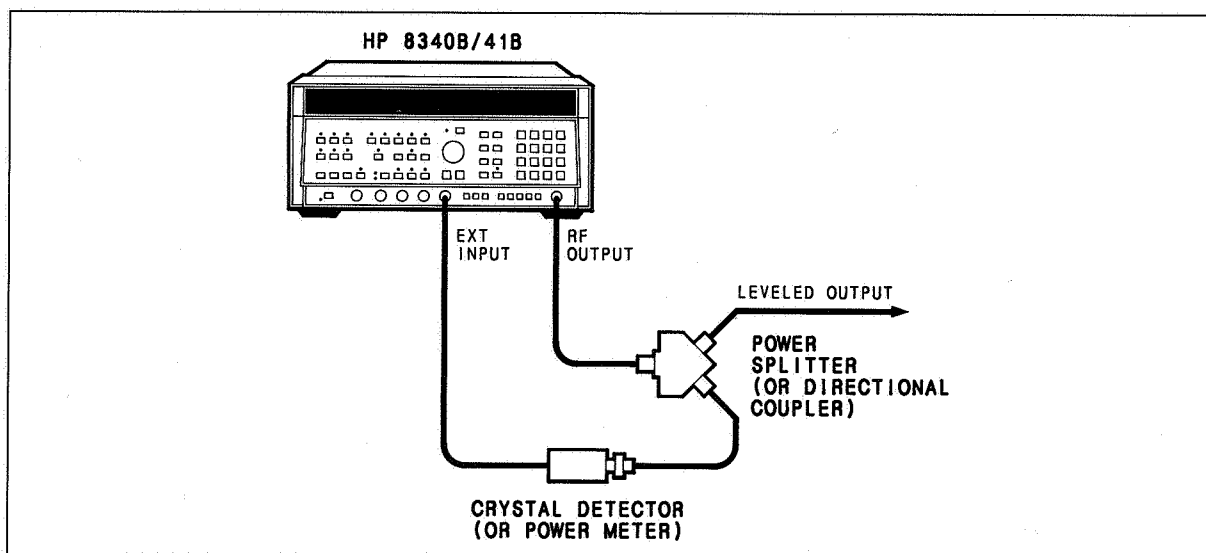
Figure 3-32. Typical External Leveling Hookup
