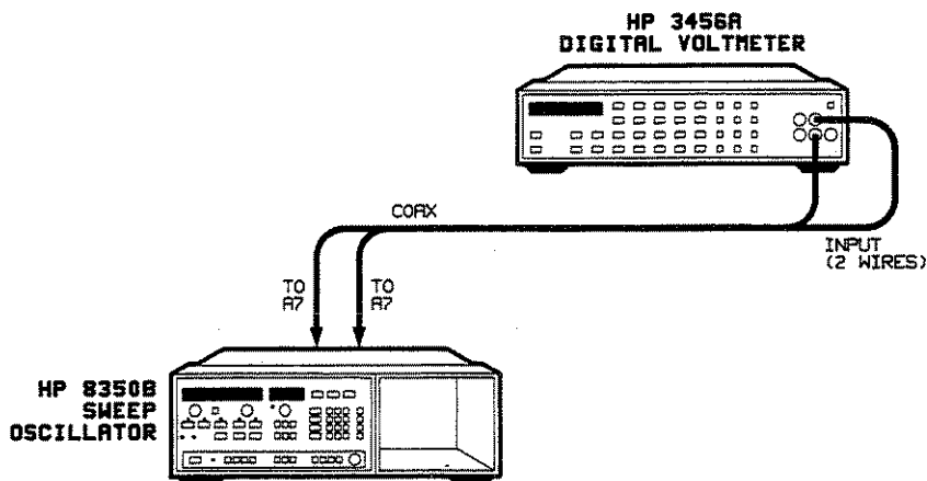
Figure 5-4. +5VA/B Power Supply Adjustment Setup
