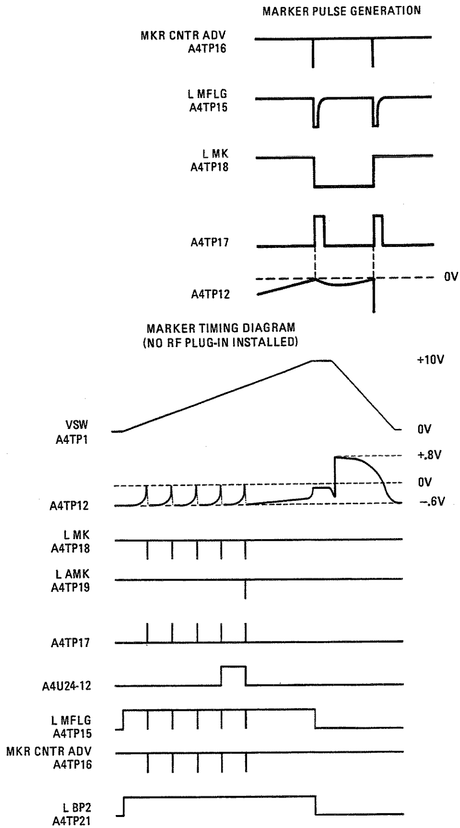
Figure 8-29. Marker Timing Diagrams
