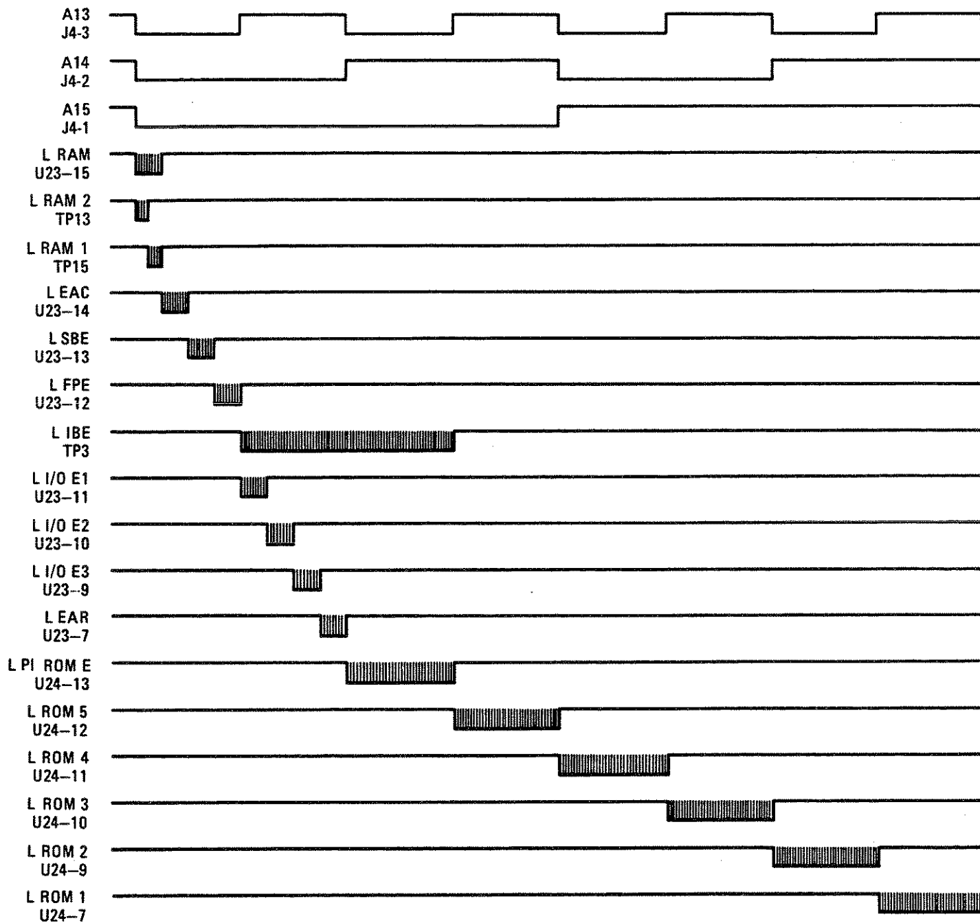
Figure 8-21. Free Run Test, Timing Diagram
