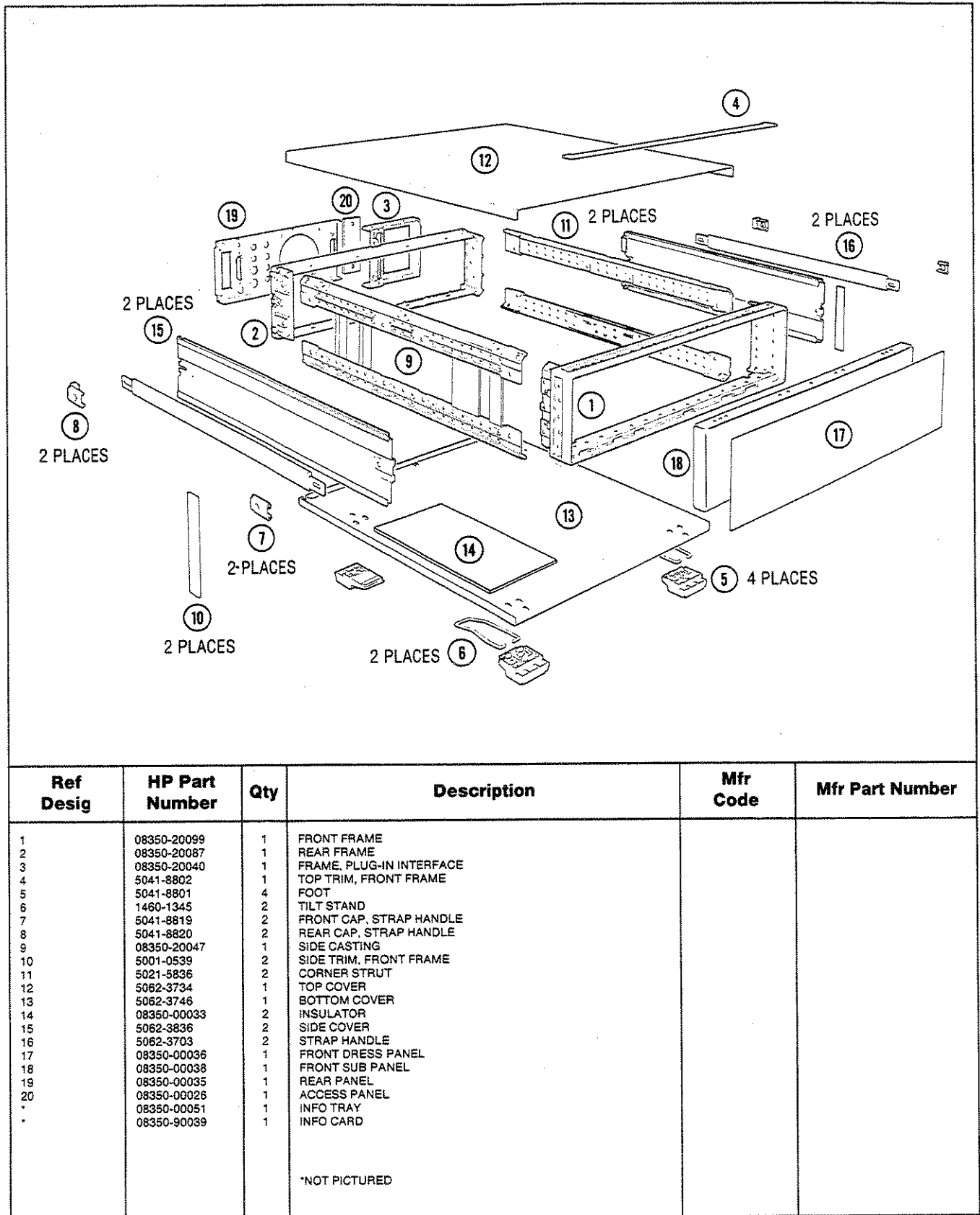
Figure 6-11. Chassis Parts Identification
