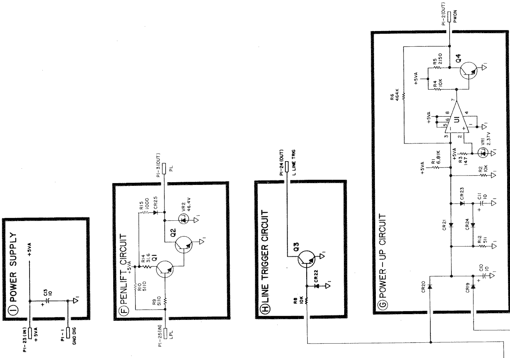
Figure 8-43. A6 Rectifier, Schematic Diagram (Change B)
