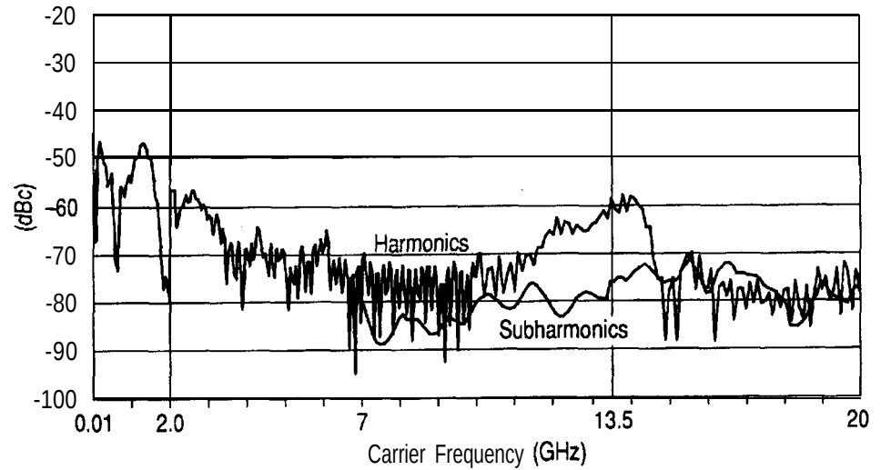
Typical HP 83620A Harmonics &amp; Subharmonics
