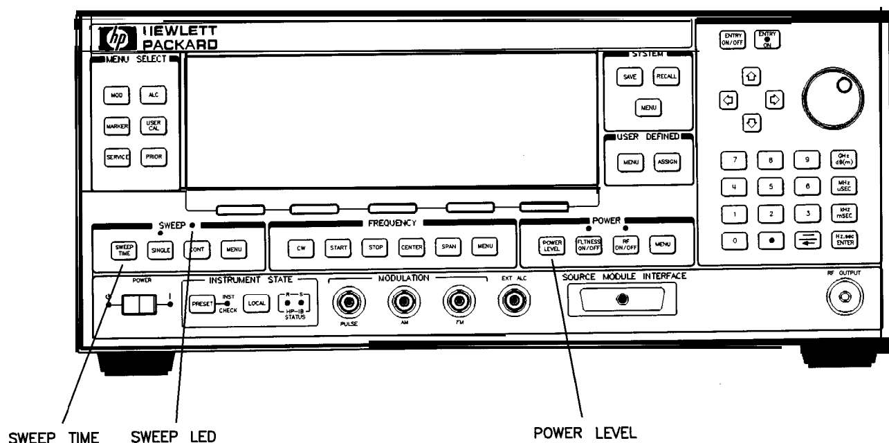
Figure 1-6. Power Level and Sweep Time Operation
