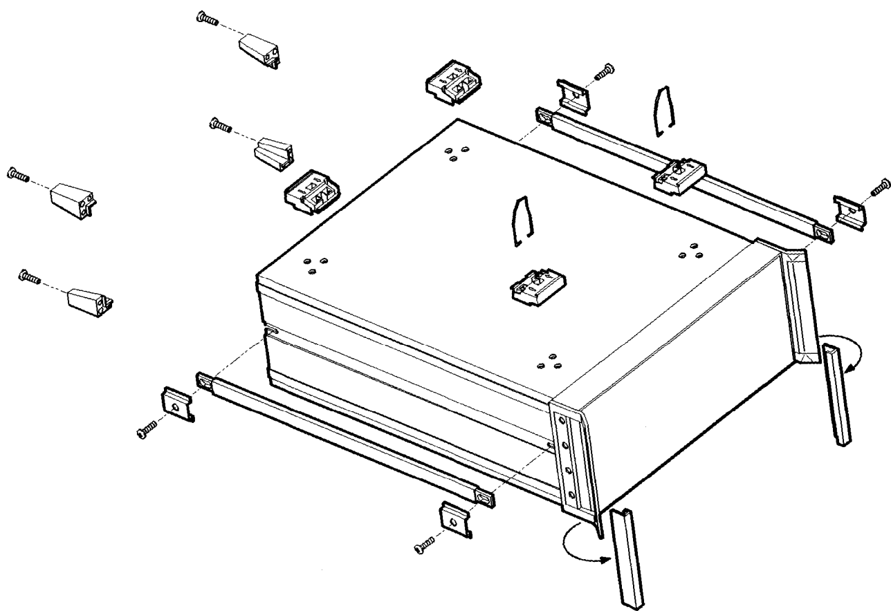
Figure 3-3. Removing the Side Straps and Feet
