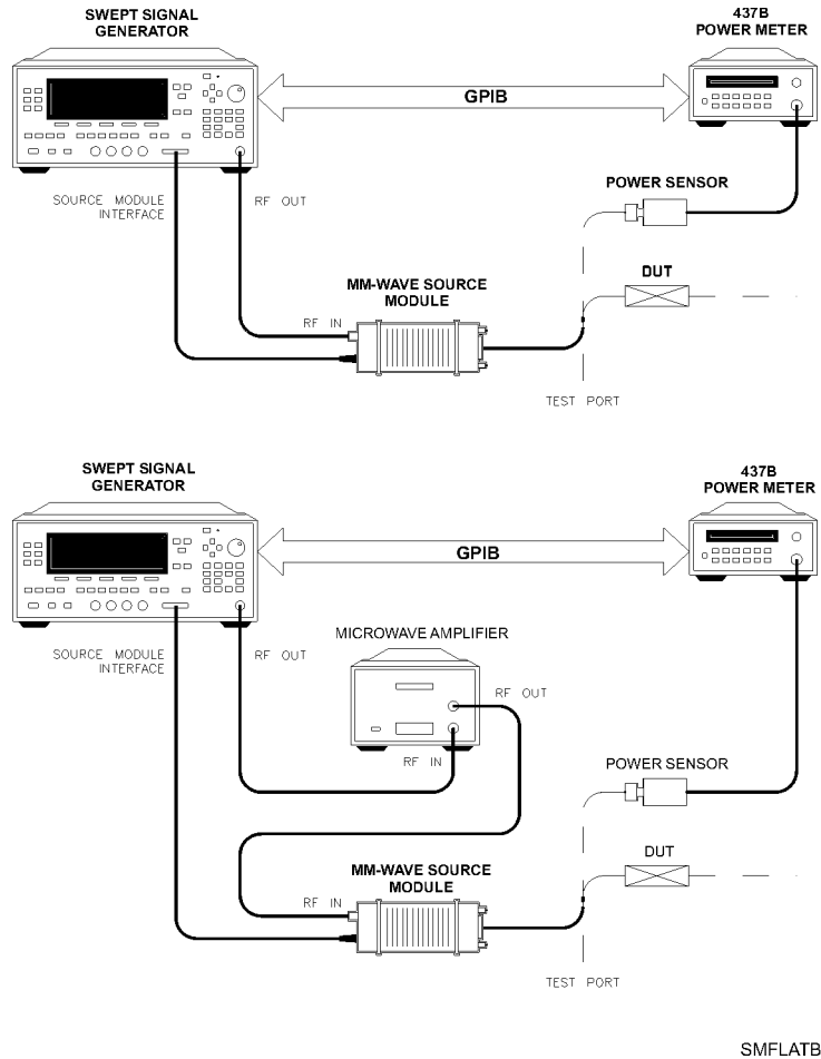
Figure 1-20. Creating Arbitrarily Spaced Frequency-Correction Pairs in a Swept mm-wave Environment
