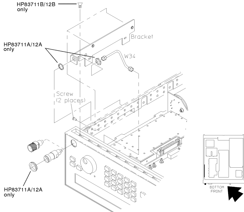
Figure 5-30. RF Output Connector Removal-Standard
