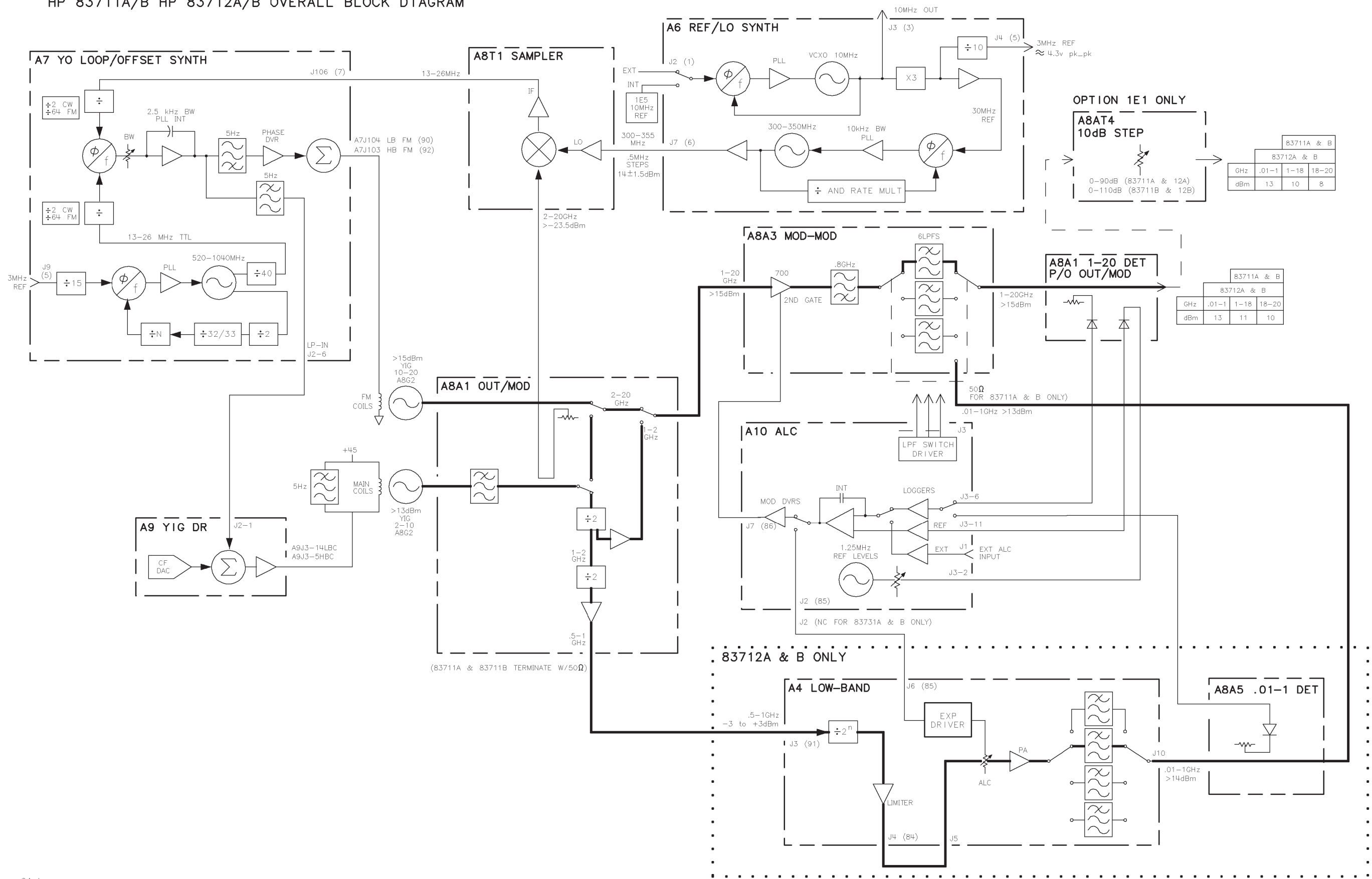
HP 83711A/B HP 83712A/B OVERALL BLOCK DIAGRAM
