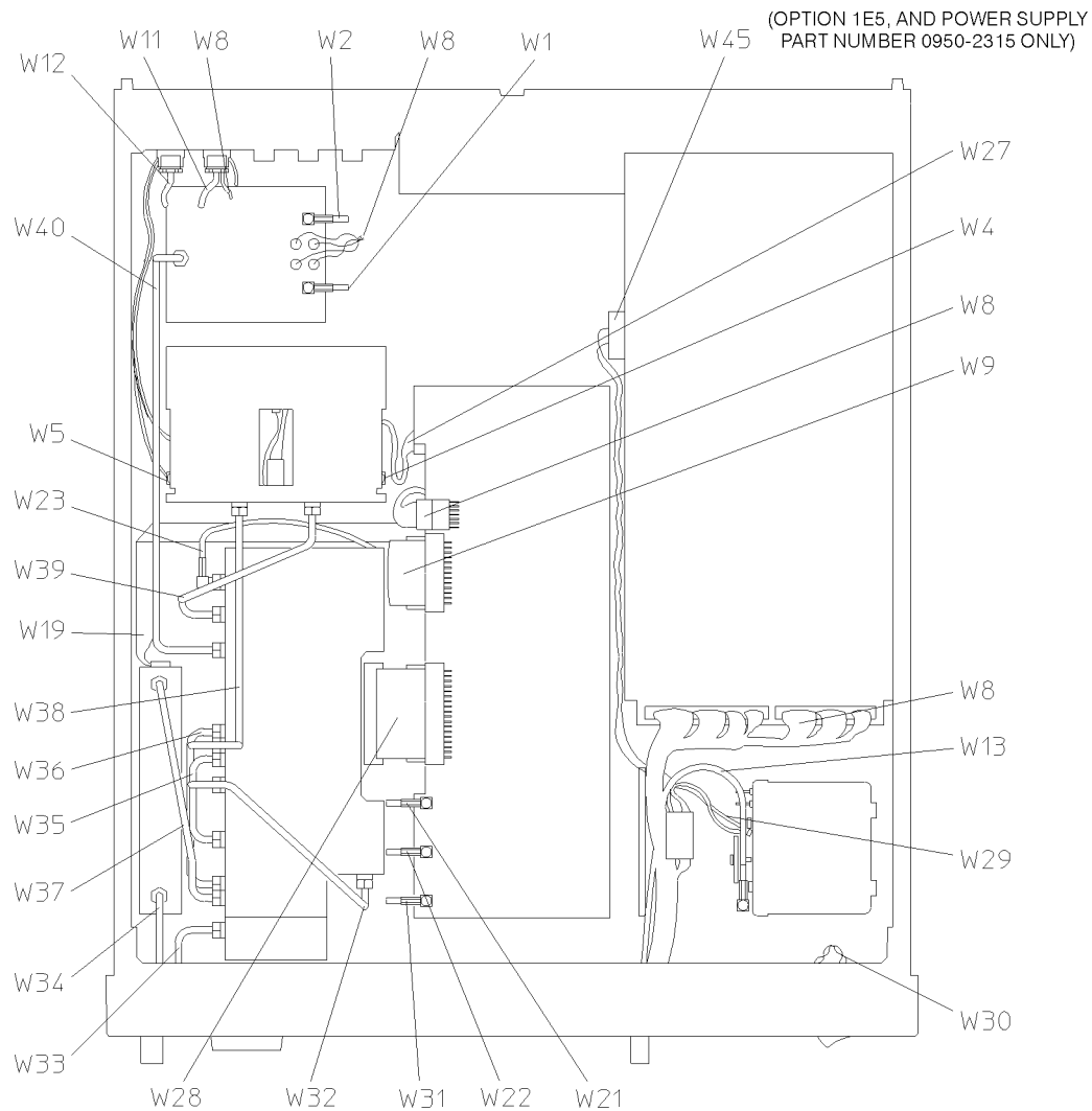
Figure 3-4. Cable Assemblies – Bottom View
