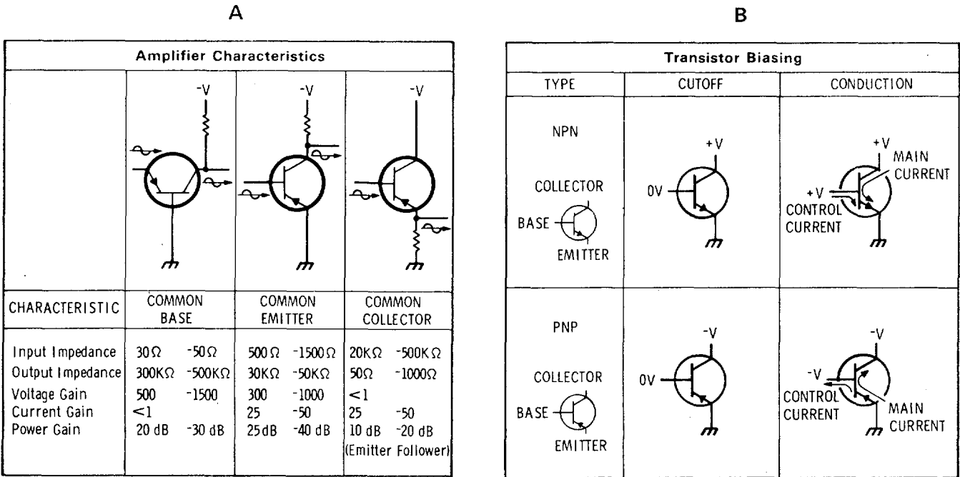
Figure 8-1. Transistor Operation 8-5
