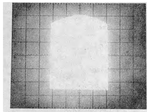
Figure 5-6. First Converter Passband CR T Display
