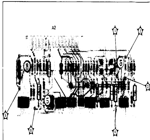
Figure 8-10. Modulator/Oscillator Driver Assv A2 Component Locations
