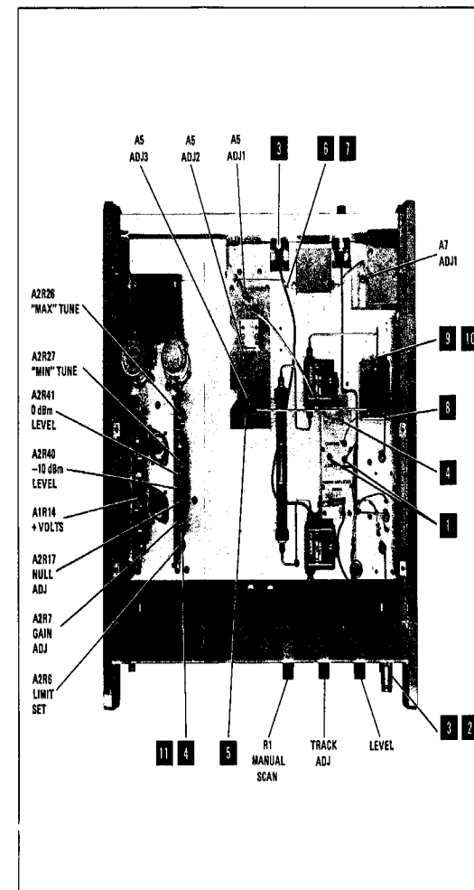
Figure 8-5. Adjustment and Test Point
