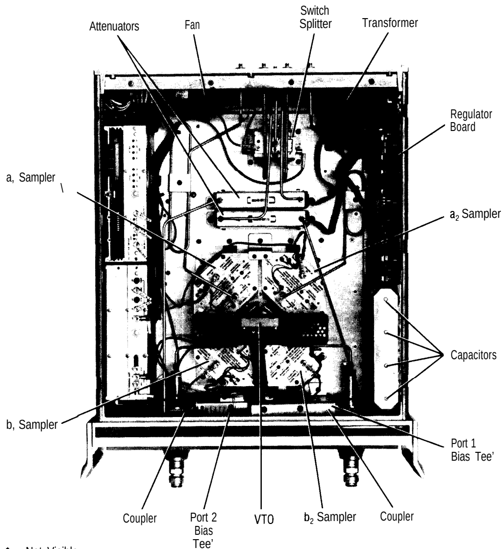
Figure 5-6. General Component Location Diagram
