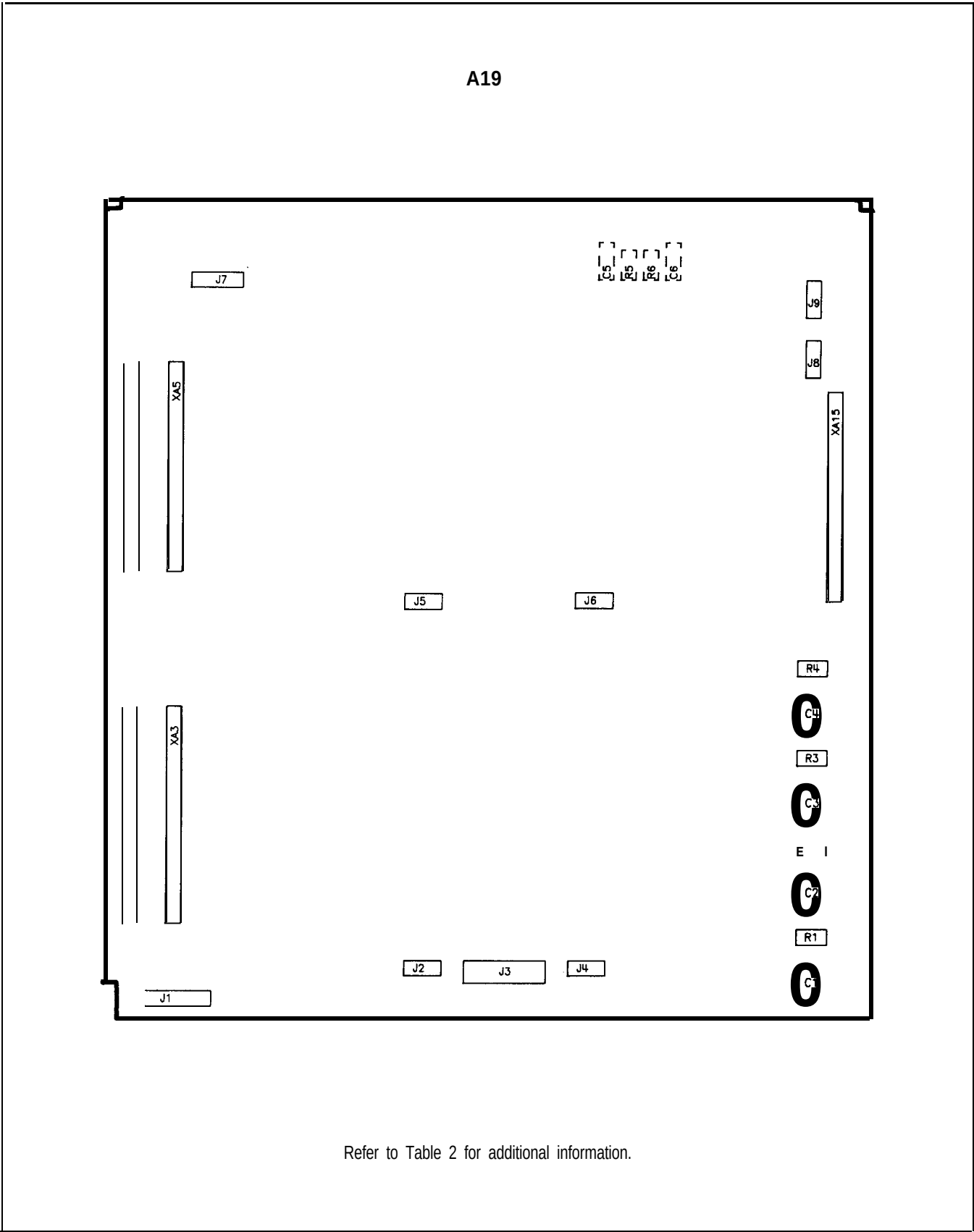
Figure 6-3. HP 8514B and HP 8512A Motherboard Component Location Diagram
