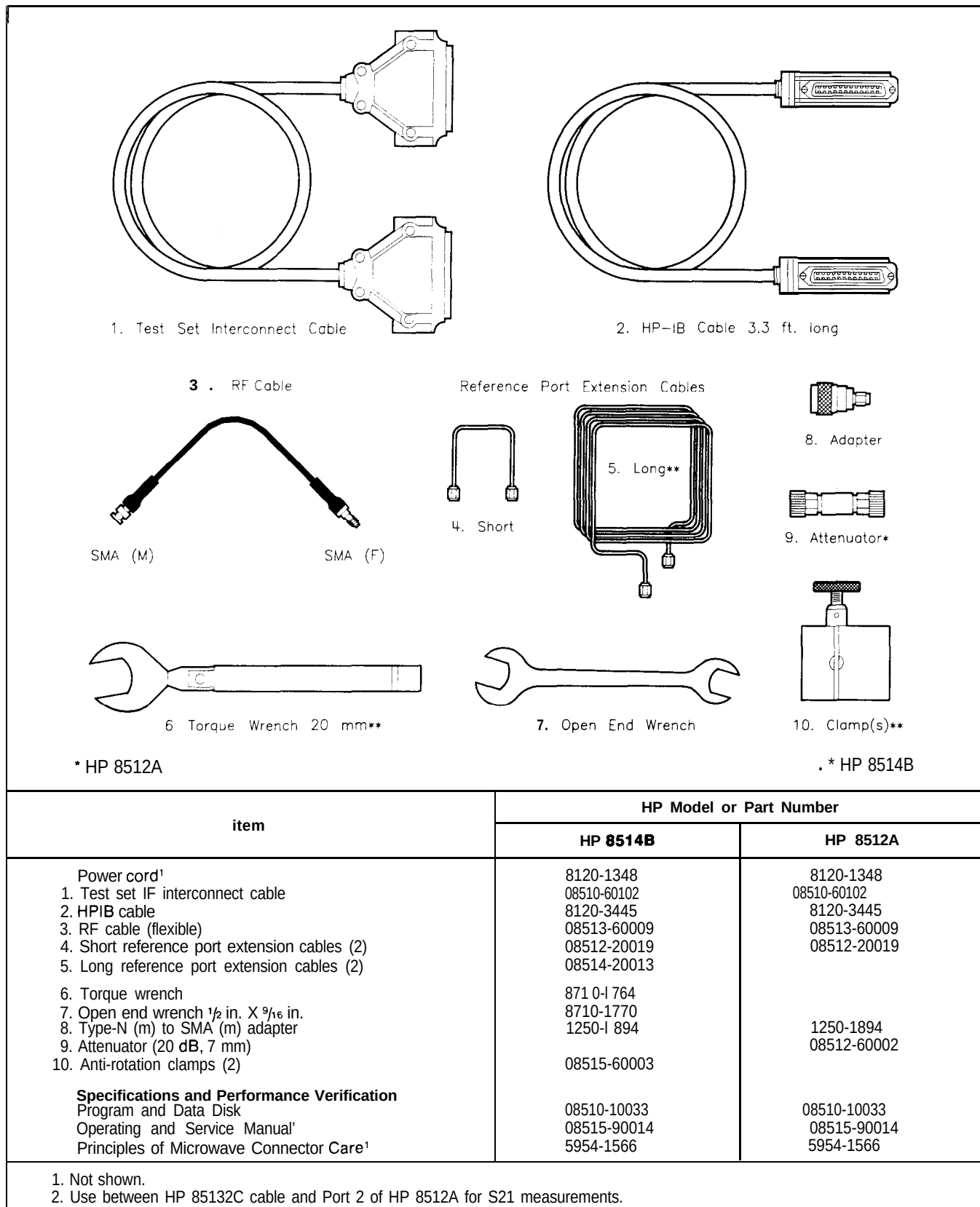
Figure 2-1. Accessories supplied with HP 8514B and HP 8512A
