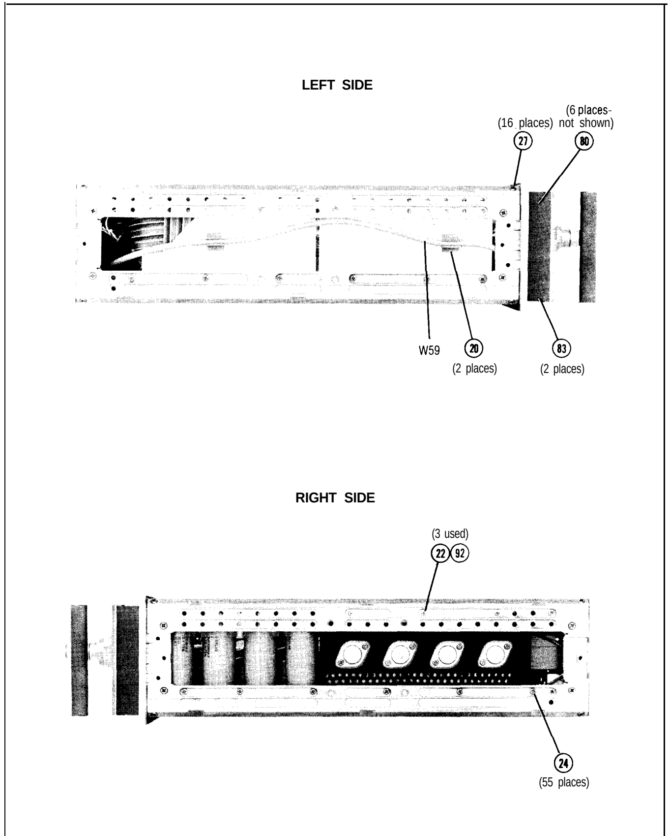
Figure 6-2. HP 8514B Miscellaneous Mechanical, Chassis, and Electrical Parts (2 of 5)
