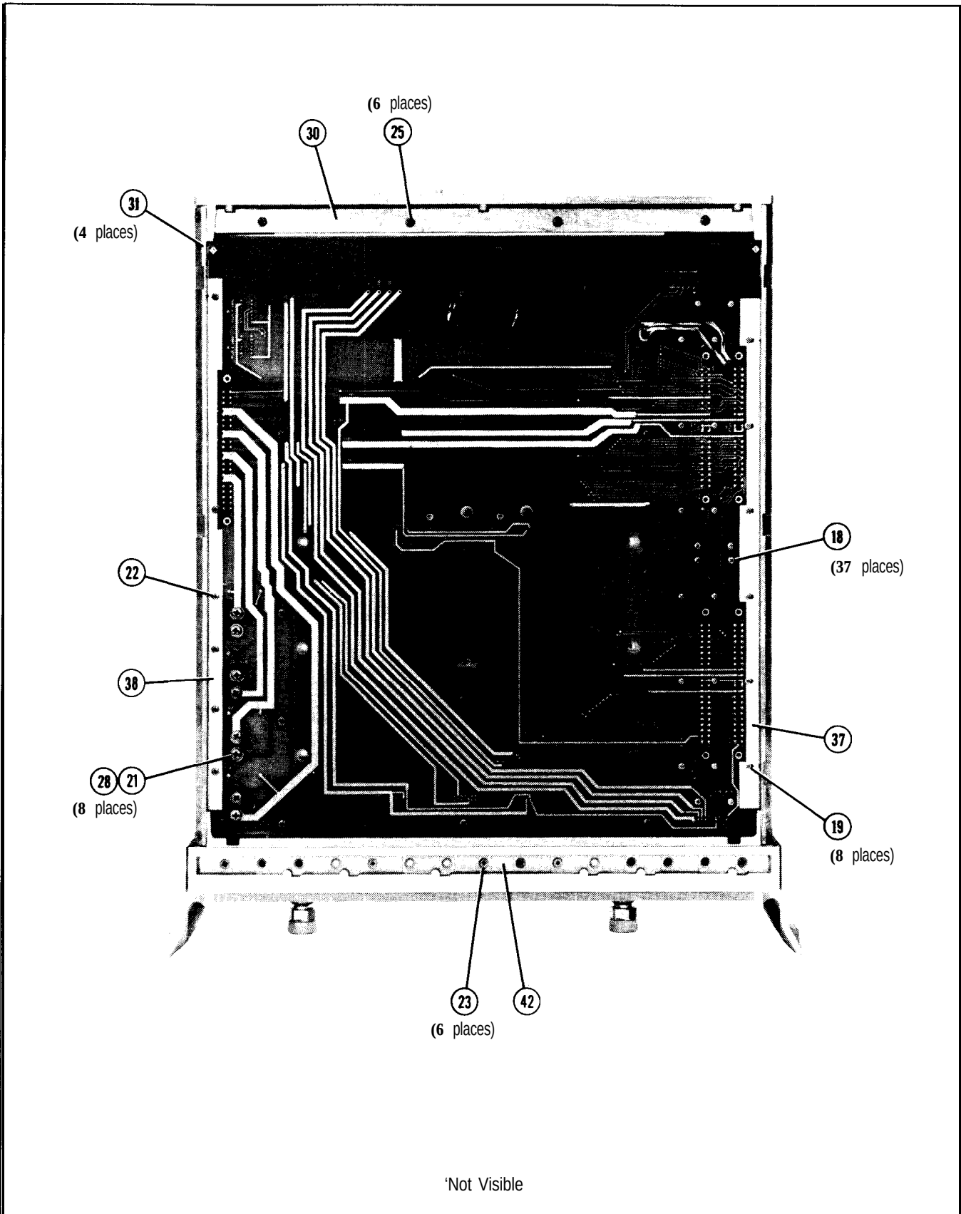
Figure 6-10. HP 8512A Miscellaneous Mechanical, Chassis, and Electrical Parts (3 of 5)
